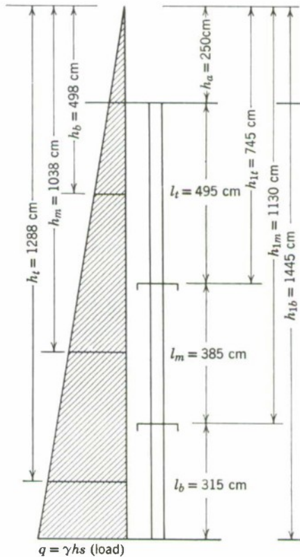
Figure 6.3 Specification of Design Parameters
