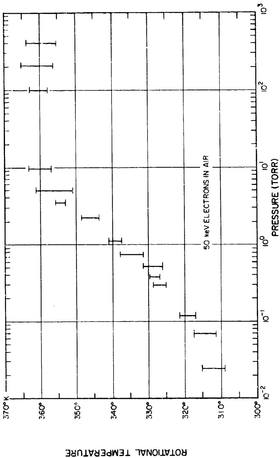
ROTATIONAL TEMPERATURE OF N_2^+ (3914 Å)
