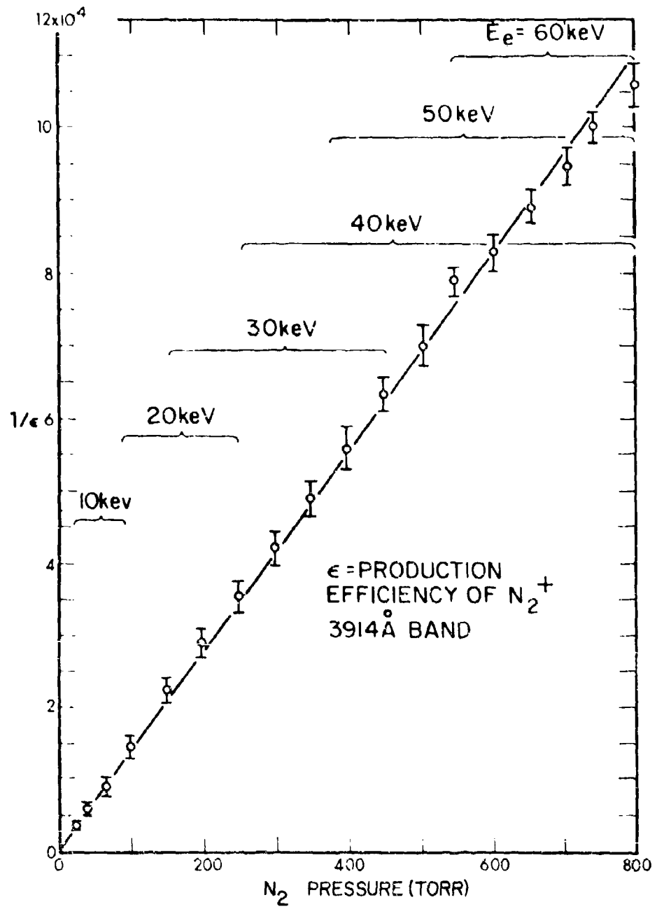
Figure 16 Production Efficiency of N_2^+ (3914 Å) Emission by Electrons
