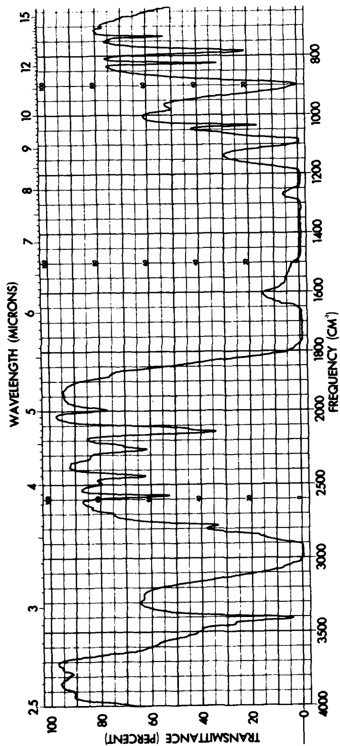
Figure 20. Infrared spectrum of \text{Ca}(\text{NO}_3)_2 in acetone (sodium chloride cell)
