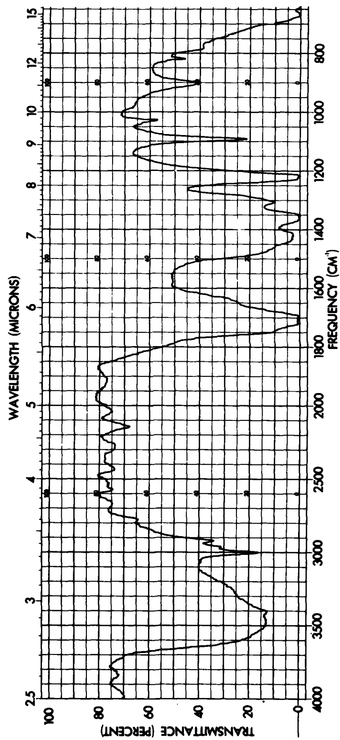
Figure 5. Infrared spectrum of \text{Mn}(\text{NO}_3)_2 \cdot x\text{H}_2\text{O} in acetone (Irtran cell)
