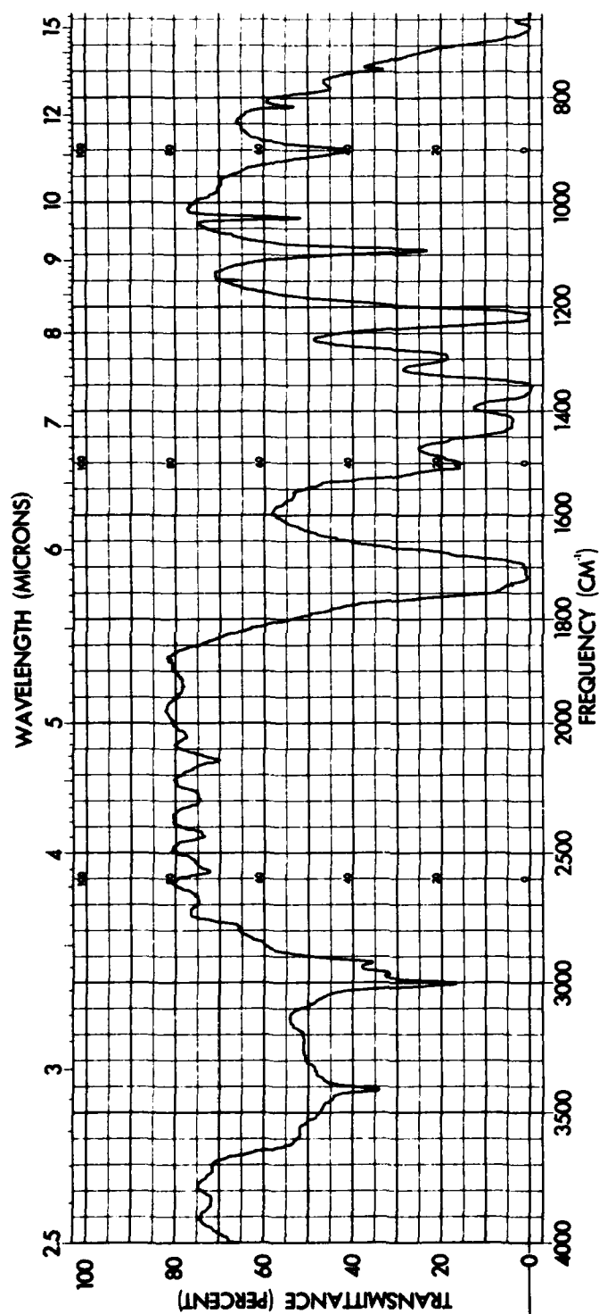
Figure 14. Infrared spectrum of \text{Y}(\text{NO}_3)_2 \cdot 4\text{H}_2\text{O} in acetone (Irtran cell)
