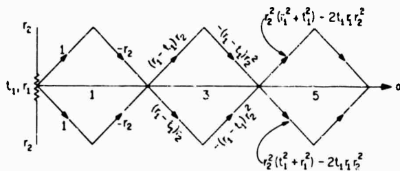
Fig. 4 - General form of traveling waves
