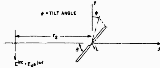
Fig. 2 - Receiving antenna
