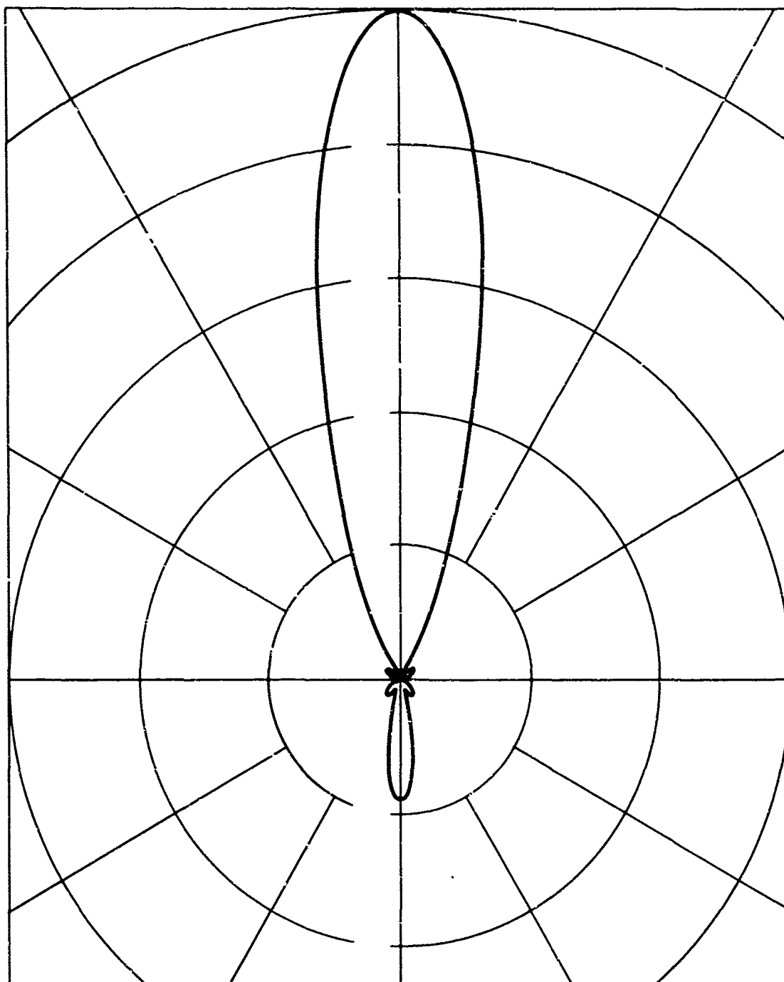
FIG. 7b: The radiation patterns of the triangular lattice arrays with d/\lambda = 0.6 , h/\lambda = 0.4 , E-plane pattern of a 10-element short dipole array.
