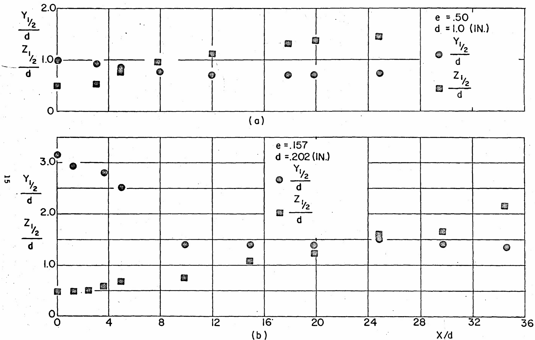
Fig. No. 6 (a) HALF VELOCITY BOUNDARY GROWTH FOR THREE-DIMENSIONAL WAKE, VERNA (1966). (b) HALF VELOCITY BOUNDARY GROWTH FOR THREE-DIMENSIONAL WAKE. PIBAL DATA (1968).
