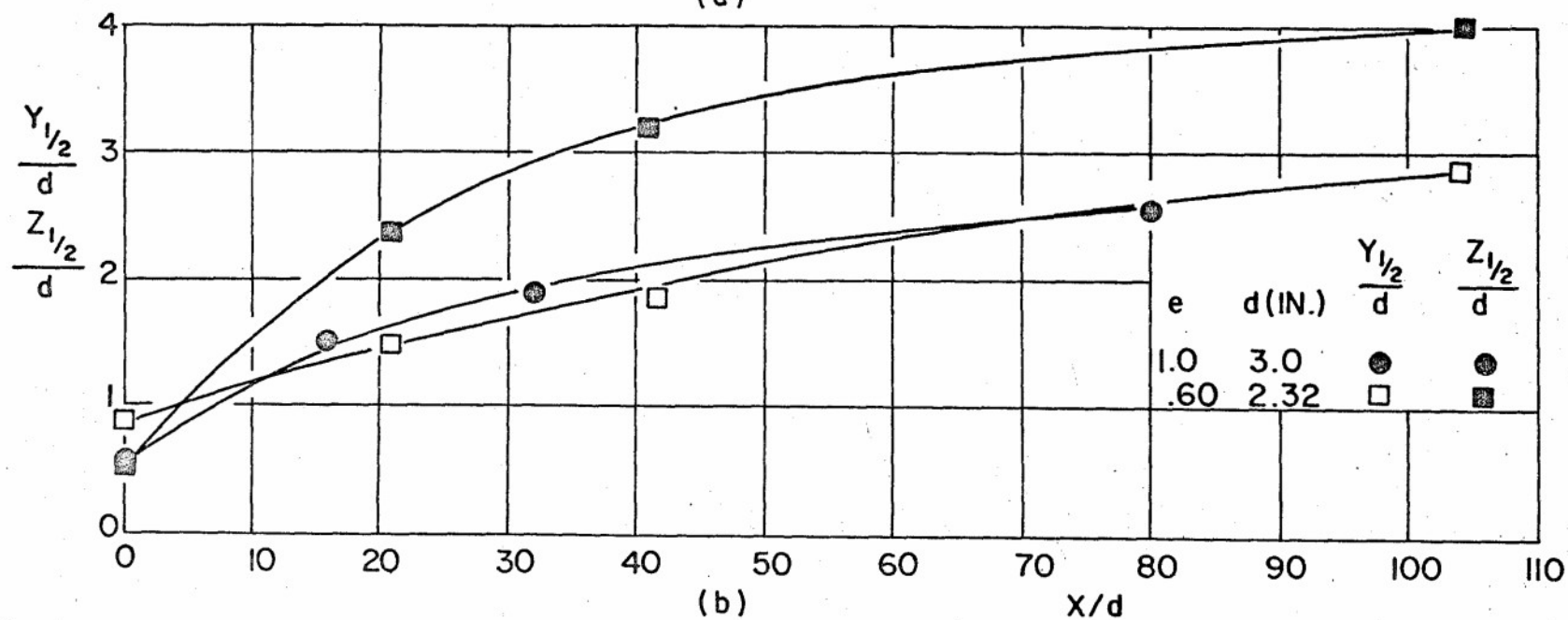
Fig. No. 5 HALF VELOCITY BOUNDARY GROWTH FOR THREE-DIMENSIONAL WAKES. KUO and BALDWIN (1967).
