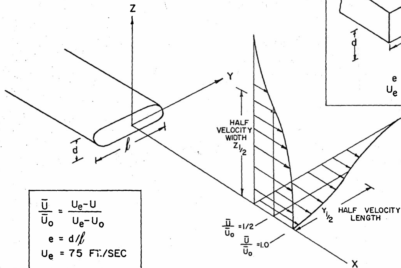
Fig. No. 1c SCHEMATIC REPRESENTATION OF THREE-DIMENSIONAL WAKE FLOW FIELD. SOLID OVAL BODY SUPPORTED UPSTREAM, PIBAL DATA (1968). UPPER RIGHT HAND CORNER, SOLID RECTANGULAR BODY SUPPORTED UPSTREAM, VERNA(1966).
