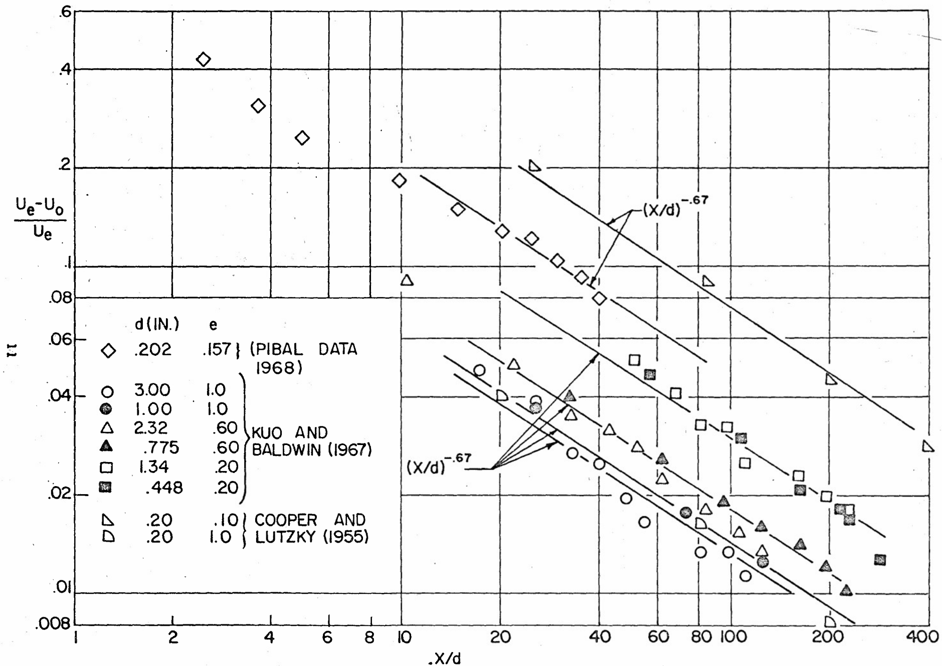
Fig. No. 2 AXIAL VELOCITY DEFECT DECAY OF THREE-DIMENSIONAL WAKE.
