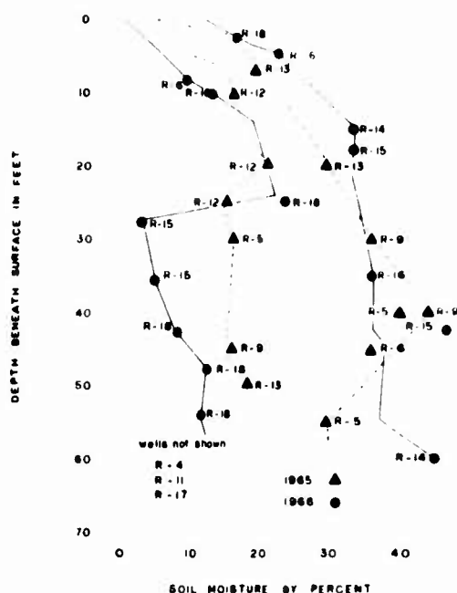
Figure 10. Limits of Soil Moisture Content with Depth for Years 1965 and 1966, Rogers Playa
