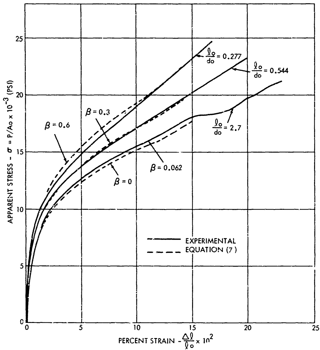
FIG. 12 EFFECTS OF FRICTION ON APPARENT STRESS-STRAIN BEHAVIOR
