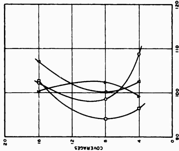
DRY OF OPTIMUM MOISTURE (7.0 %)
