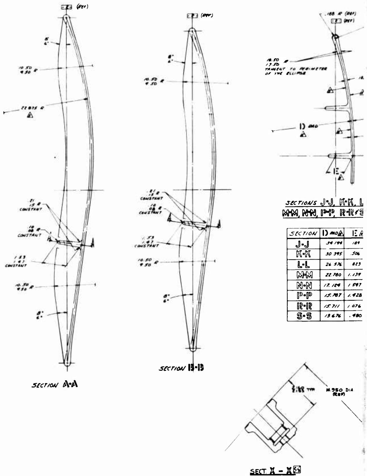
Figure 37. Blade (Sheet 2 of 2).
