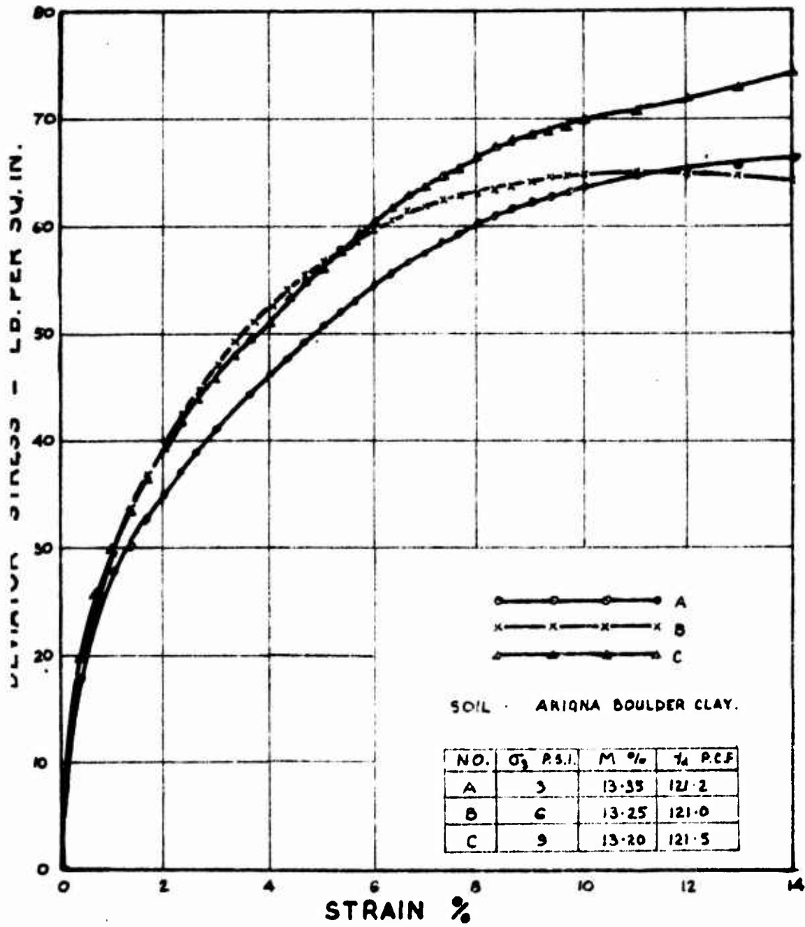
TYPICAL RESULTS OF SLOW UNDRAINED TRIAXIAL TEST
