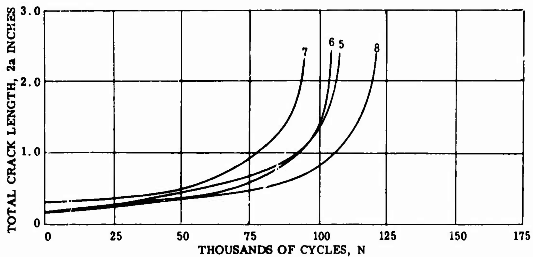
Figure 32. Crack Length versus Cycles to Failure for Ti-13V-11Cr-3Al, Second Stress Level = 13,400 \pm 10,000 psi, Specimens 5, 6, 7, and 8.
