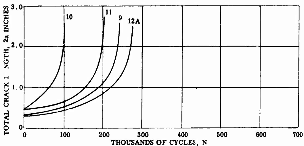
Figure 33. Crack Length versus Cycles to Failure for Ti-13V-11Cr-3Al, Third Stress Level = 20,000 \pm 5,000 psi, Specimens 9, 10, 11, and 12A.
