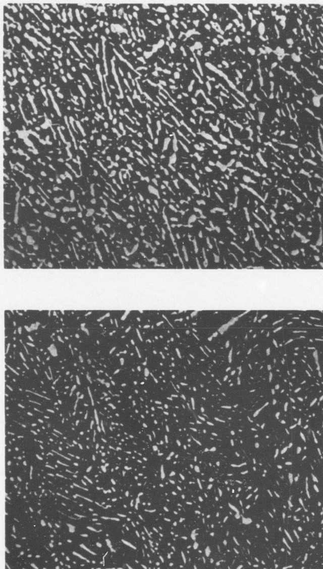
Figure 61. Photomicrograph of Ti-6Al-6V-2Sn Cuff Forging - Hub (Top) and Web (Bottom).
