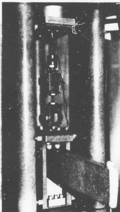
Figure 4. Axial Specimen Installed in SF-1-U Five-to-One Ampli- fier.
