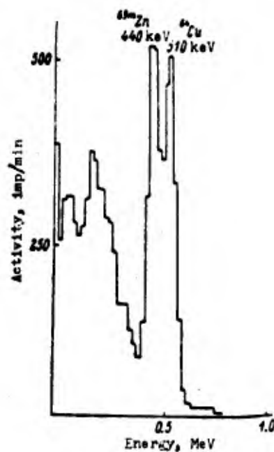
Fig. 4. \gamma -Spectrum of the third group.
