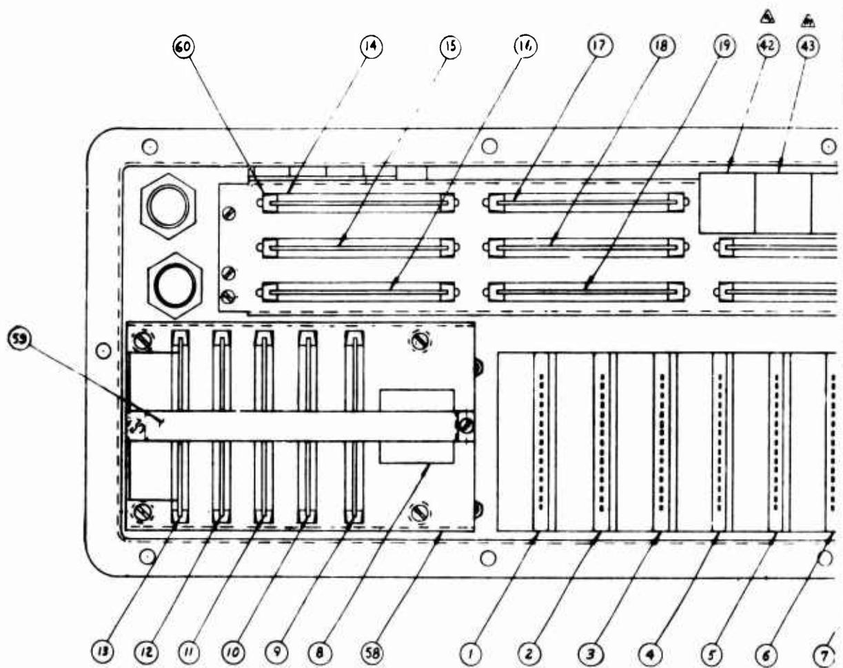
REAR VIEW
