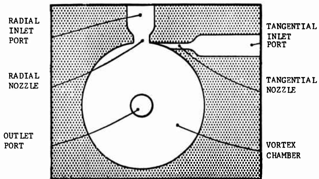
FIGURE 4 - VORTEX AMPLIFIER
