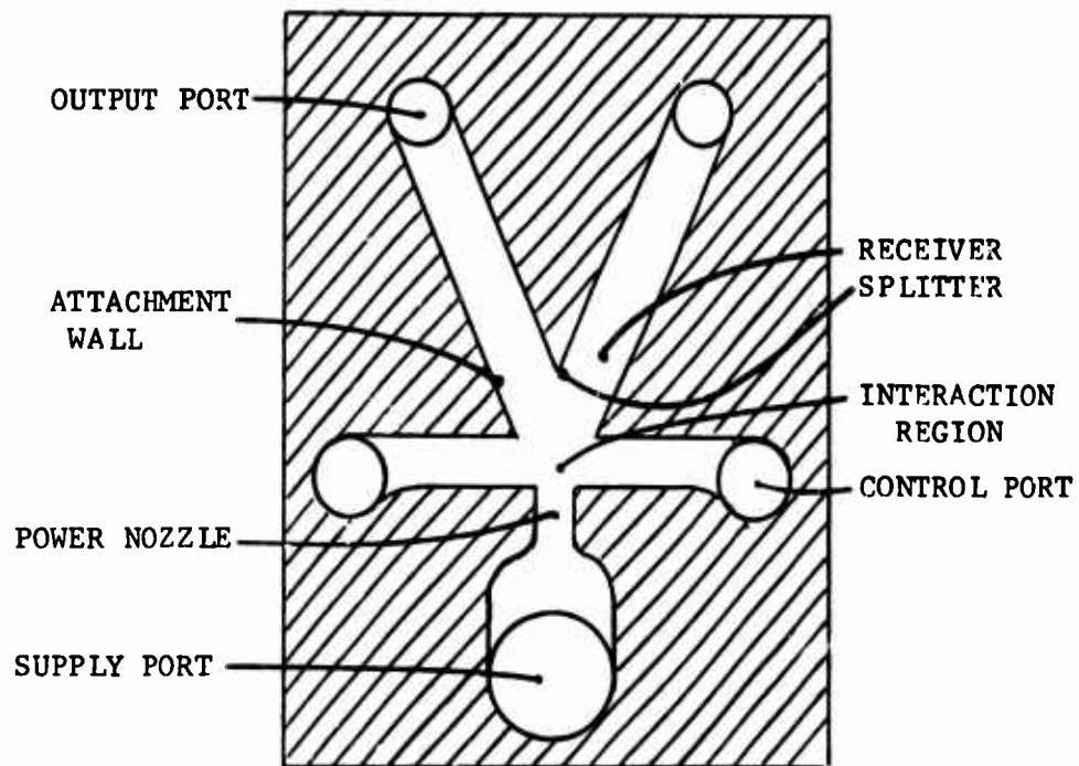
FIGURE 3- WALL-ATTACHMENT AMPLIFIER
