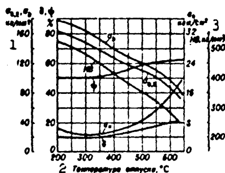
Fig. 10. Influence of tempering temperature on the mechanical characteristics of 40KhNMA steel. 1) kg/mm 2 ; 2) tempering temperature, °C; 3) kg-m/cm 2 .
