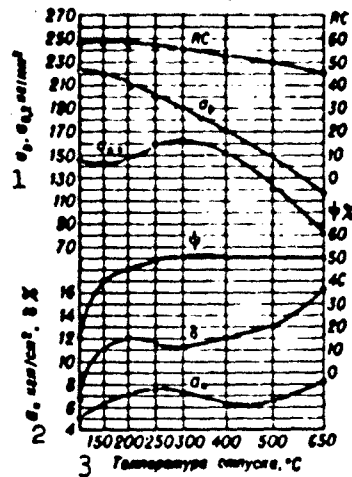
Fig. 2. Influence of tempering temperature on the mechanical characteristics of EI643 steel. 1) kg/mm 2 ; 2) kg-m/cm 2 ; 3) tempering temperature, °C.
