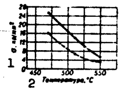
Fig. 2. Long-term strength of 20KhML steel over 100,000 hr (solid line) and creep strength (dash line) of same steel over 100,000 hr at elevated temperatures in the presence of 1% residual deformation. 1) kg/mm 2 ; 2) temperature, °C.
