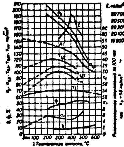
Fig. 1. Physicommechanical characteristics of 50KhFA steel as a function of tempering temperature. 1) kg/mm 2 ; 2) tempering temperature, °C; 3) stress relaxed over 100 hr at \tau_0 = 56 kg/mm 2 .
