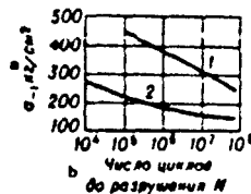
Fig. 10. Fatigue curves for bending in one plane for organic glass ( \sigma_b = 625 \text{ kg/mm}^2 ): 1) Specimen thickness 3.2 mm; 2) specimen thickness 6.4 mm. a) \sigma_{-1} kg/cm^2 ; b) number of cycles to failure, N .
