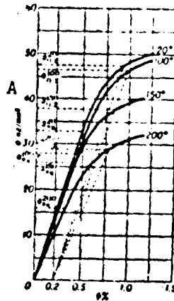
Fig. 4. Compression diagram to yield point at room and elevated temperatures for V95AT alloy (sheet 2 mm thick, \sigma_b = 52 \text{ kg}/\text{mm}^2 , \delta_{10} = 14\% ). A) \text{kg}/\text{mm}^2 . \epsilon\% = pts.
