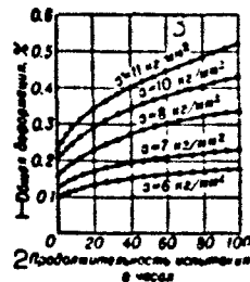
Fig. 7. Creep curves for D16T alloy at 200° (sheet 2 mm thick). 1) Total deformation, %; 2) test time, hr; 3) kg/mm 2 .
