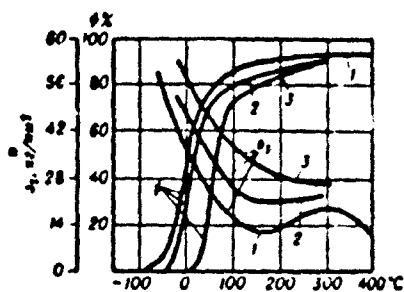
Fig. 12. Effect of deformation rate ( v ) on critical brittleness temperature of annealed molybdenum; 1) v = 2.8 \cdot 10^{-4} \text{ sec}^{-1} ; 2) v = 4.10^{-3} \text{ sec}^{-1} ; 3) v = 0.17 \text{ sec}^{-1} . a) \text{kg}/\text{mm}^2 .
