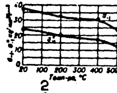
Fig. 6. Fatigue strength of the 2Kh13 steel (quench from 1050° in oil, temper at 700°). 1) σ -1 , σ n-1 , kg/mm 2 ; 2) temperature, °C.
