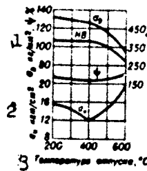
Fig. 4. Influence of tempering temperature on the mechanical characteristics of 18KhNVA steel. 1) kg/mm 2 ; 2) kg-m/cm 2 ; 3) tempering temperature, °C.
