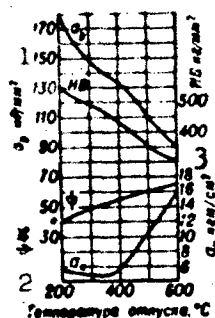
Fig. 1. Influence of tempering temperature on the mechanical characteristics of 38KhA steel (quenched from 850° in oil). 1) kg/mm 2 ; 2) tempering temperature, °C; 3) kg-m/cm 2 .
