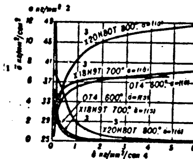
Fig. 3. Variation of breaking stress \sigma with loading rate \dot{\delta} , and loading rate rise \ddot{\delta} for the titanium alloy OT4, for Kh18N9T steel, for the nickel alloy Kh20N8OT (El435); \dot{\delta} (kg/mm 2 /sec) is the first derivative of the stress with respect to loading rate and characterizes the loading rate; \ddot{\delta} (kg/mm 2 /sec 2 ) is the second derivative of the stress as a function of loading rate and characterizes the increase of the loading rate. 1) kg/mm 2 /sec 2 ; 2) kg/mm 2 ; 3) Kh - N - T; 4) kg/mm 2 /sec.
