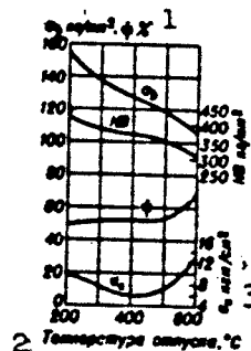
Fig. 5. Influence of tempering temperature on the mechanical characteristics of 25KhNVA steel. 1) kg/mm 2 ; 2) tempering temperature, °C; 3) kg-m/cm 3 .
