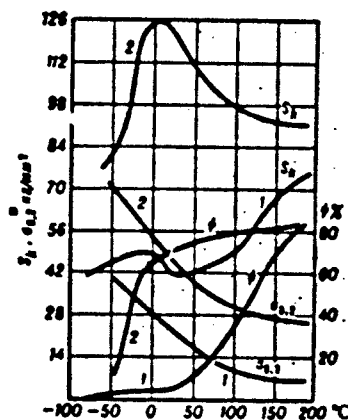
Fig. 7. Effect of grain size on cold shortness of molybdenum produced by powder metallurgy method: 1) Grain No. 3-4; 2) grain No. 7-8. a) \text{kg}/\text{mm}^2 .
