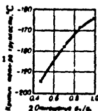
Fig. 13. Effect of biaxiality during plane tension on critical brittleness temperature of SAE1045 steel. 1) Critical brittleness temperature, ^{\circ}\text{C} ; 2) ratio.
