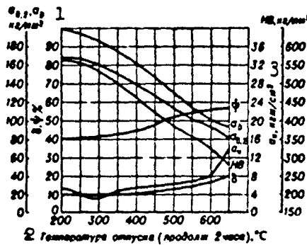
Fig. 6. Influence of tempering temperature on the mechanical characteristics of 38KhS steel. 1) kg/mm 2 ; 2) tempering temperature (tempering time - 2 hr), °C; 3) kg-m/cm 2 .
