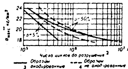
Fig. 13. Endurance curves for anodized and nonanodized specimens of the V91 alloy corresponding to fracture probability P = 50\% and P = 5\% . 1) \sigma_{max} , \text{kg/mm}^2 ; 2) number of cycles to failure; 3) anodized specimens; 4) nonanodized specimens.
