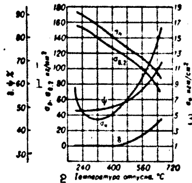
Fig. 3. Influence of tempering temperature on the mechanical characteristics of 33KhN3MA steel. 1) kg/mm 2 ; 2) tempering temperature, °C; 3) kg-m/cm 2 .
