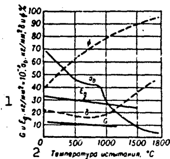
Fig. 2. Effect of test temperature on mechanical properties of wrought molybdenum produced by the arc method. 1) G and E_g , \text{kg/mm}^2 \times 10^{-3} , \sigma_b , \text{kg/mm}^2 , \delta and \psi , %; 2) test temperature, ^{\circ}\text{C} .
