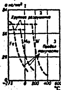
Fig. 1. Variation of yield strength and brittle fracture strength for certain metals with reduction of temperature.
