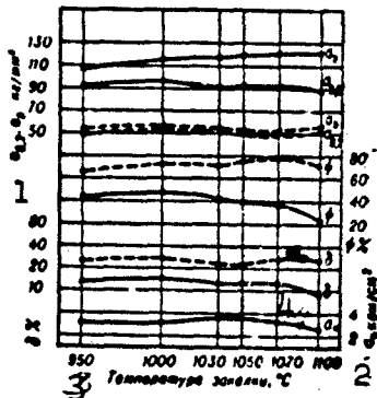
Fig. 3. Effect of quench temperature on mechanical properties of VNS-6 steel (tempered at 650°): -----) air quench; —) oil quench. 1) \sigma_{0.2} , \sigma_b , kg/mm 2 ; 2) a_n , kgm/cm 2 ; 3) quench temperature, °C; 4) a_n .
