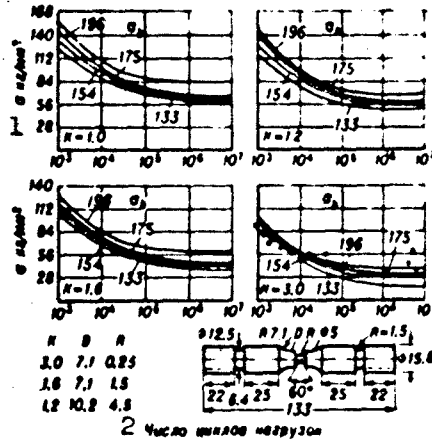
Fig. 4. Strength of 40KhNMA steel specimens under repeated loads as a function of tensile strength and stress concentration (K). (Symmetric extension-compression cycle). 1) kg/mm 2 ; 2) number of loading cycles.
