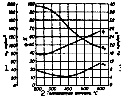
Fig. 2. Influence of tempering temperature on the mechanical characteristics of 37KhN3A steel. 1) \text{kg}/\text{mm}^2 ; 2) tempering temperature, ^{\circ}\text{C} ; 3) \text{kg}\cdot\text{m}/\text{cm}^2 .
