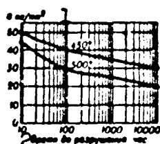
Fig. 4. Stress rupture strength of 2Kh13 steel at temperatures of 450 and 500° (air quench from 1020°, temper at 700°). 1) \sigma , kg/mm 2 ; 2) time of failure, hours.
