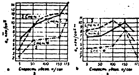
Fig. 10. Variation of impact strength as a function of the impact velocity: a) Steel after tempering at 200°; b) steel after tempering at 600°; 1) kgm/cm 2 ; 2) steel; 3) impact velocity, m/sec.
