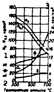
Fig. 3. Mechanical characteristics of 40KhNVA steel as a function of tempering temperature (quenching from 850° in oil). 1) kg/mm 2 ; 2) tempering temperature, °C; 3) kg-m/cm 2 .
