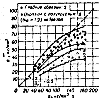
Fig. 1. Relation between endurance limits and strength limits for steel (from data of various authors); 1) kg/mm 2 ; 2) smooth specimens; 3) specimens with semicircular ( \alpha_\sigma = 1.9 ) notch.
