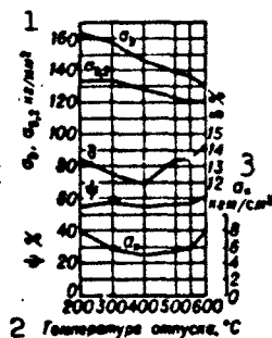
Fig. 2. Mechanical characteristics of 23Kh2NVFA (EI659) steel after quenching and tempering at various temperatures. 1) kg/mm 2 ; 2) tempering temperature, °C; 3) kg-m/cm 2 .
