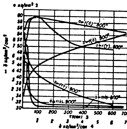
Fig. 4. Variation of breaking stress with loading time \tau (sec) and loading rate \dot{\delta} (kg/mm 2 /sec), and increase of loading rate \ddot{\delta} (kg/mm 2 /sec 2 ) for alloy EI868 at temperatures of 800 and 900°. 1) kg/mm 2 /sec 2 ; 2) kg/mm 2 ; 3) (sec); 4) kg/mm 2 /sec.
