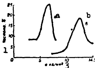
Fig. 3. Frequency curves of the strength of friction cermets: a) Tensile test; b) bending test. 1) Frequency, in %; 2) \sigma , \text{kg}/\text{mm}^2 .
