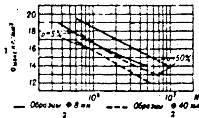
Fig. 8. Fatigue curves of specimens of various diameters made from the AV-T1 alloy with failure probability P = 50\% and P = 5\% . 1) \sigma_{max} , kg/mm^2 ; 2) \phi 8-mm-diam specimens.
