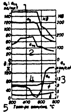
Fig. 2. Variation of mechanical properties of 1Kh13 steel with tempering temperature (oil quench from 980°). 1) \sigma_b , \sigma_{pts} , kg/mm 2 ; 3) a_n , kgm/cm 2 ; 4) a_n ; 5) tempering temperature, °C.
