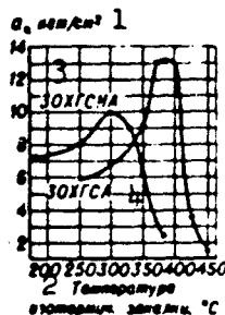
Fig. 3. Influence of isothermal quenching temperature on the impact strength of 30KhGSNA and 30KhGSA steels. 1) kg-m/cm 2 ; 2) isothermal quenching temperature, °C; 3) 30KhGSNA; 4) 30KhGSA.
