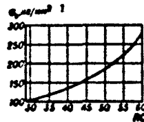
Fig. 2. Ultimate tensile strength of steel as a function of hardness. 1) kg/mm 2 .
