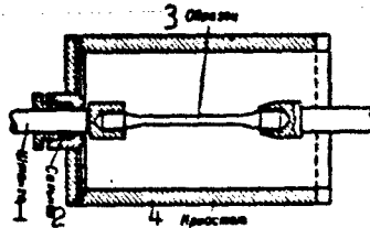
Fig. 3. Cryostat for the tensile test of smooth notched specimens at low temperatures. 1) Rod; 2) stuffing box; 3) specimen; 4) cryostat.
