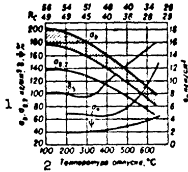
Fig. 4. Influence of tempering temperature on the mechanical characteristics of 30KhGSA steel. 1) kg/mm 2 ; 2) tempering temperature, °C; 3) kg-m/cm 2 .
