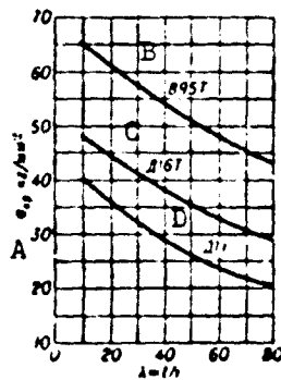
Fig. 5. Curves of longitudinal stability for P-section profiles, 35 x 35 x 4-mm section, made from alloys V95T, D16T and D1T; supported at faces. A) \sigma_{kr} , \text{kg}/\text{mm}^2 ; B) V95T; C) D16T; D) D1T.
