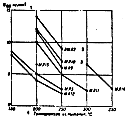
Fig. 6. Stress-to-rupture limits of cast magnesium alloys (after 100 hours). 1) kg/mm 2 ; 2) VML; 3) ML ; 4) test temperature, °C.
