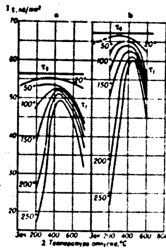
Fig. 2. Relaxation resistance of 50KhFA and 65S2VA steels over 100 hr (initial stress E_0 = 56 \text{ kg/mm}^2 for 50KhFA steel and E_0 = 67 \text{ kg/mm}^2 for 65S2VA steel) as a function of tempering temperature at various relaxation temperatures: a) 50KhFA steel; b) 65S2VA steel. 1) \text{kg/mm}^2 ; 2) tempering temperature, ^\circ\text{C} .
