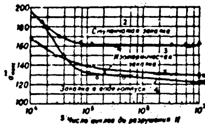
Fig. 2. Endurance of SAE1095 steel (type U9 carbon steel) as a function of the heat treatment regime at hardness RC 53 \sigma_{max} in pounds per dm 2 ). 1) \sigma_{max} ; 2) stepped quench; 3) isothermal quench; 4) water quench plus temper; 5) number of cycles to failure, N.
