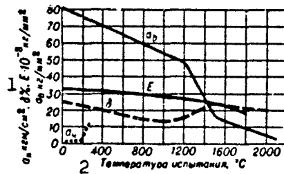
Fig. 2. Effect of temperature on mechanical properties of the VM-2 alloy. 1) \sigma_p , \text{kg/cm}^2 , \delta\% , E \cdot 10^{-3} , \text{kg/mm}^2 ; 2) test temperature, ^{\circ}\text{C} .
