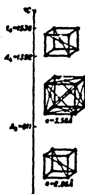
Fig. Scheme of the change of the crystalline structure of iron on heating (the value of the lattice constant is given for 20°).
