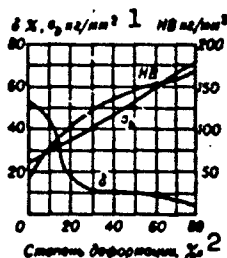
Fig. 1. Variation of mechanical properties of LO90-1 brass with degree of deformation. 1) kg/mm 2 ; 2) degree of deformation.
