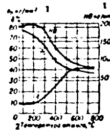
Fig. 2. Variation of mechanical properties of LMts58-2 brass as a function of annealing temperature. 1) \text{kg/mm}^2 ; 2) annealing temperature, °C.
