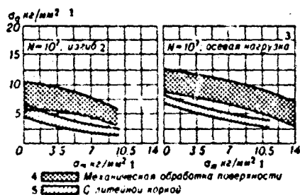
Fig. 7. Influence of average cycle stress on amplitude of safe stresses in Mg-Al-Zn alloys. 1) kg/mm 2 ; 2) bending; 3) axial load; 4) surface machining; 5) with casting skin.
