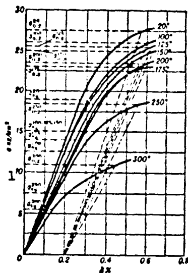
Fig. 4. Graphs showing extension of D16AT alloy to yield point at room and elevated temperatures (sheet 2 mm thick with minimal TU properties). 1) \sigma , kg/mm 2 .
