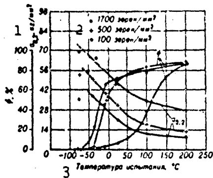
Fig. 1. Effect of grain size on molybdenum plasticity.
