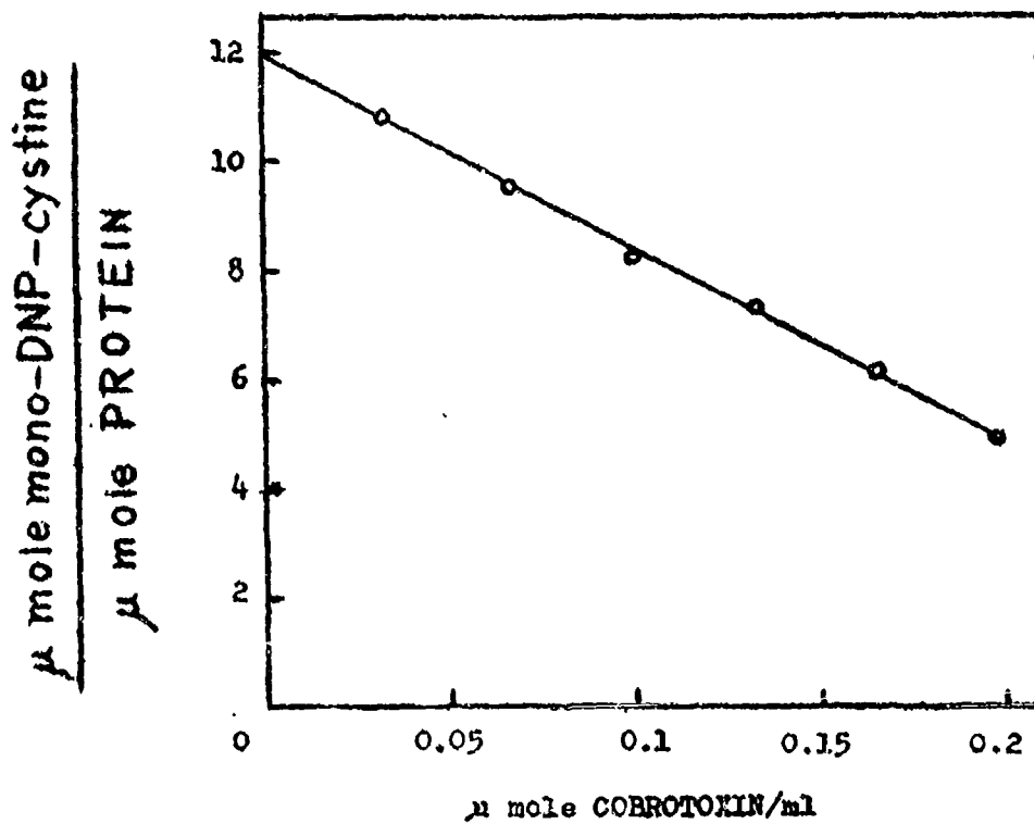
Fig. 1. Equilibrium values for the formation of mono-DNP-cystine in 9.6 N HCl at 39° as a function of cobrotoxin concentration.
