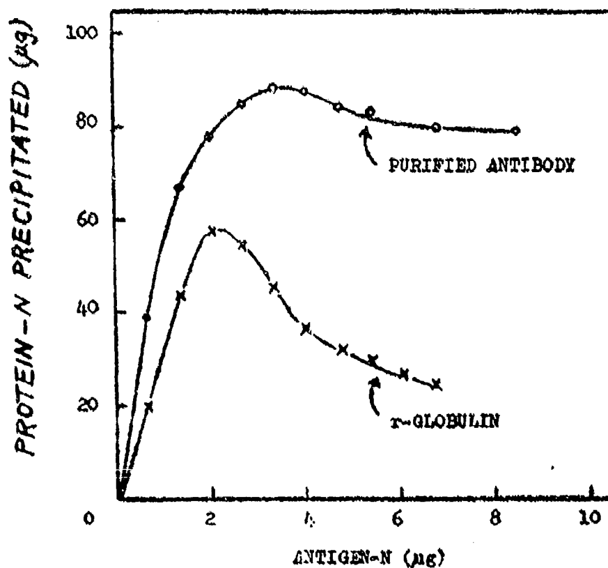
Fig. 9. Precipitin reactions of fluorescent cobrotoxin with r-globulin fraction from rabbit anti-cobrotoxin sera and of cobrotoxin with the purified antibody. r-Globulin-N (848 µg) and the purified antibody-N (84.5 µg) were used. As indicated in the text, the r-globulin fraction contained 6.48 % antibody and the purified antibody was 100 % precipitable.
