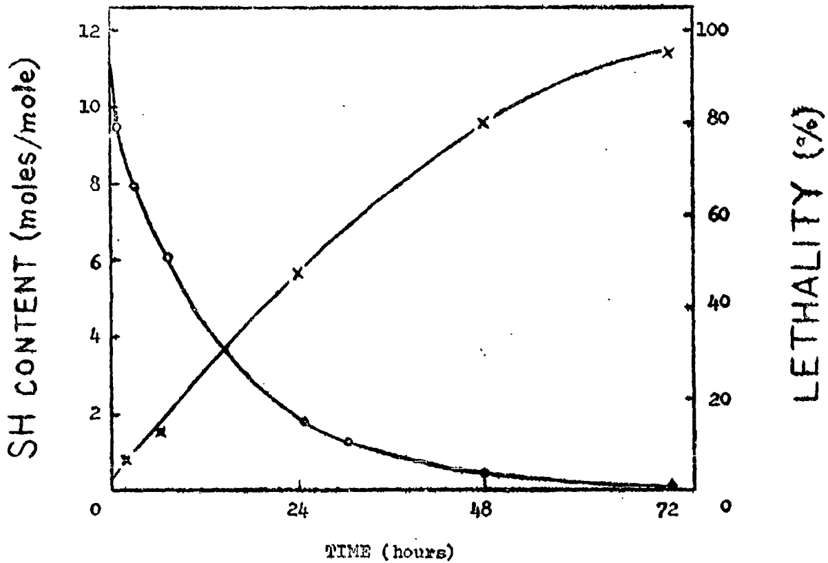
Fig. 2. Restoration of the lethality and disappearance of free sulfhydryl groups on oxidation of reduced cobrotoxin in air. The solution of reduced cobrotoxin (1.8 mg/ml) in 0.05 M phosphate buffer (pH 7.1) containing 0.1 M NaCl was stood at room temperature (25-27°). —●— SH groups; —x— lethality.
