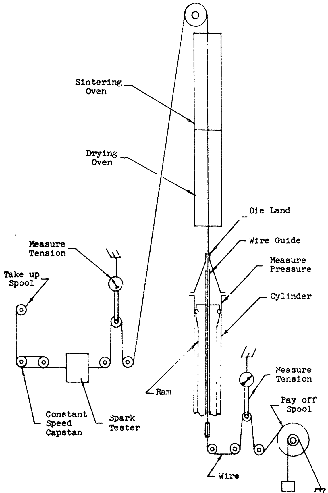
Figure 2 Paste Extrusion Wire Coating Equipment
