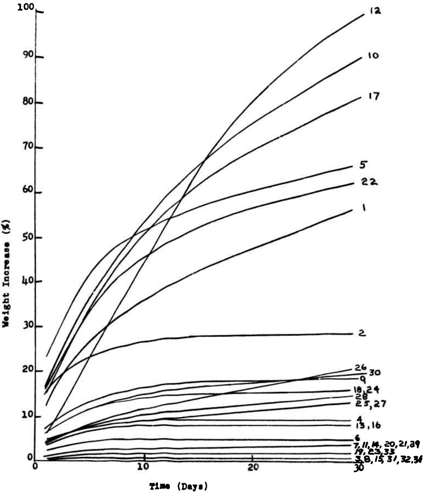
FIGURE 11 WATER ABSORPTION BY FILLERS
