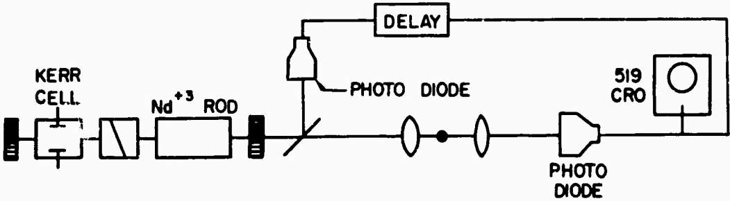
APPARATUS SCHEMATIC
