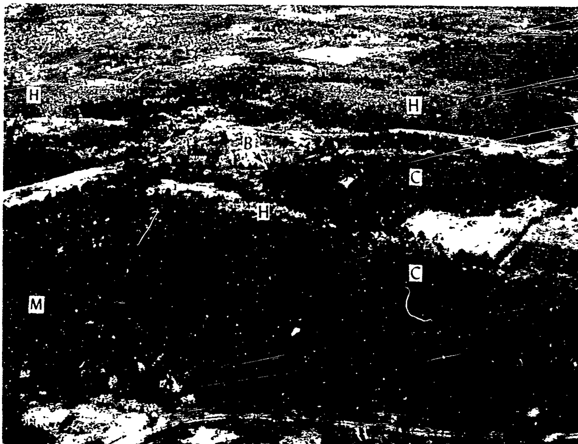
Photo 12. Forest types in north part of NLABS Annex east of headquarters (looking ENE). On the large drumlin (foreground), mixed hardwoods and conifers (M) predominate but forest types range locally from pure conifers (C) to small stands of hardwoods (H). Beyond the hill, a large conifer grove (C) covers most of the lowland on this side of Taylor Brook (B). On far side of patrol road, a representative hardwood forest (H) occupies a broad hill top (252 ft); the forest canopy is fairly open. A second area of hardwoods is also shown at left (H). U.S. Navy photograph, 4 May 1966.
