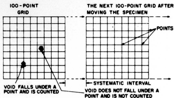
Fig. 8 — Schematic diagram showing the point-count technique for the determination of void content in GRP composites
