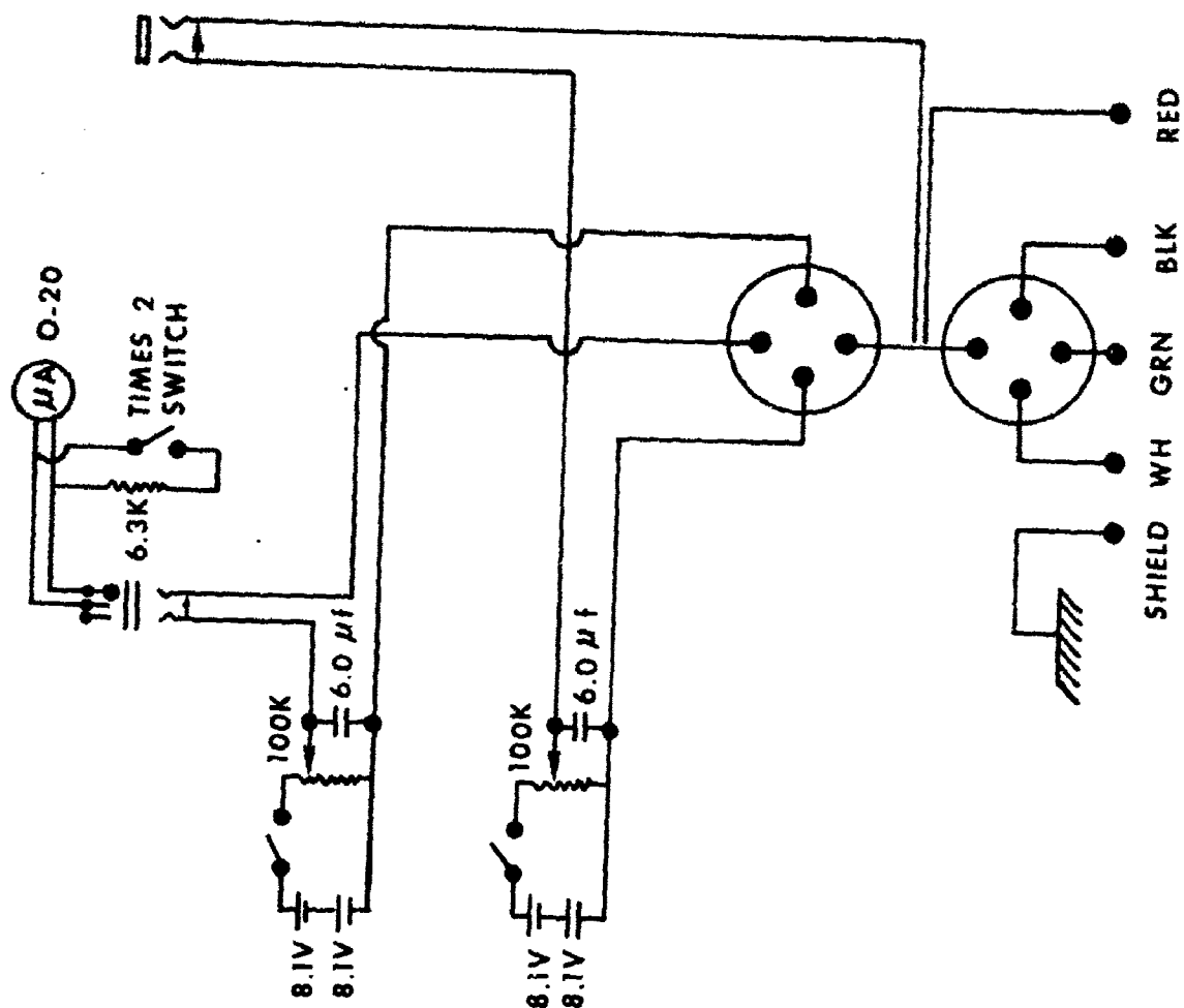
Fig. 5, SCHEMATIC OF DETECTOR BIAS SUPPLY
