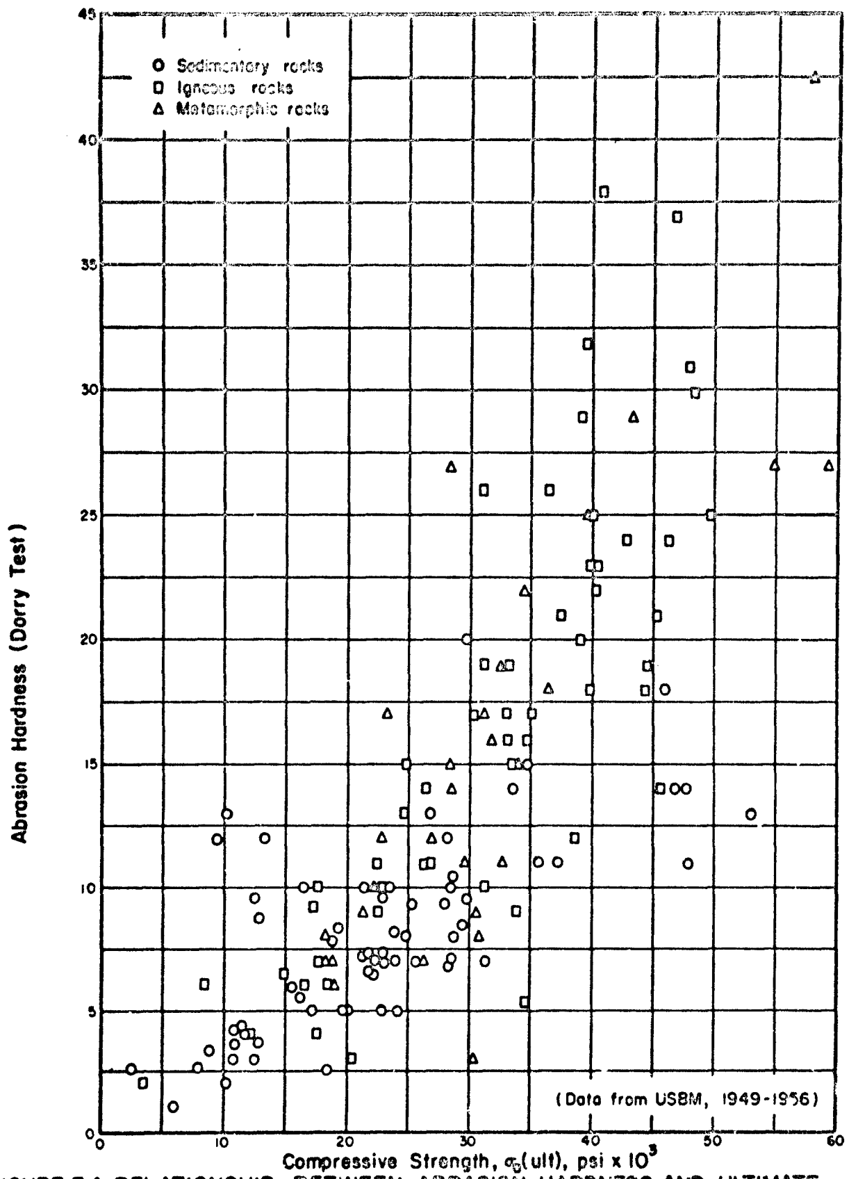
FIGURE 3.4 RELATIONSHIP BETWEEN ABRASION HARDNESS AND ULTIMATE COMPRESSIVE STRENGTH FOR ROCK IN UNIAxIAL COMPRESSION
