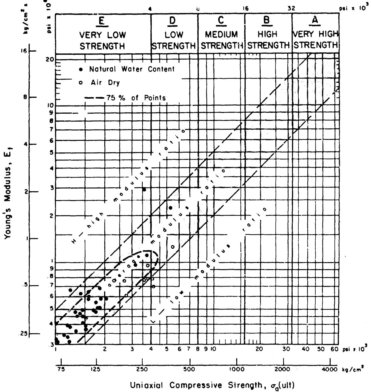
FIGURE 6.12 ENGINEERING CLASSIFICATION FOR INTACT ROCK—POROUS TUFF (44 Specimens, 2 Locations, Various Sources)
