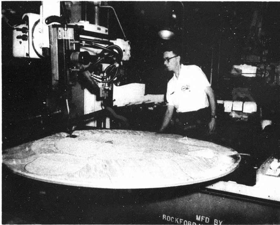
Figure 4 Honeycomb Core - Wing Fan Door
