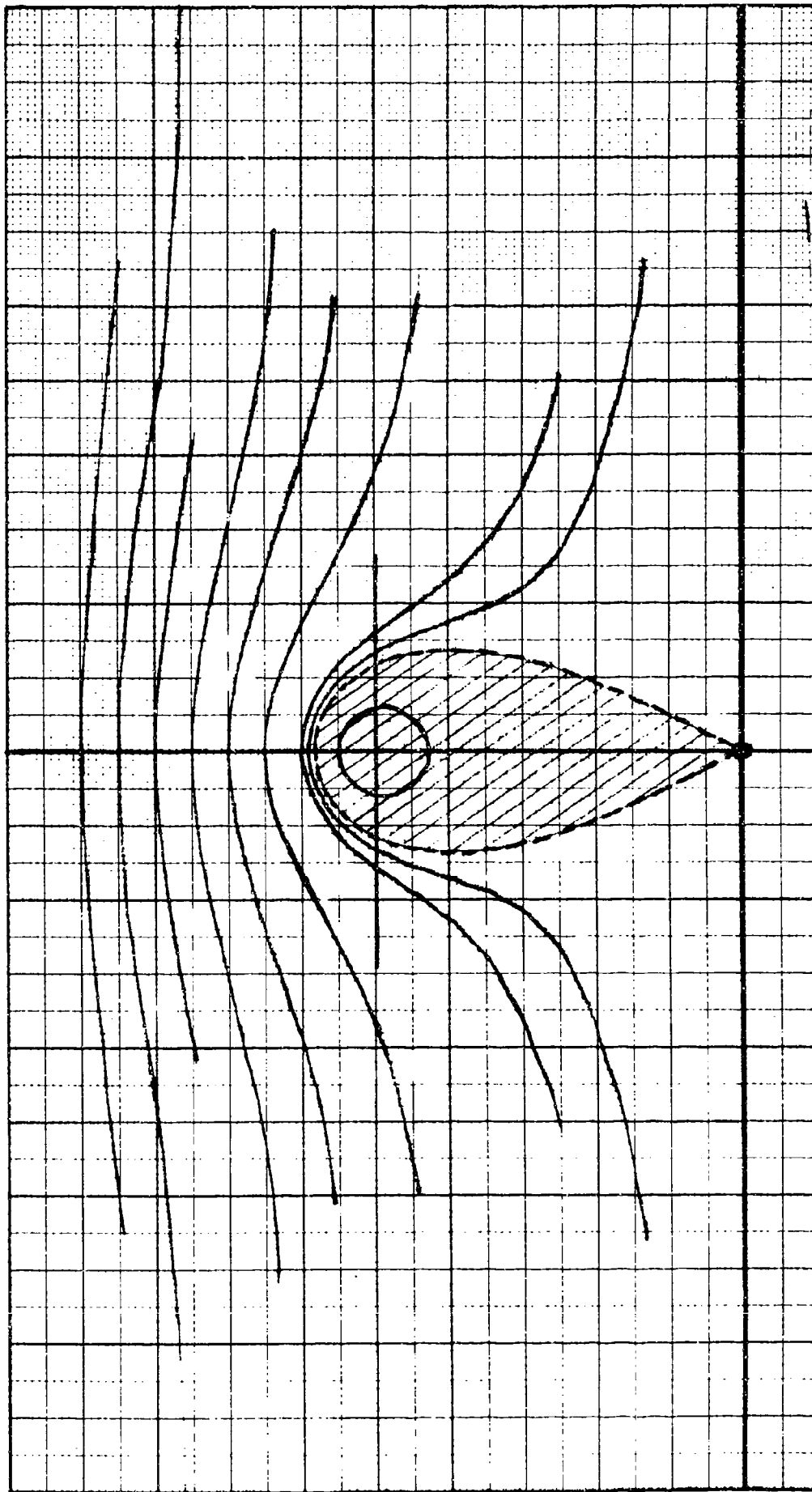
Figure 5. Helmholtz's flow for U = \pi , which is the dividing line between the "blobs" and "true rings". Both stagnation points (the forward and the rear) coincide at the center of the ring.
