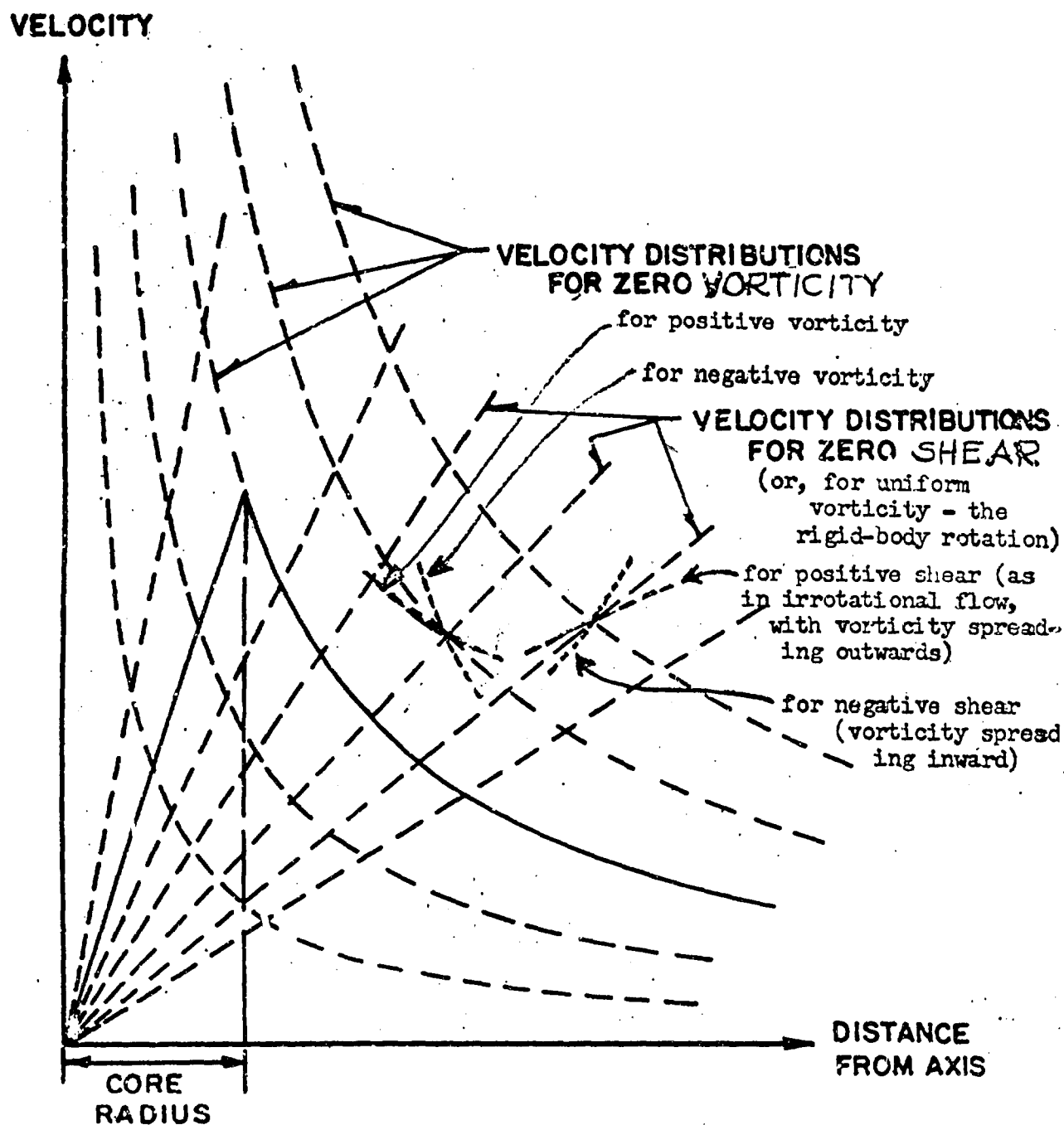
Figure 14. Illustrating the two extreme regimes of flow (zero vorticity and zero shear), and the possible departure of the velocity distribution from these extremes.
