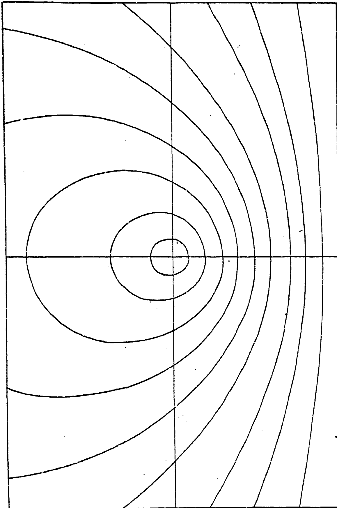
Figure 1b. Streamlines of an idealized vortex ring in a stationary coordinate system at the instant when the ring passes through the plane x = 0 .
