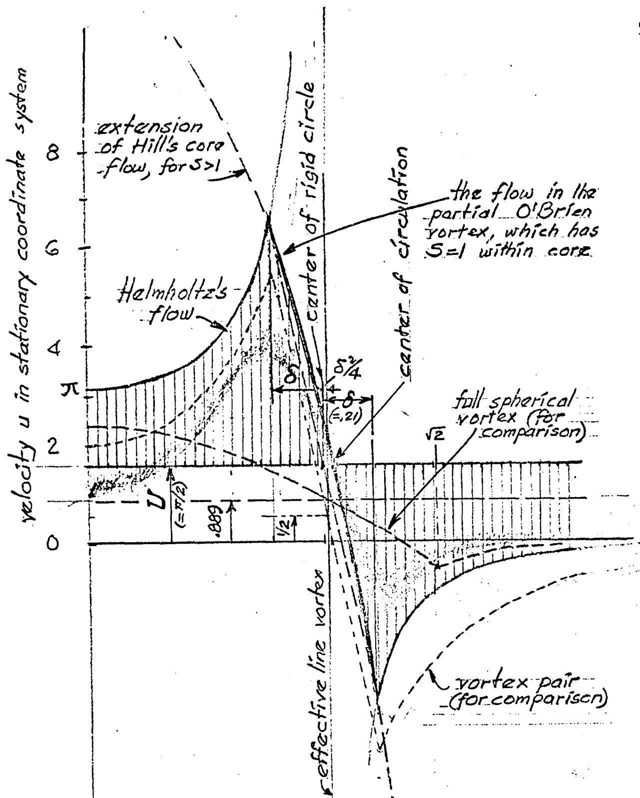
Figure 16. Plots of longitudinal velocity u in the central plane ( x = 0 ). Several unrelated velocity distributions are shown. Solid lines illustrate the distribution in the pattern of Fig. 3 (for U = 1.57 , \delta = .215 ). Dotted lines refer to patterns of Fig. 8 (full spherical vortex) and Fig. 18 (vortex pair). The thick blurred line suggests a possible velocity distribution in an actual "weak true ring", in which the main core is sheathed in a partial return vortex analogous to that of Fig. 15.
