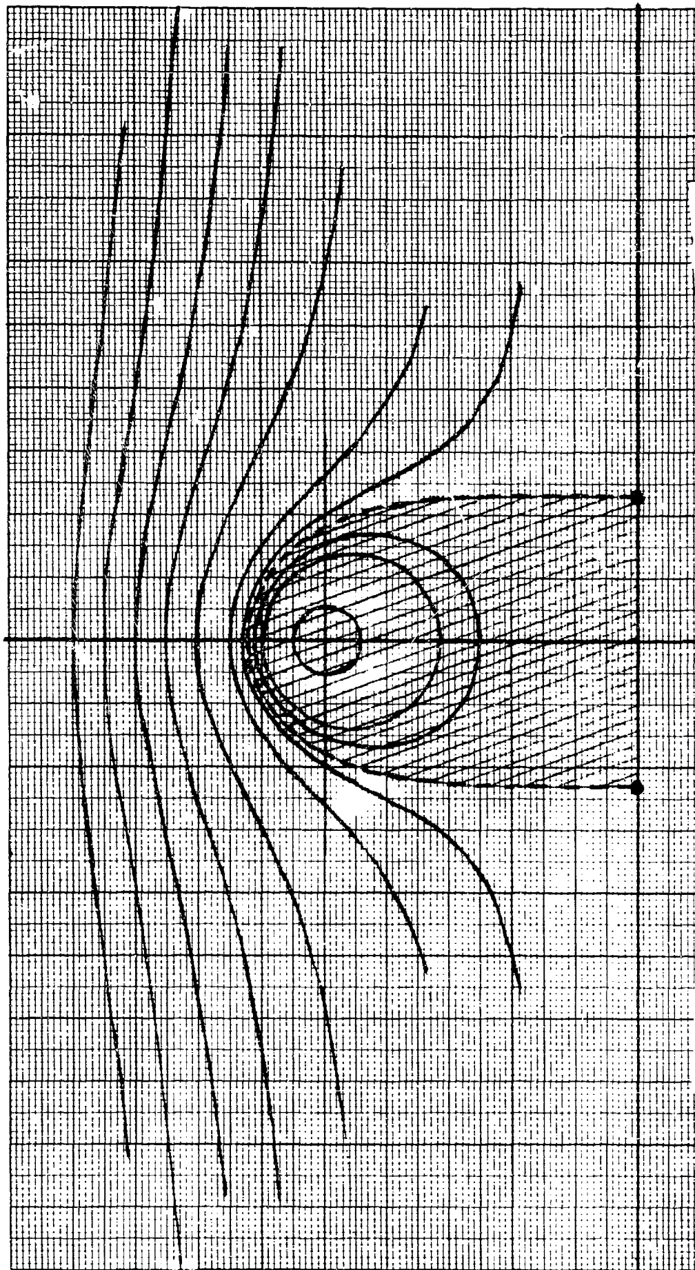
Figure 4. Helmholtz's flow for U = 3\pi/4 . The streamline which moves as the rigid body constitutes a circle so small it cannot very well be shown on this plot.
