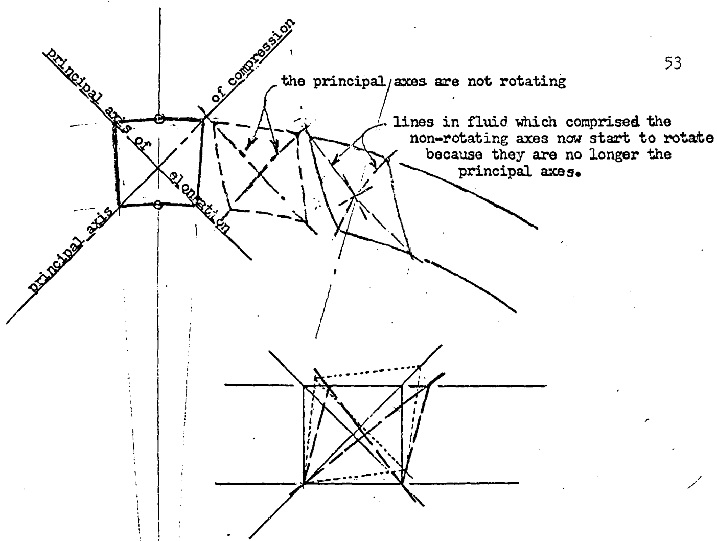
Fig. 13. Illustrating what may appear a paradox: the flow in circles about some center can be irrotational, while the shearing flow in straight parallel lines has rotation. In either case an elementary square distorts into a rhomboid; but the question is whether its diagonals are turning or not.
