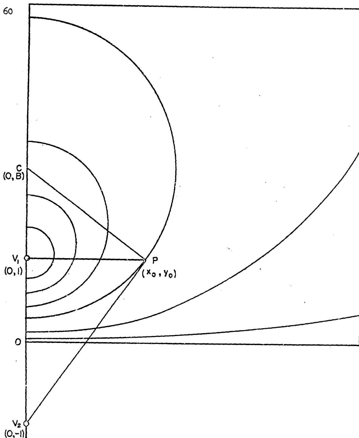
Figure 17. Streamlines of a vortex pair in a stationary coordinate system at the instant when the vortex pair passes through the plane x = 0 .
