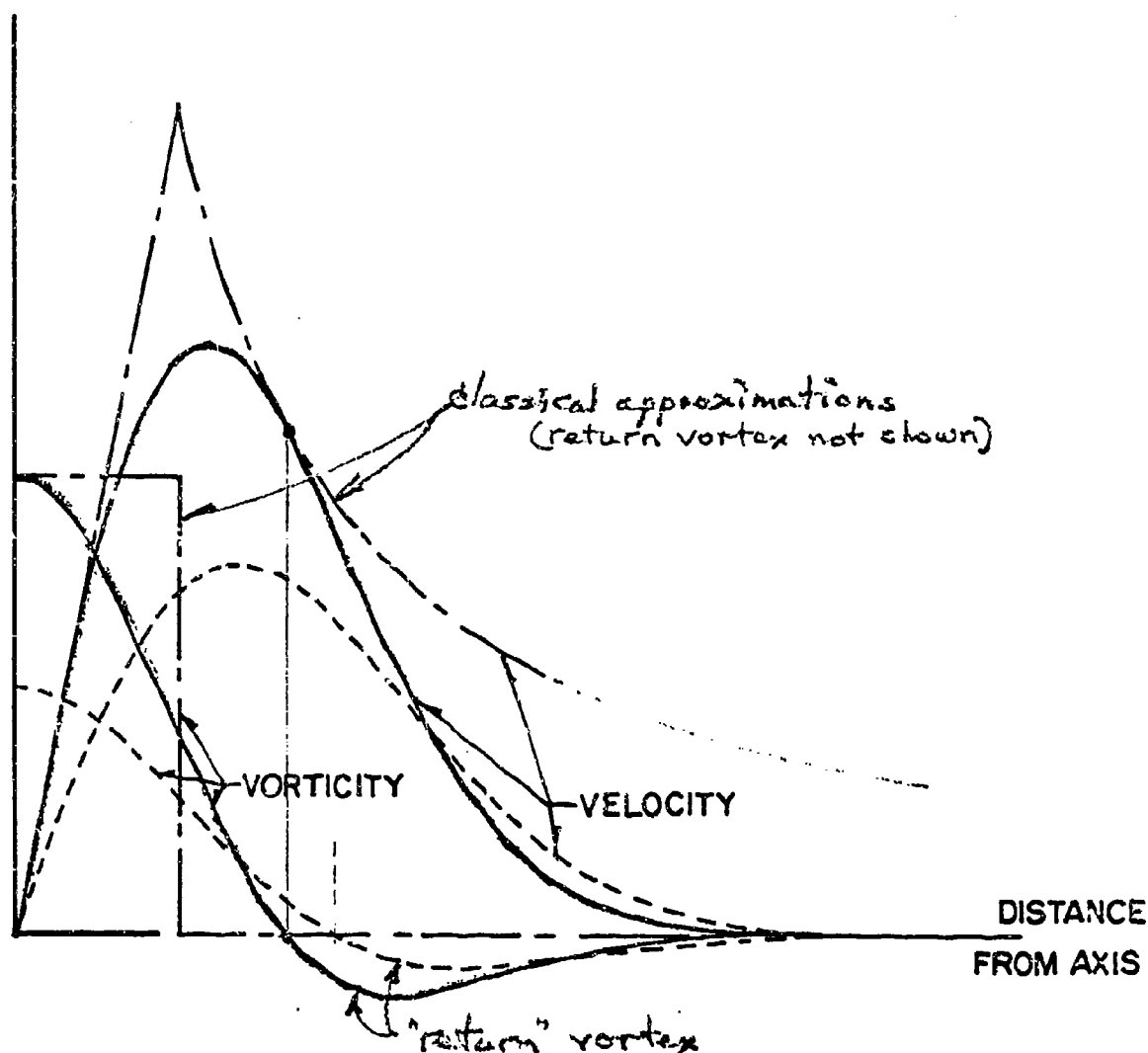
Figure 15. Theoretical structure of a coaxial single vortex. As the vortex spreads, the profiles of velocity and vorticity retain certain proportions; the equations (see reference 4) are
