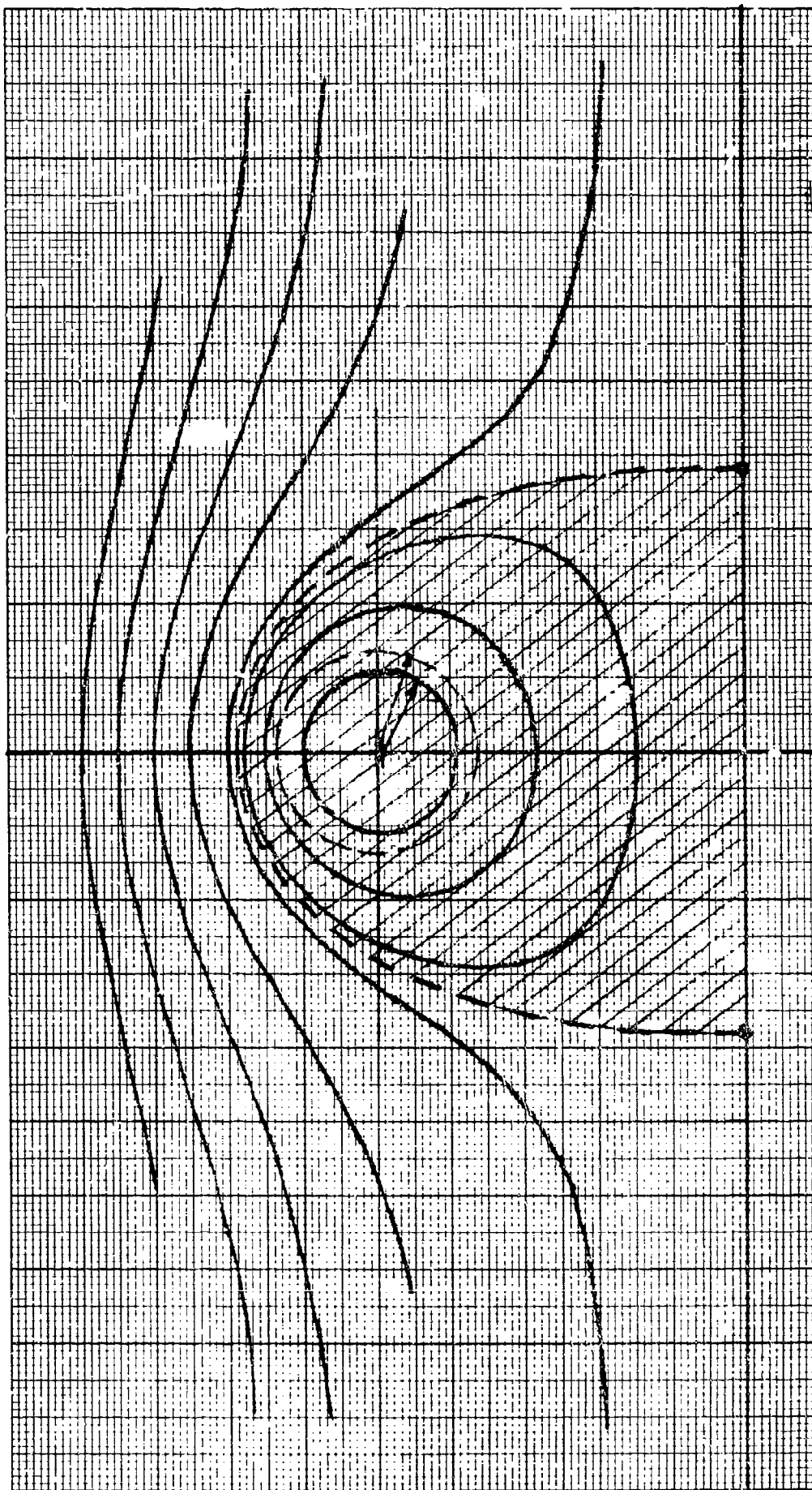
Figure 3. Helmholtz's flow streamlines for U = \pi/2 . The inner streamline shown is practically a circle that moves as a rigid body. The dotted circle represents the core according to Helmholtz-Kelvin-Hicks formula (see the section on "Helmholtz's Vortex Ring: General Description").
