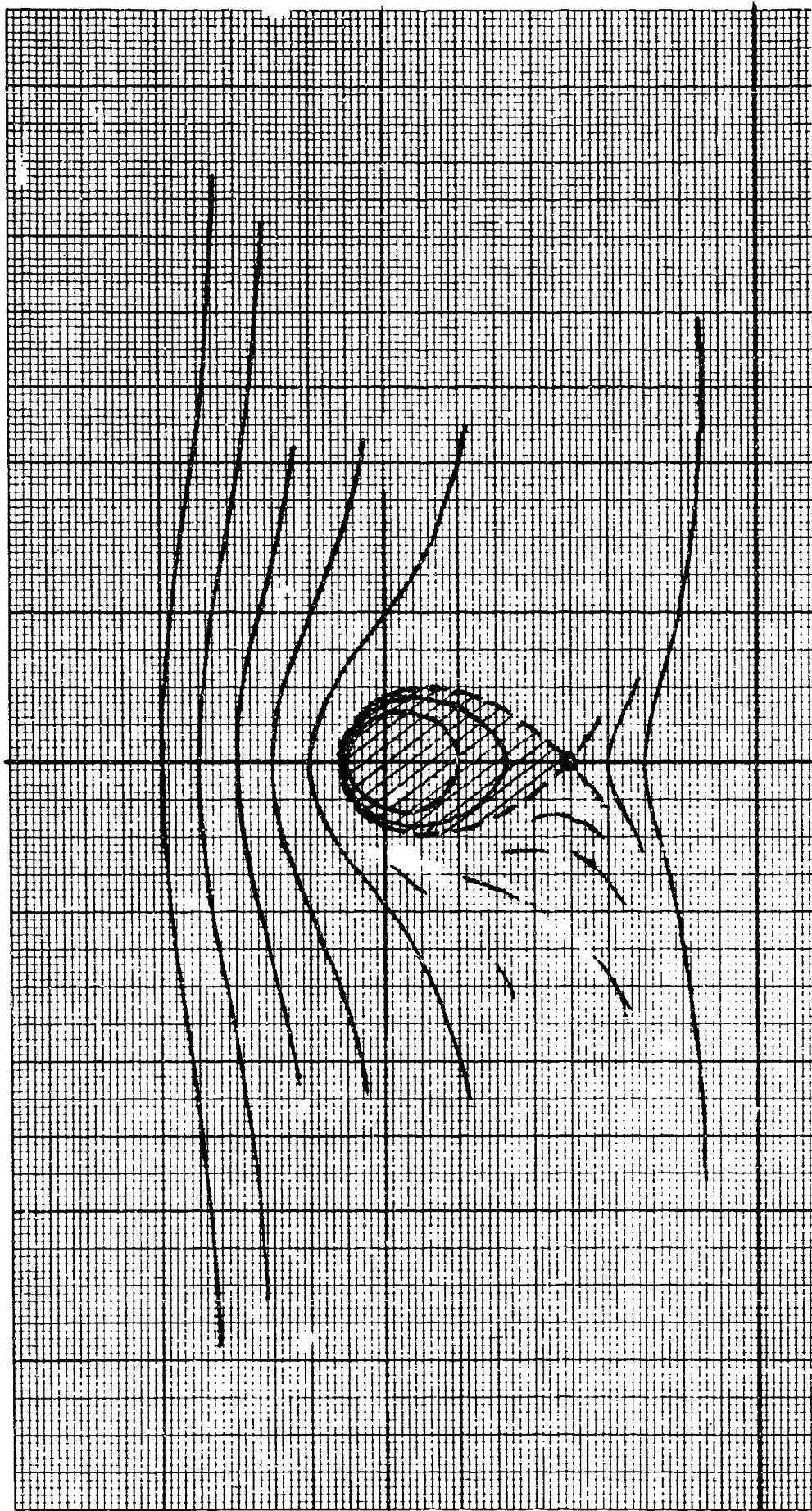
Figure 6. Helmholtz's flow for U = 5\pi/4 , representative of "true" rings. The stagnation points became a ring within the ring. The size of the core is entirely too small to be represented here. It is doubtful that such rings exist.
