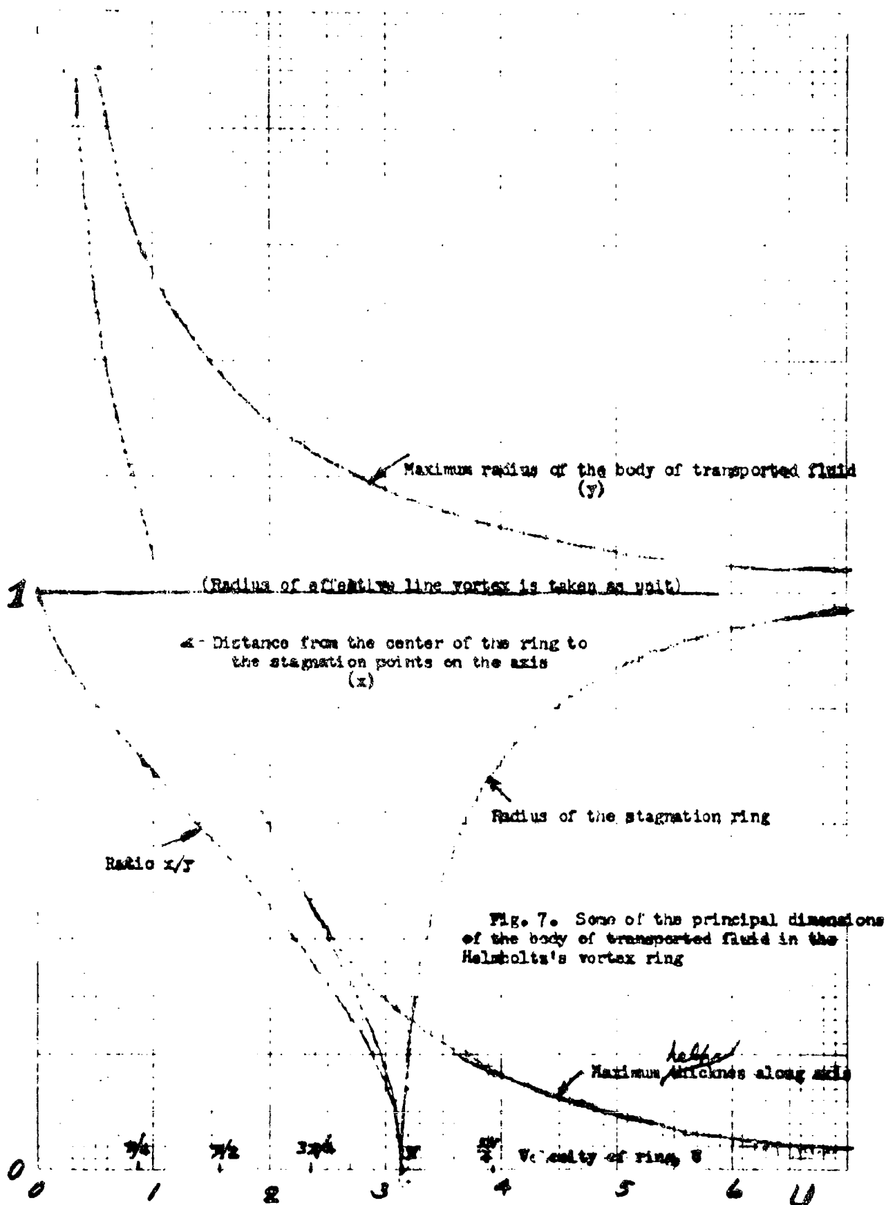
Figure 7. Some of the principal dimensions of the body of transported fluid in the Helmholtz's vortex ring.
