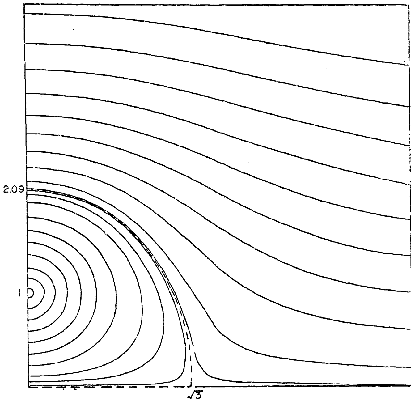
Figure 18. Pathlines in a vortex pair; i.e., streamlines in the coordinate system moving with the pair. The separatrix between the two families of curves defines the fluid moving with the pair. This separatrix has the shape of an oval with semi-axes of 2.09 and \sqrt{3} = 1.73 (Lamb); [1, 17]. Note that the trajectories near the vortex are very nearly concentric circles; this seems to be a good justification of the rigid-core hypothesis.
