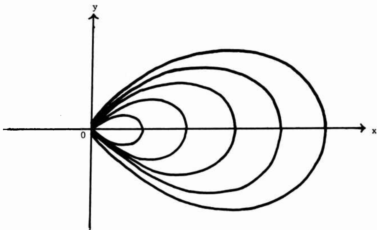
FIGURE 2. FIRE SPREAD MODIFIED BY WIND VECTOR
