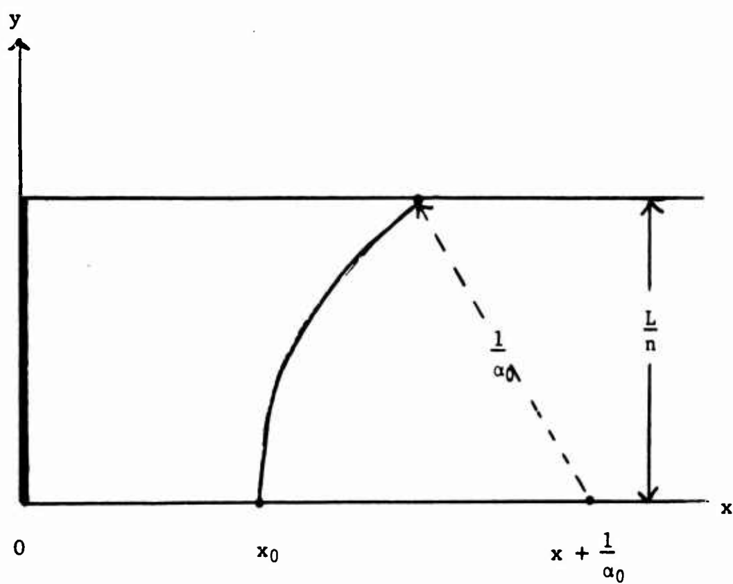
FIGURE 8. EXTREMAL FIREBREAK ( \rho \geq 1 )
