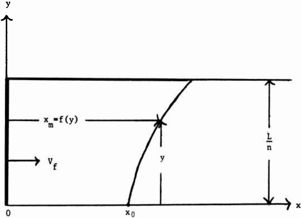
FIGURE 6. GEOMETRY OF PLANE WAVE FIREBREAK
