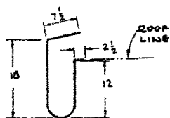
TYPICAL TROUGH SECTION
