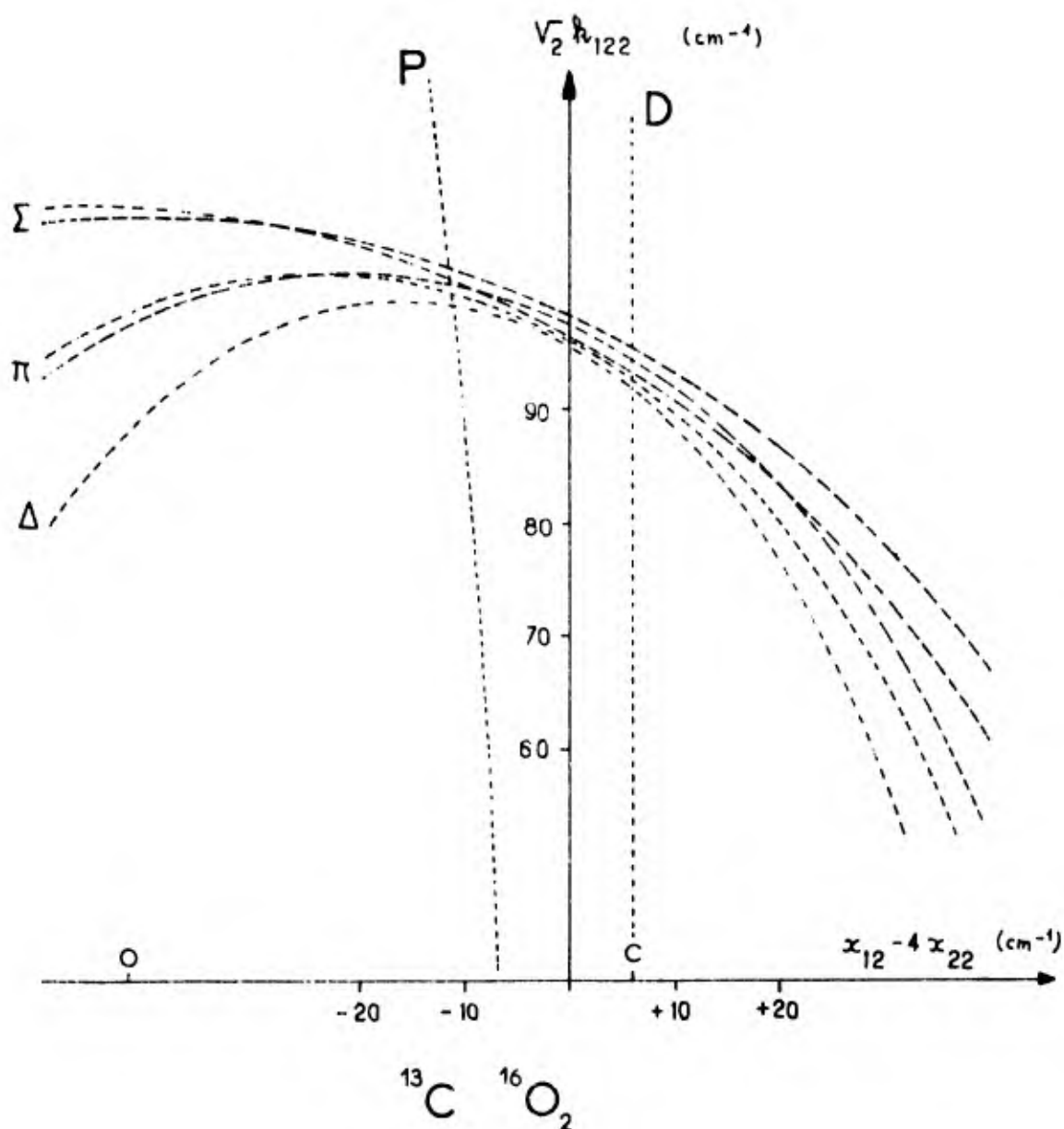
FIG. 3. Determination of (x_{12} - 4x_{22}) and k_{122} for \text{C}^{13}\text{O}_2^{16}
