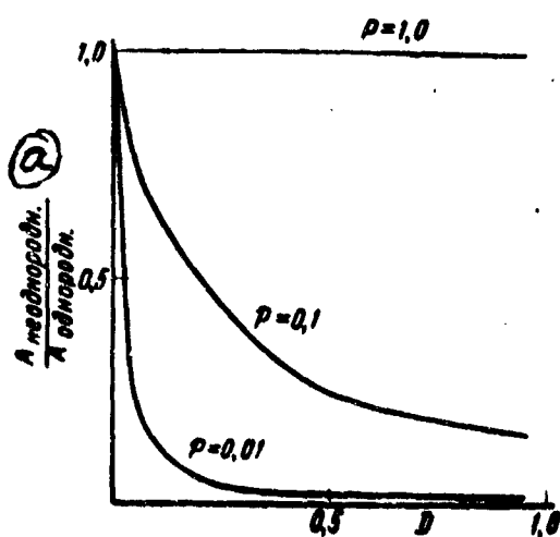
Figure 6. Relation of the coefficients of absorption of a heterogeneous object to the coefficient of absorption of a homogeneous object as the function of the optical density of the latter at various levels of disruption of homogeneity. a = A_{\text{heterogeneous}} / A_{\text{homog.}}
