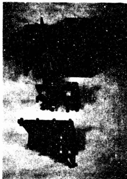
A-2 Oscillograph and Bridge Balance Box
