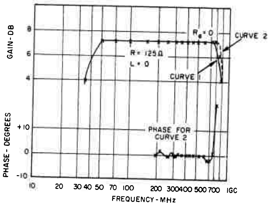
Figure 36. Emitter Feedback - Collector Base Feedback Amplifier Response Using 2N2999 in Configuration of Figure 33(b)
