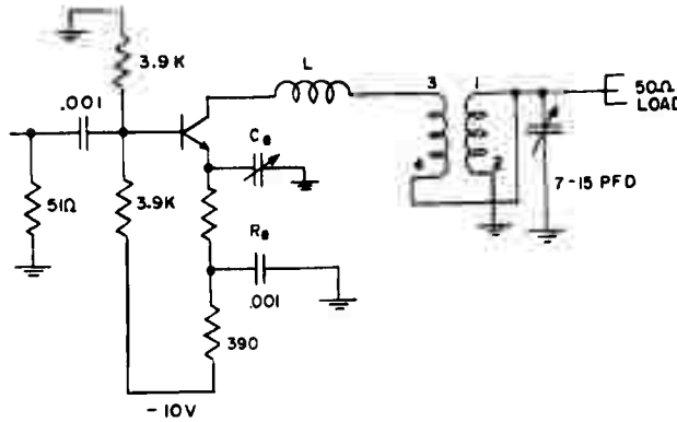
Figure 16. Emitter Feedback and Wideband Transformer With Inductive Peaking Added
