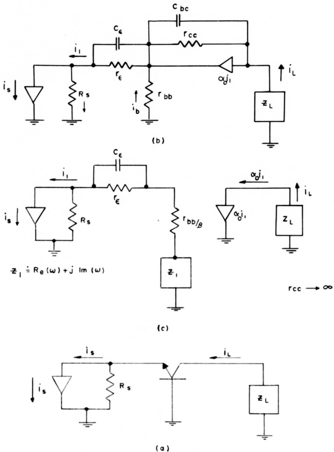
Figure 20. Grounded Base Amplifier Equivalent Circuit
