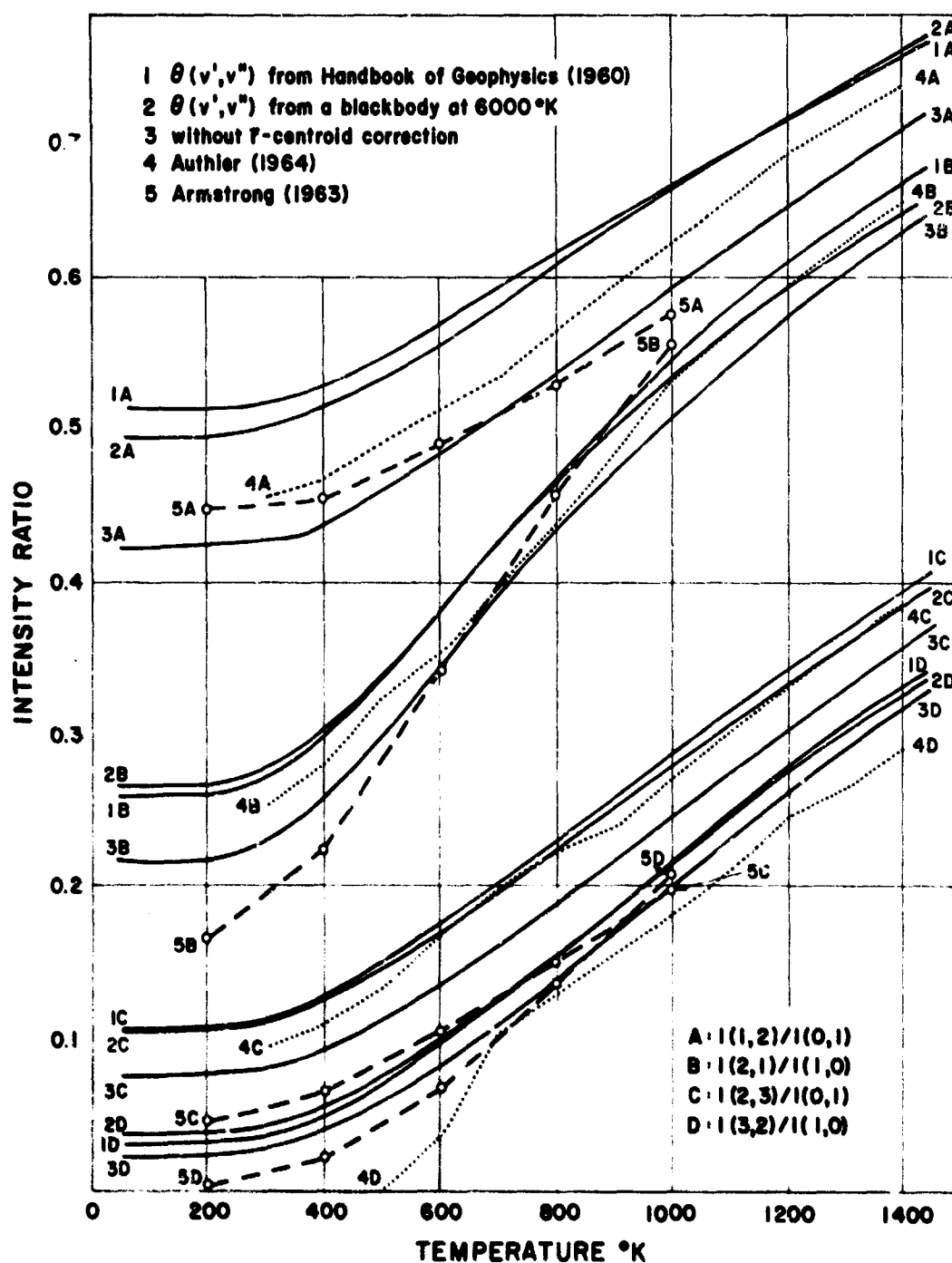
Figure 9. Intensity Ratio of Bands Within the \Delta v = +1 and -1 Sequence as a Function of Temperature
