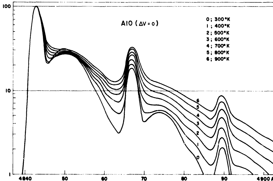
Figure 10. Synthetic Spectrum of the \Delta v = 0 Sequence for Various Temperatures, 2.5 Å Slit Function
