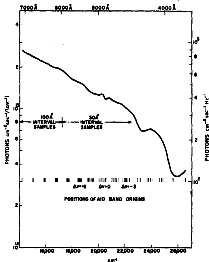
Figure 5. Photon Intensity on the Top of the Atmosphere
