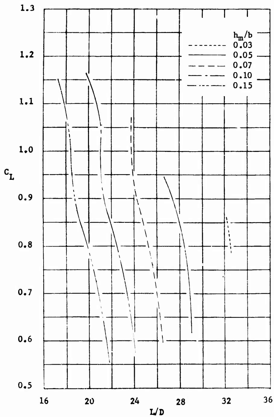
Figure 5 (Continued) (b) Concluded
