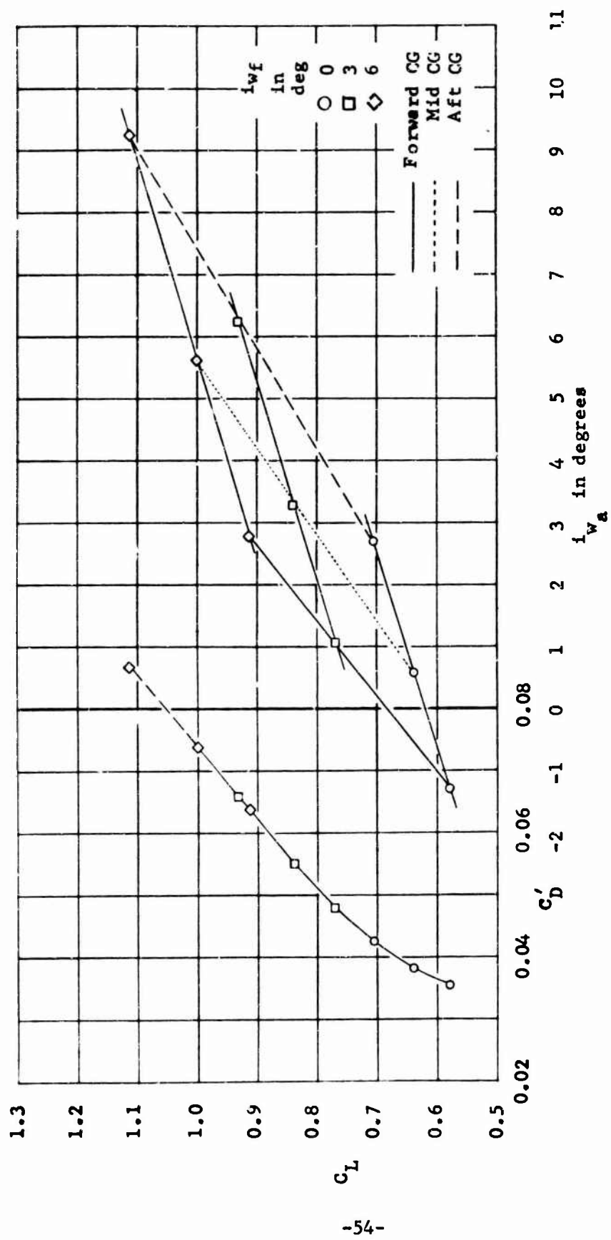
Figure 13 (Continued) (b) \alpha = 3^\circ
