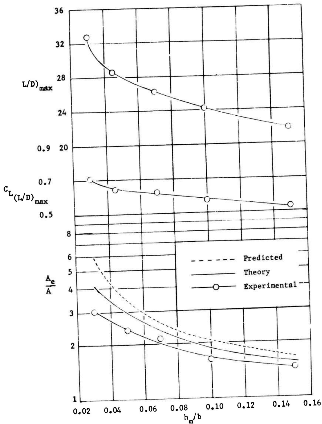
Figure 7 - Performance Parameters of Trimmed TWIG Model at Mid c.g. \alpha = 0^\circ
