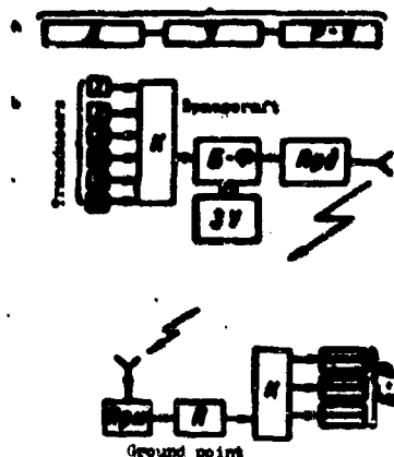
Fig. 4. Block diagram of a laboratory facility (a) and the biotelemetric system of a spacecraft (b). D) transducers; Y) amplifiers; B-P) recorders; K) commutators; B-P) telemetric signal shaping unit; 3V) memory unit; ПРД)
