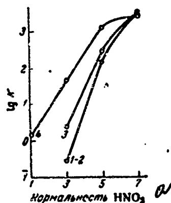
Fig. 3. Dependence of copper corrosion rate logarithm in nitric acid solutions upon its normalcy at 20^\circ : 1- \text{HNO}_3 + 5 weight % PR; 2-ditto + 1 weight % KO; 3-ditto + 5 weight % MT; 4-without decelerator. a-normalcy of \text{HNO}_3
