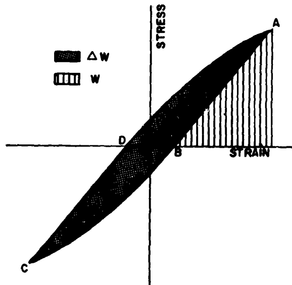
Figure 1. Hysteresis Loop in Stress-Strain Diagram (After Jenson 2 )
