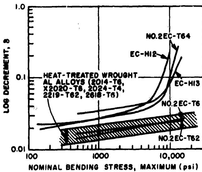
Figure 12. Low Strength Electrical Conductor Alloys have Significantly Greater Damping Capacity than Wrought Alloys (After Kaufman 10 )
