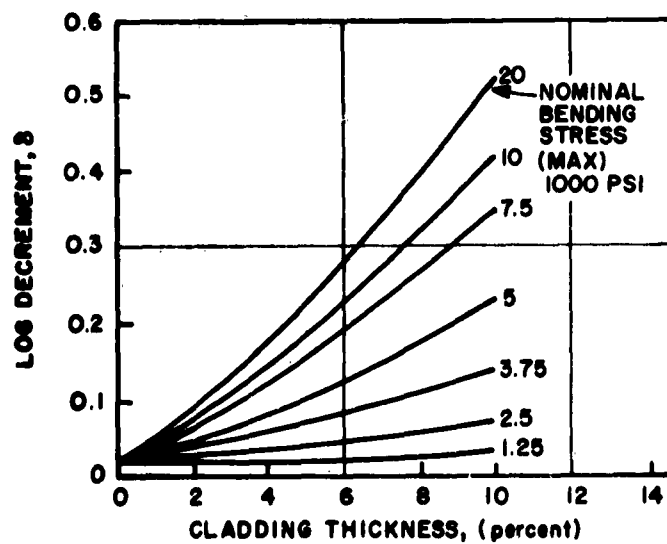
Figure 14. Cladding Increases the Damping Capacity of Aluminum Alloys. Cladding can be on One or Both Sides (After Kaufman 10 )
