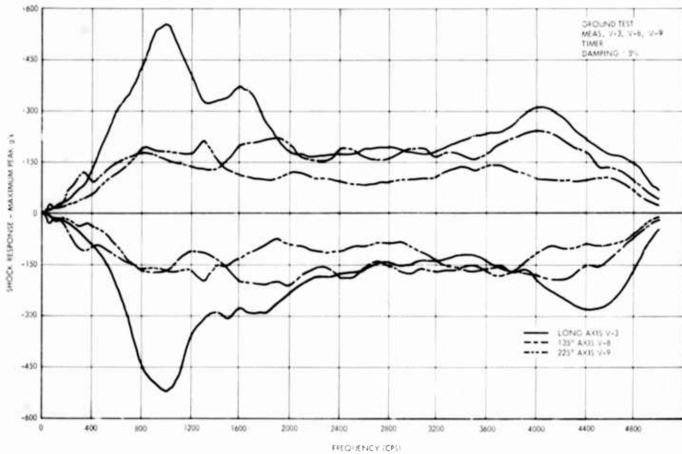
Fig. 17. Shock response spectra, ground separation test, timer
