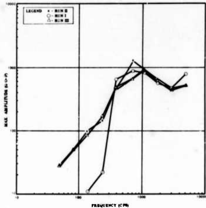
SHOCK RESPONSE SPECTRUM OF MEAS NO 23 (NOSE FAIRING BARREL NEAR RELAY BOX, RADIAL STA 149)
