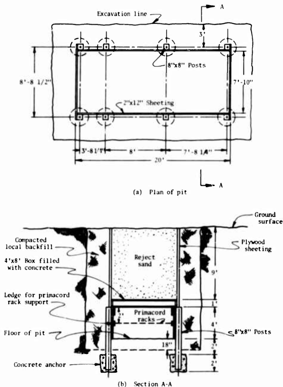
Fig. 7. Details of pit construction
