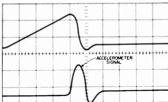
Fig. A-3. Filtered exact program before touch-up
