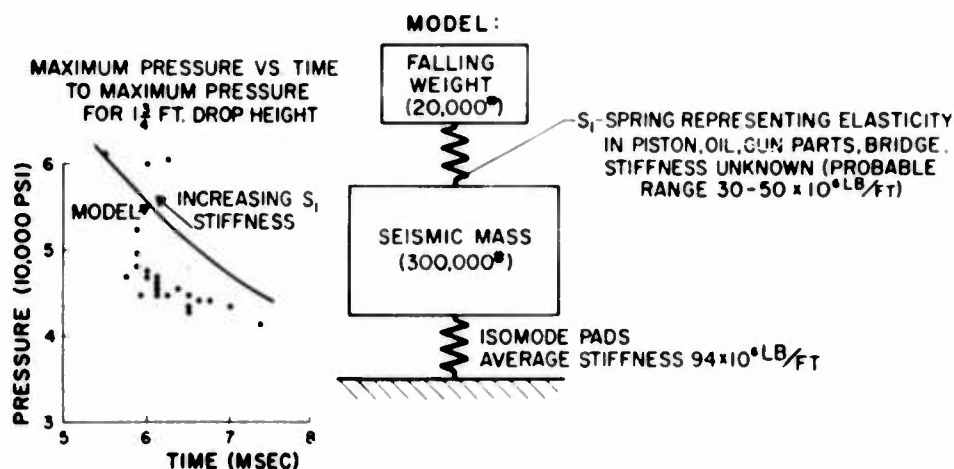
Fig. 13. Comparison of experiment with simplified analytical model
