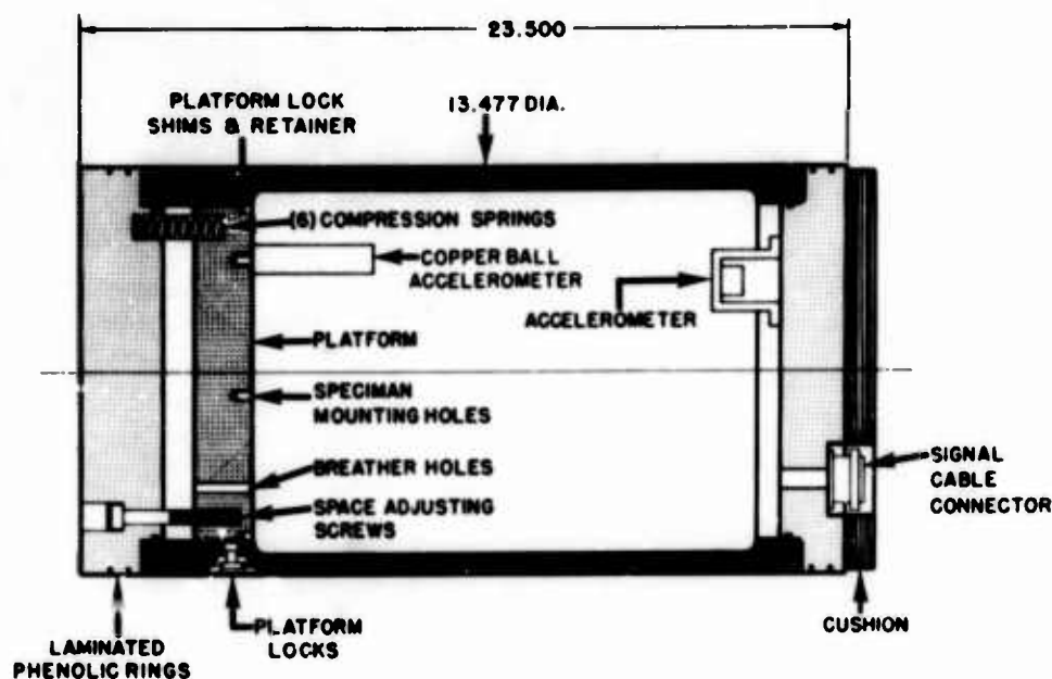
Fig. 21. Piston load (test item carriage) diagram
