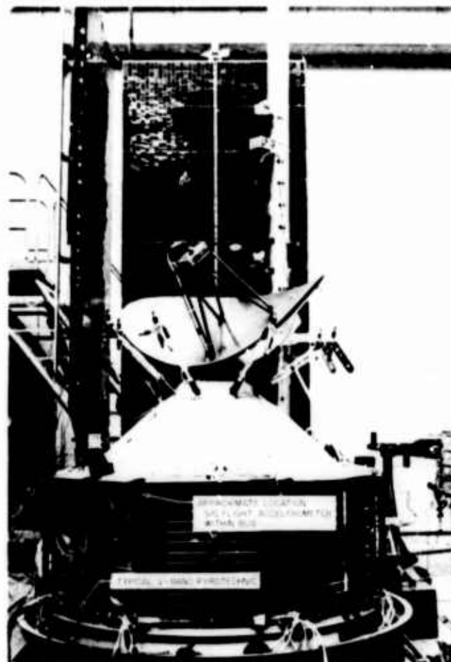
Fig. 6. Mariner Mars test configuration (two solar panels removed)
