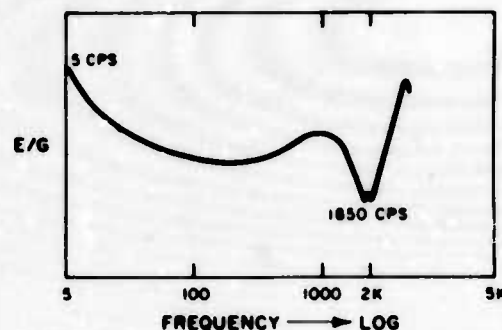
Fig. 10. C210 E/G curve
