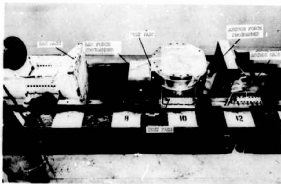
Fig. 4. Close-up of test setup -- lateral axis
