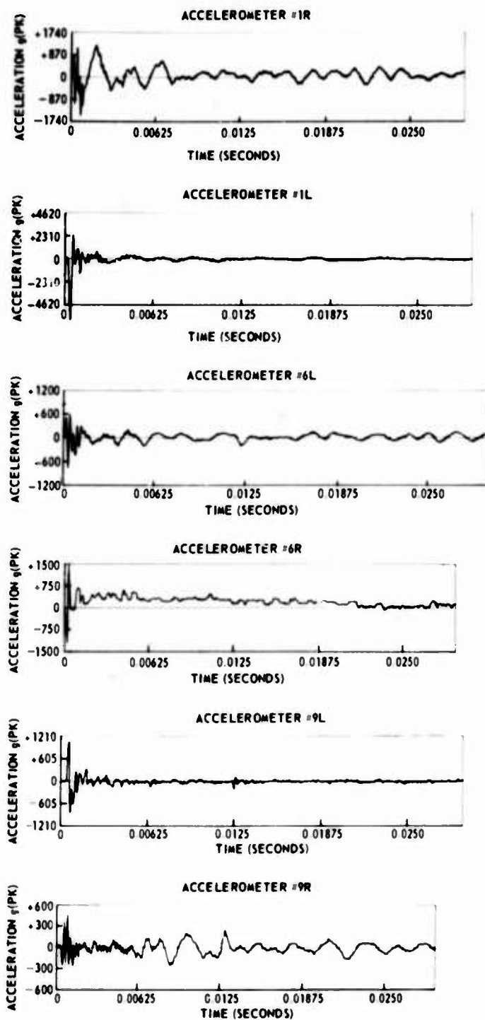
Fig. 7. Shaped charge firing at Z-13 -- test 2
