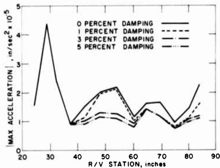
Fig. 28. Absolute max acceleration vs station lateral model
