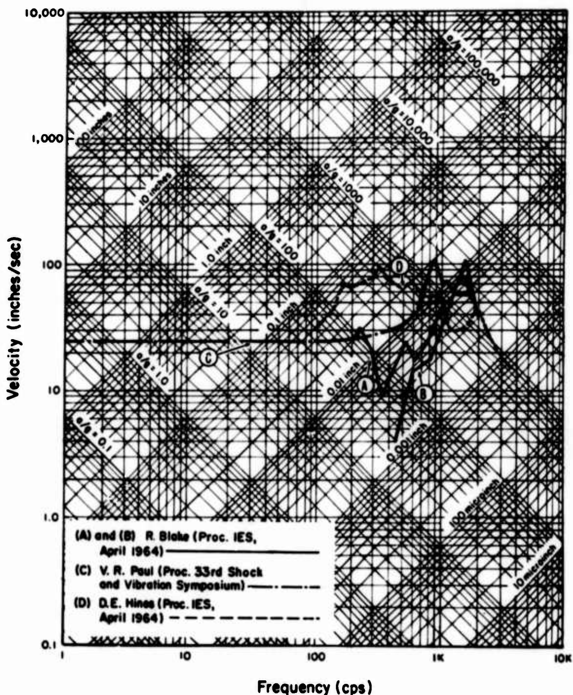
Fig. 5. Typical separation shock spectra
