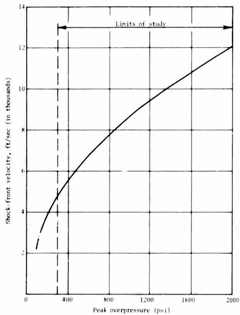
Fig. 3. Shock-front velocity vs peak overpressure
