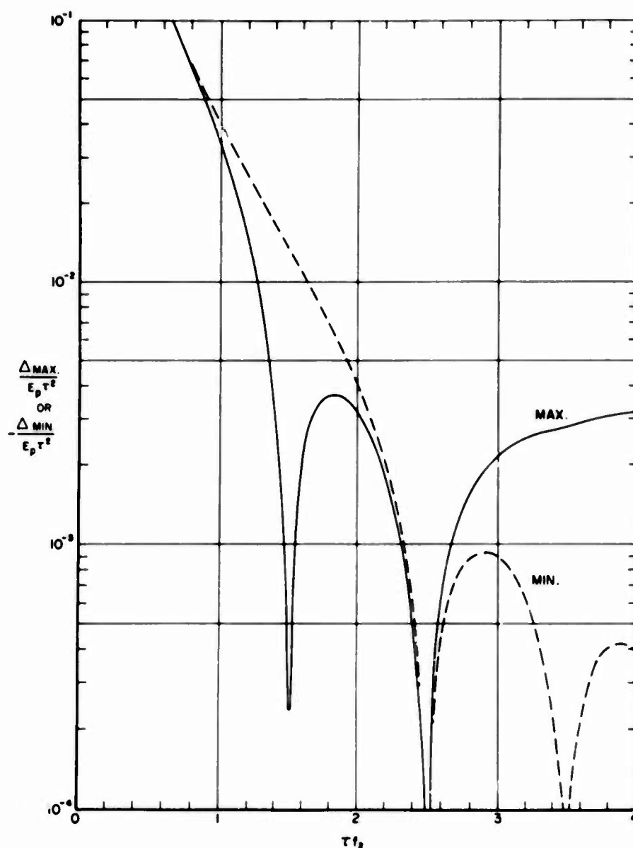
Fig. 11. Proximity spectra of half-sine excitation function when \zeta = 0.005 and \tau f_1 = 2.5
