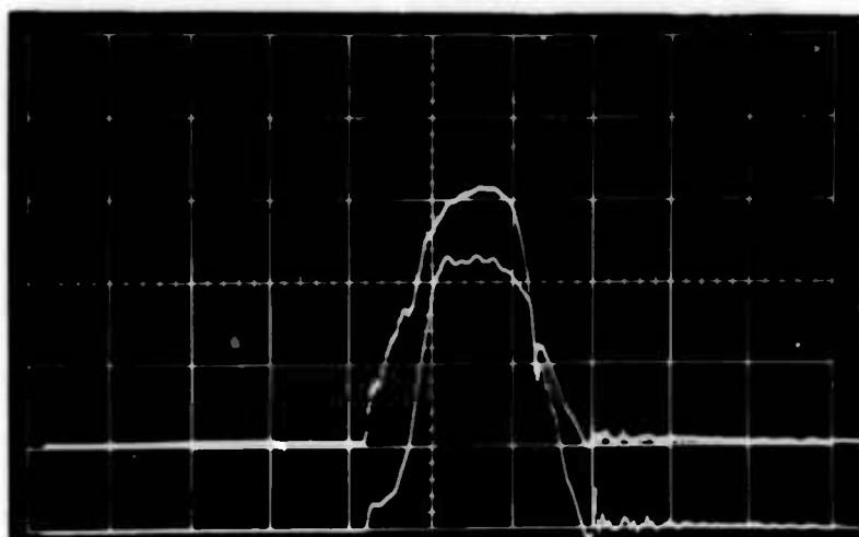
Fig. 9. Pressure-time pulse
