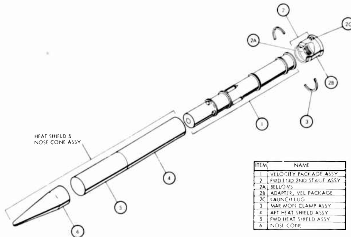
Fig. 2. Velocity package assembly
