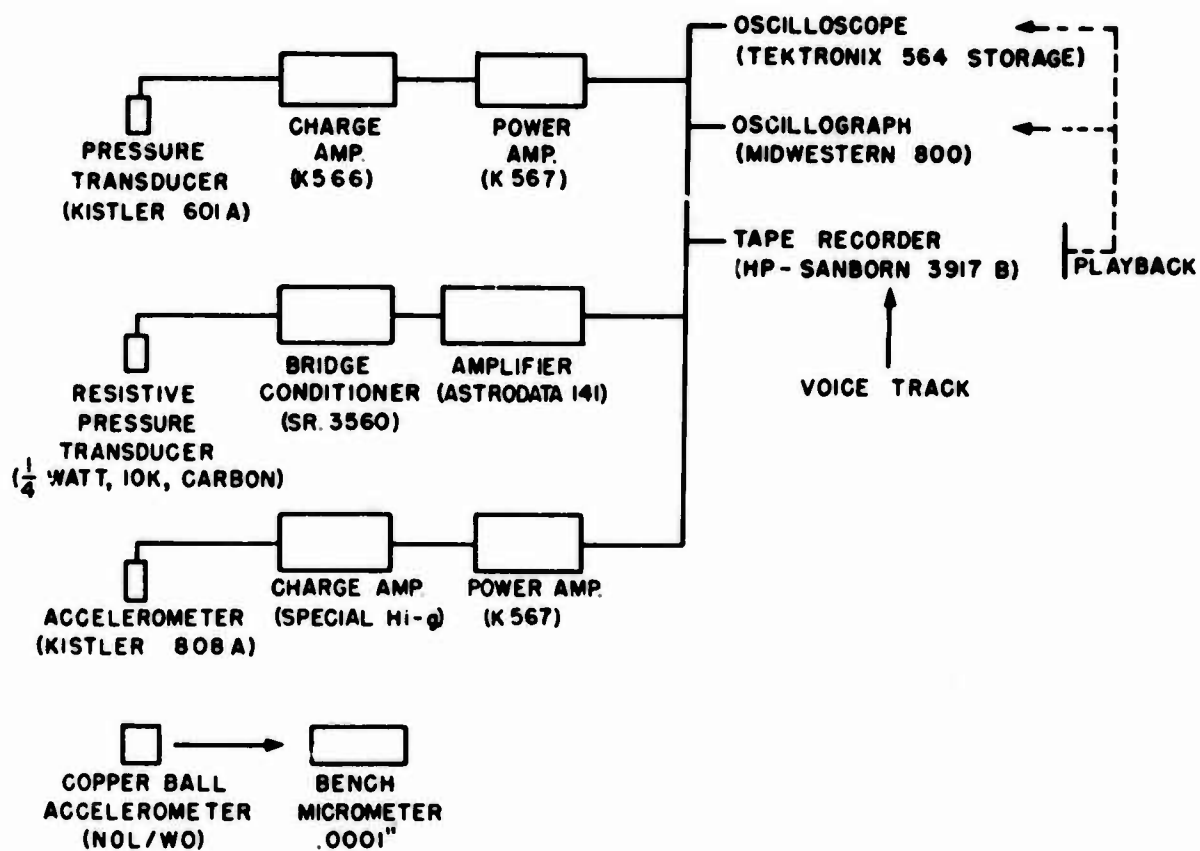
Fig. 16. Typical instrumentation block diagrams
