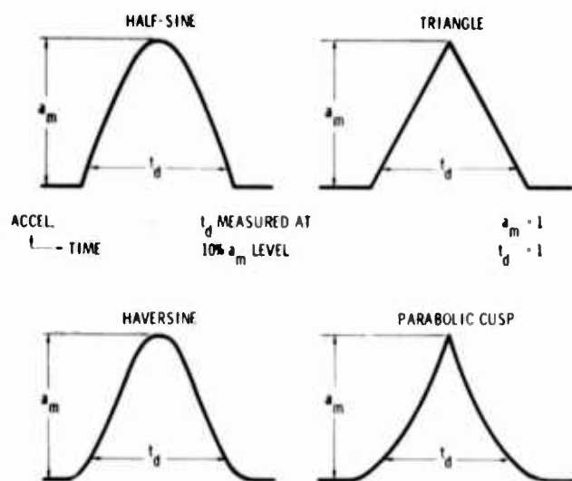
Fig. 1. Four normalized symmetrical pulse shapes
