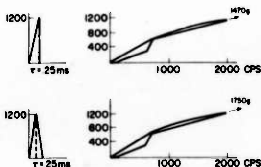
Fig. 10. Shock spectra and specification for 0.25-ms 1200-g pulse
