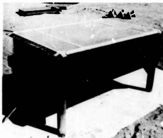
Fig. 7. Rectangular steel explosive test chamber
