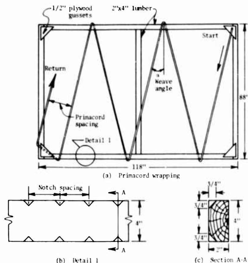
Fig. 8. Primacord racks and wrapping
