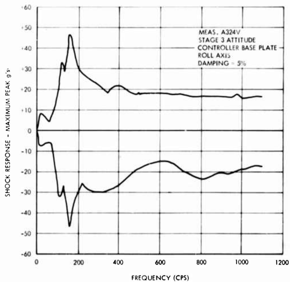
Fig. 12. Shock response spectrum, maximum envelope A-324V
