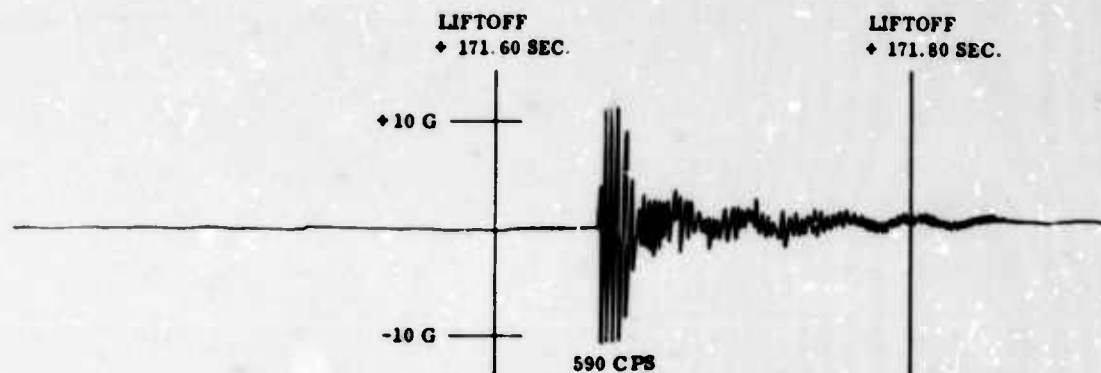
Fig. 18. Atlas-Centaur flight measurement CY540 (payload attachment No. 3, sta. 128, Z axis, IRIG telemetry channel 18)
