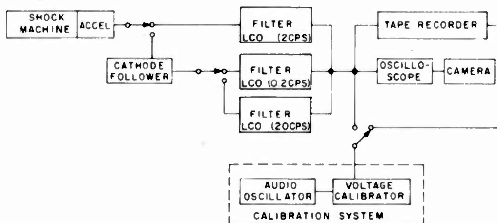
Fig. 1. Typical pulse recording system
