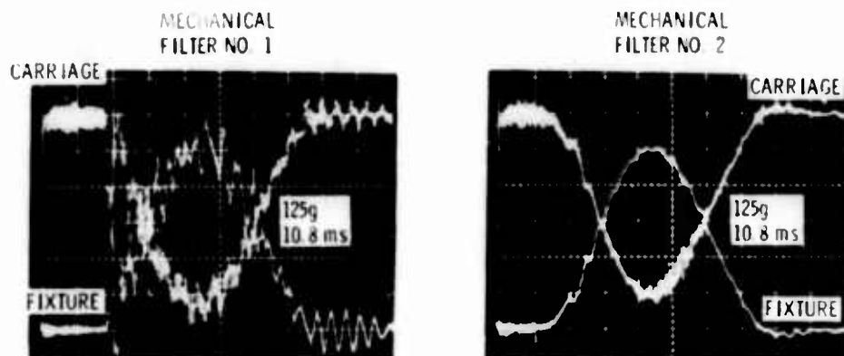
Fig. 18. Mechanical filter effect on pulse smoothing
