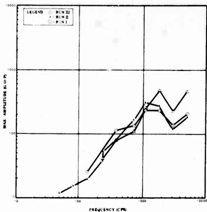
SHOCK RESPONSE SPECTRUM OF MEAS. NO. 13 (AZUSA TRANSPONDER DUMMY PACKAGE NORMAL TO BHD STA 104)
