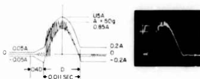
Fig. 12. Nominal 30-g 11-ms half-sine acceleration pulse; pulse same as shown in Fig. 11 except filter cutoff set at 1200 cps; response down; 1 db (10 percent) at 450 cps; \Delta V_m = 6.05 fps; \Delta V_i = 6.15 fps
