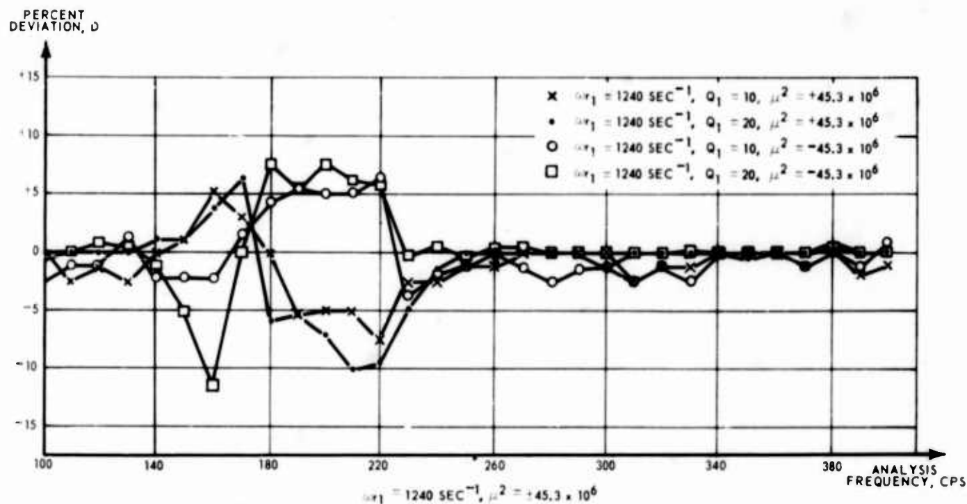
Fig. 9. Deviations in shock spectra due to Q_1
