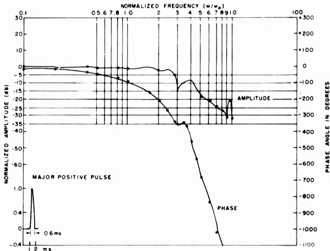
Fig. 4. Typical Bode diagram of 180-JAN shock machine pulse (major positive pulse)
