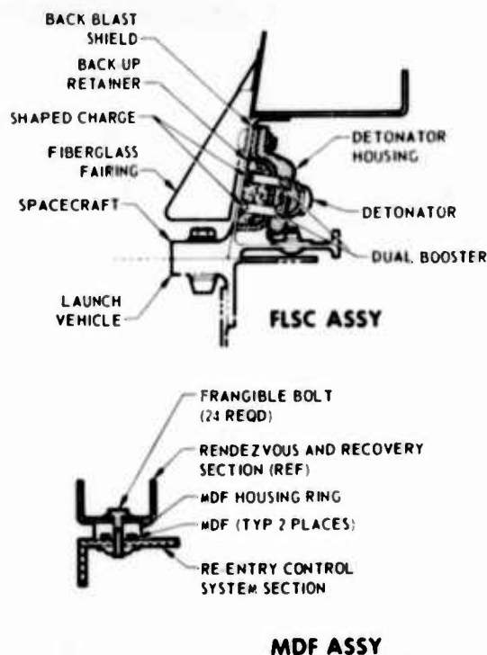
Fig. 3. Pyrotechnic assemblies
