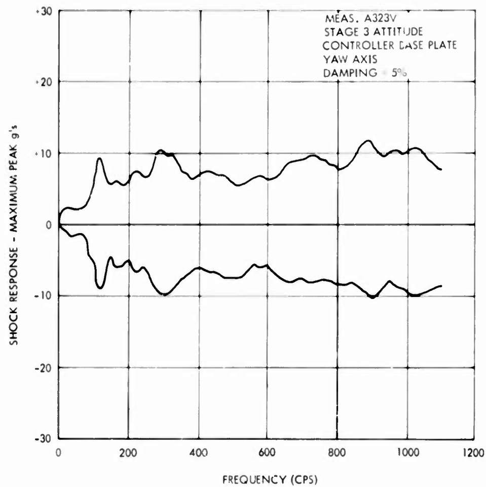
Fig. 11. Shock response spectrum, maximum envelope A-323V
