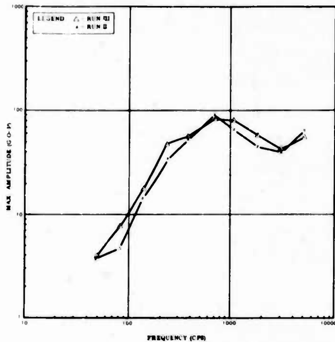
SHOCK RESPONSE SPECTRUM OF MEAS NO 20 (AT PAYLOAD LATCH Z AXIS STA 128 - 129°)
