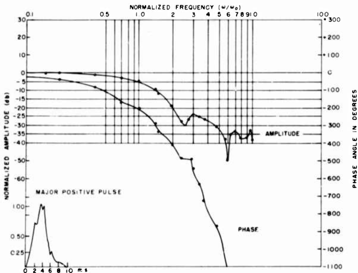
Fig. 14. Typical Bode diagram of Barry 20VI shock machine pulse
