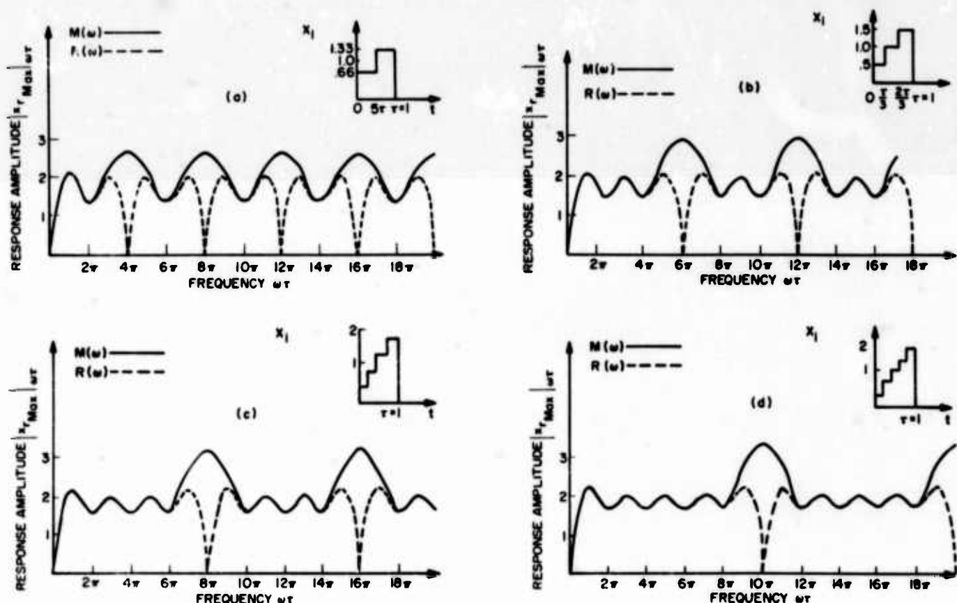
Fig. B-1. Shock spectra for step-type pulses
