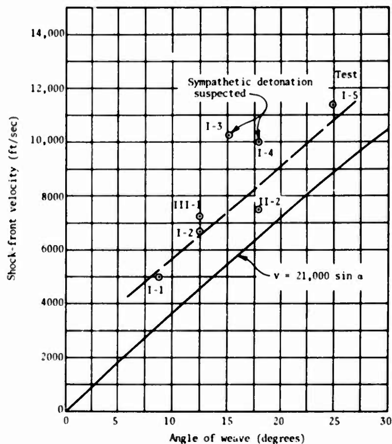
Fig. 14. Shock-front velocity vs angle of weave
