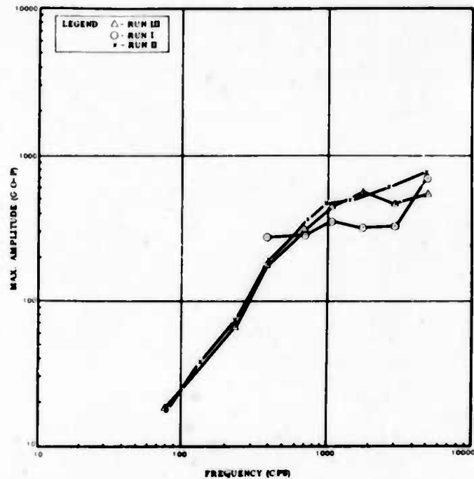
SHOCK RESPONSE SPECTRUM OF MEAS NO 22 (NOSE FAIRING BARREL AT RELAYS Z AXIS STA 149)
