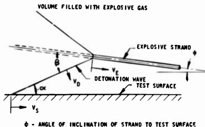
Fig. 4. Detonation wave initiated by solid explosive strand, general case
