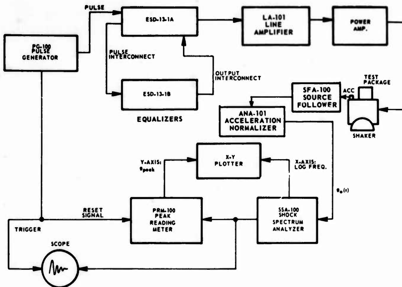
Fig. 1. Electrodynamic shaker shock synthesis and analysis system
