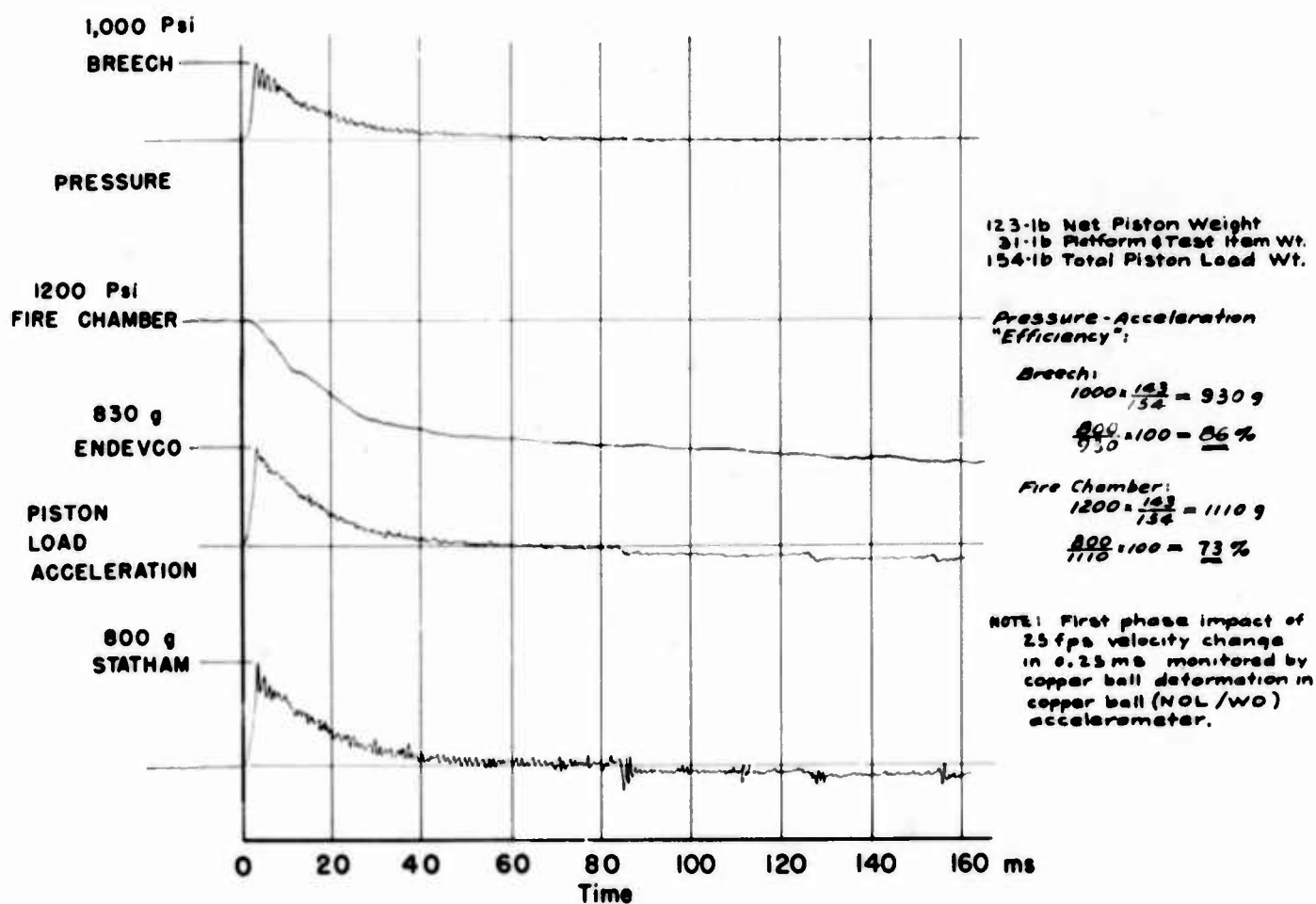
Fig. 30. Typical test shot responses
