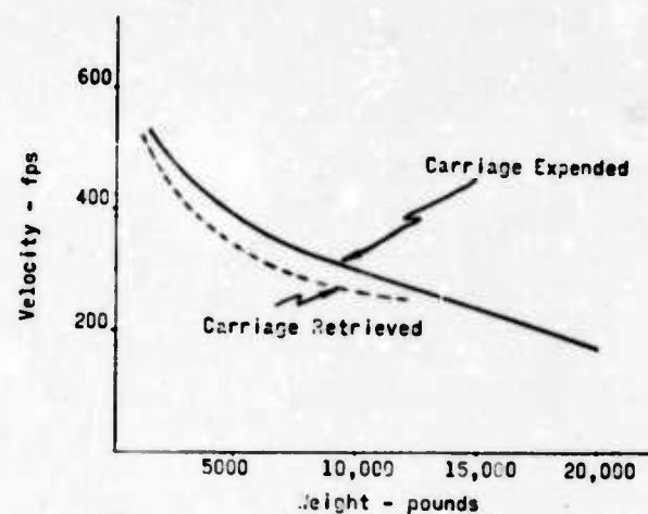
Fig. 7. Predicted maximum velocity capability of water jet catapult vs carriage weight
