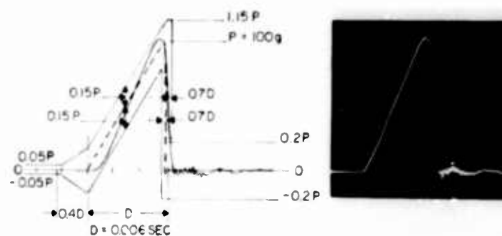
Fig. 25. Nominal 100-g 6-ms terminal-peak sawtooth pulse, unfiltered; total impact weight 98 lb; \Delta V_m = 10 fps; \Delta V_i = 9.66 fps
