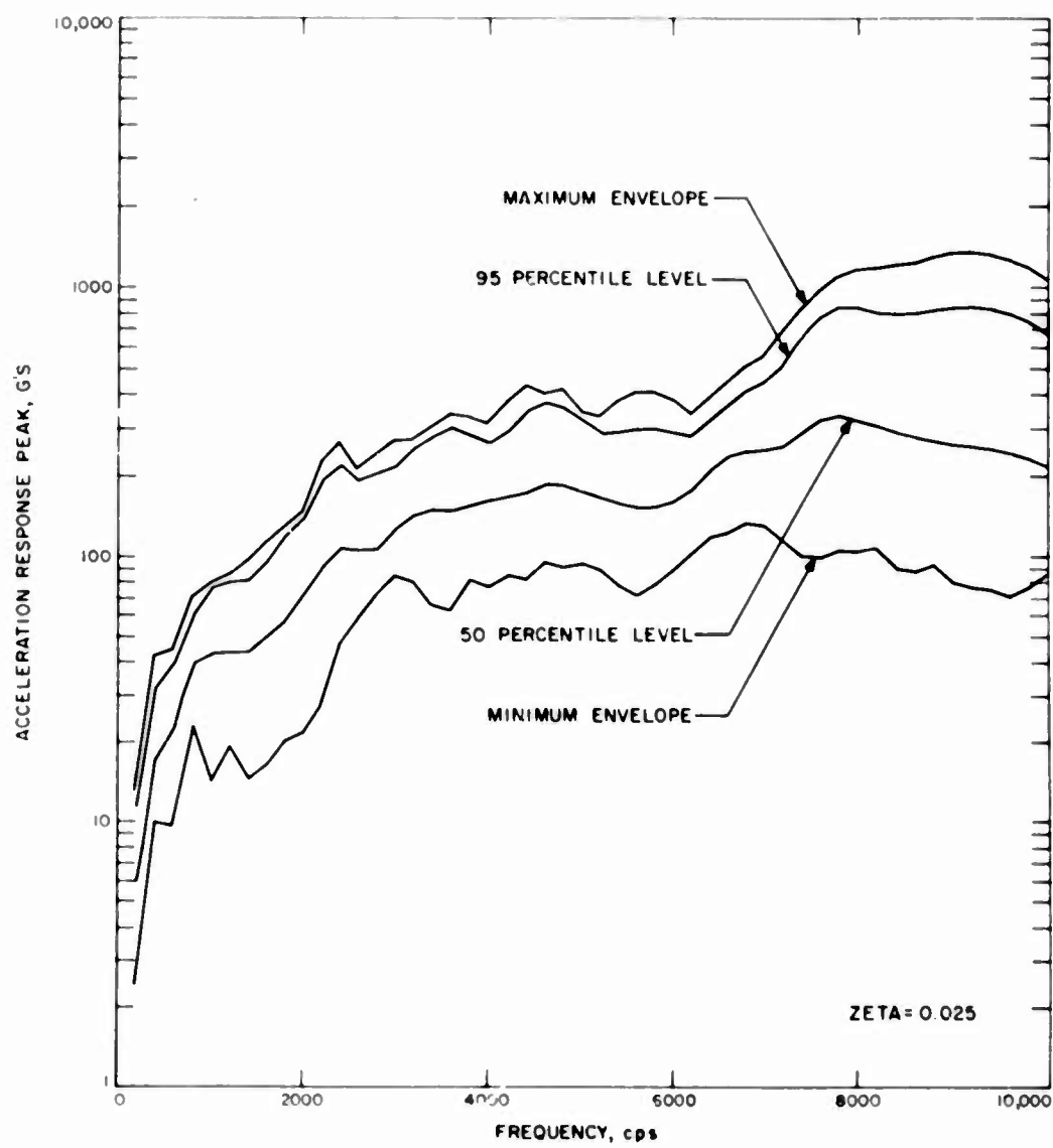
Fig. 12. Ranger Case IV response to mechanical separation
