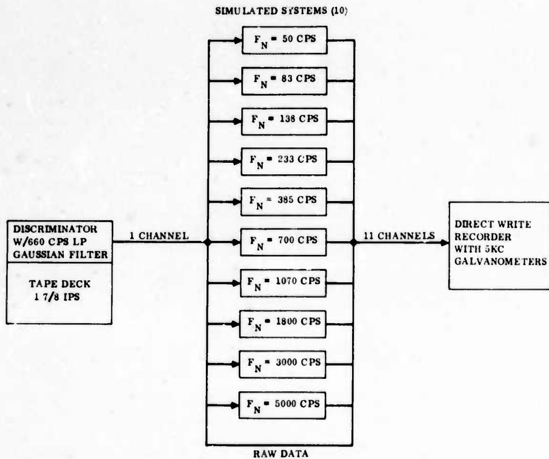
Fig. 8. Shock spectrum analyzer block diagram
