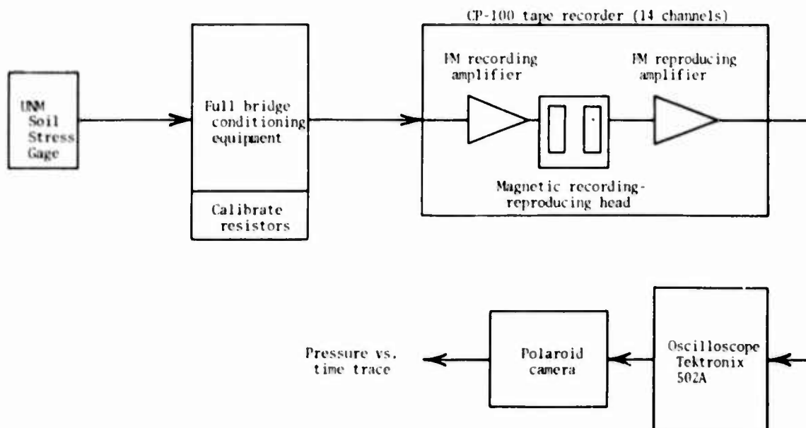
Fig. 11. Schematic of electronic recording system
