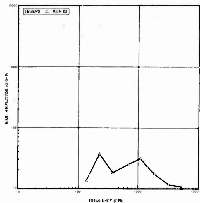
SHOCK RESPONSE SPECTRUM OF MEAS NO 23 (AT BASE OF RELAY INSIDE OF TELEPAK, STA 170)
