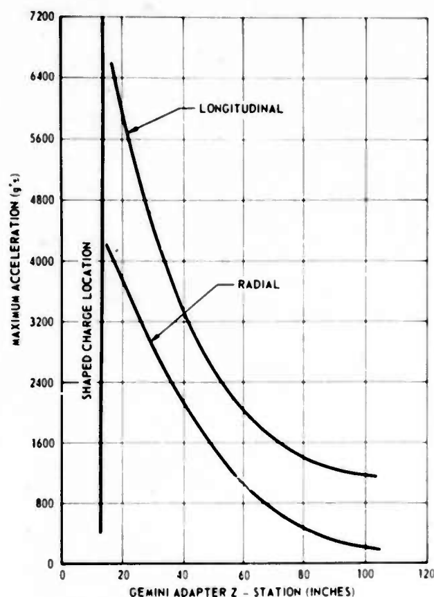
Fig. 12. Impulse attenuation -- Z-13 firing, 10 grains/ft
