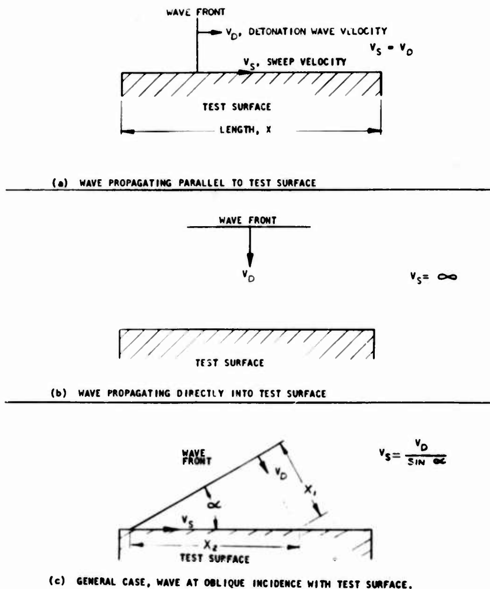
Fig. 2. Examples of detonation wave intercepting test surface
