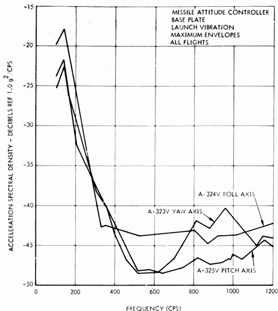
Fig. 6. Acceleration spectral density, Stage 3
