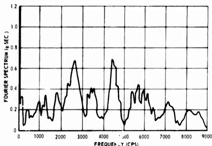
Fig. 23. Shaped charge firing at Z-69 -- test 2, accelerometer 9L
