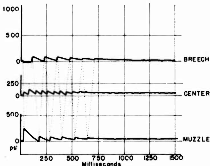
Fig. 24. Barrel air pressure vs time, without load
