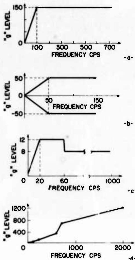
Fig. 5. Typical shock spectra specifications
