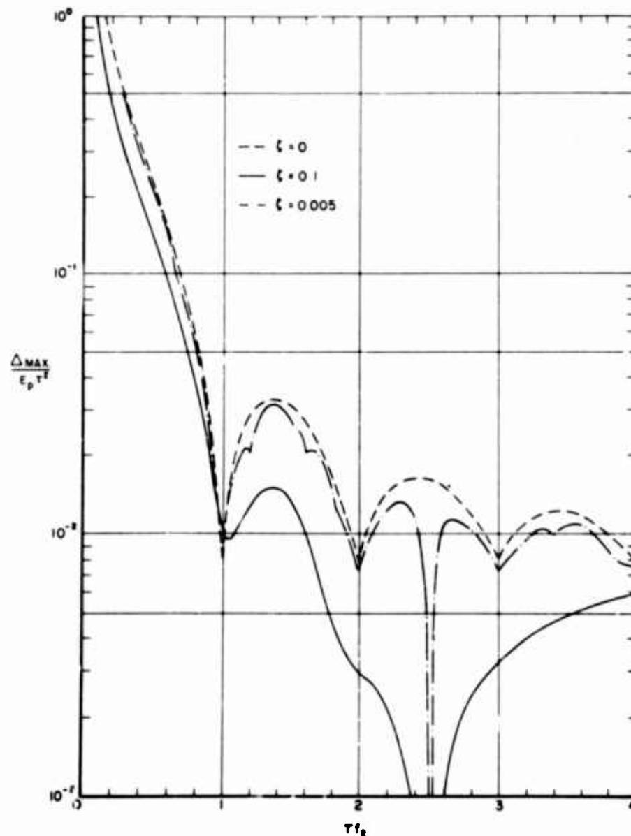
Fig. 15. Effects of damping on positive proximity spectra of square wave excitation function when \tau f_1 = 2.5
