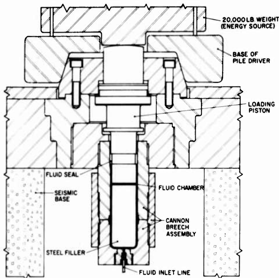
Fig. 1. Sectional view of impact test facility
