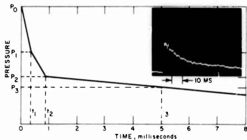
Fig. 13. Idealized pressure pulse applied to cylinder end
