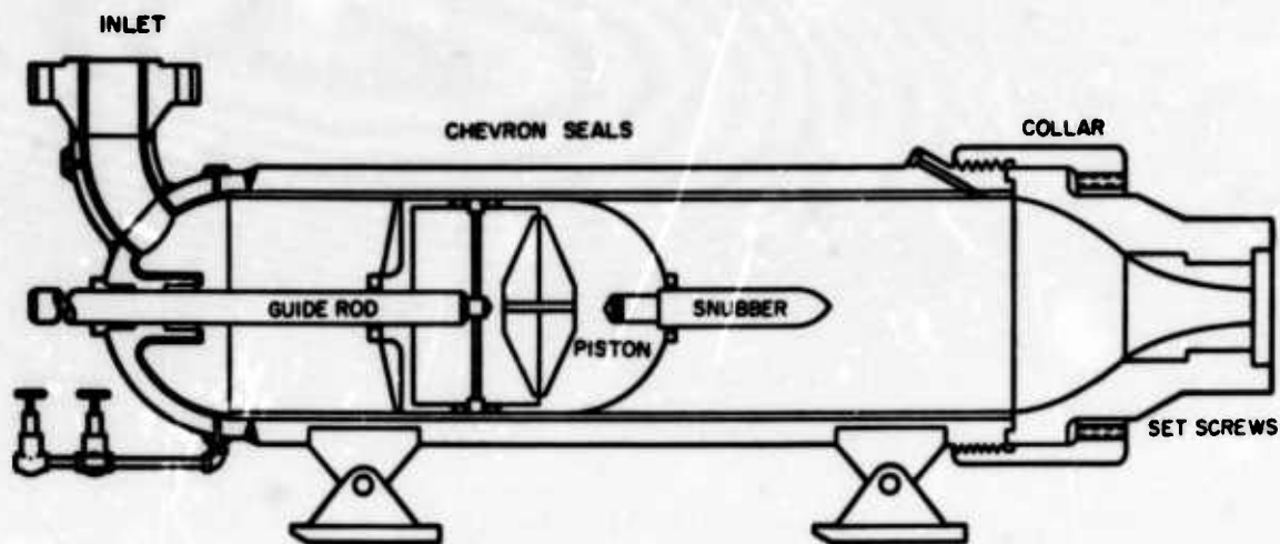
Fig. 4. Plenum assembly for water jet catapult
