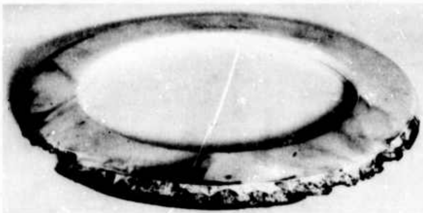
Fig. 3. Firing valve seal after first shot, fire pressure of 1500 psi
