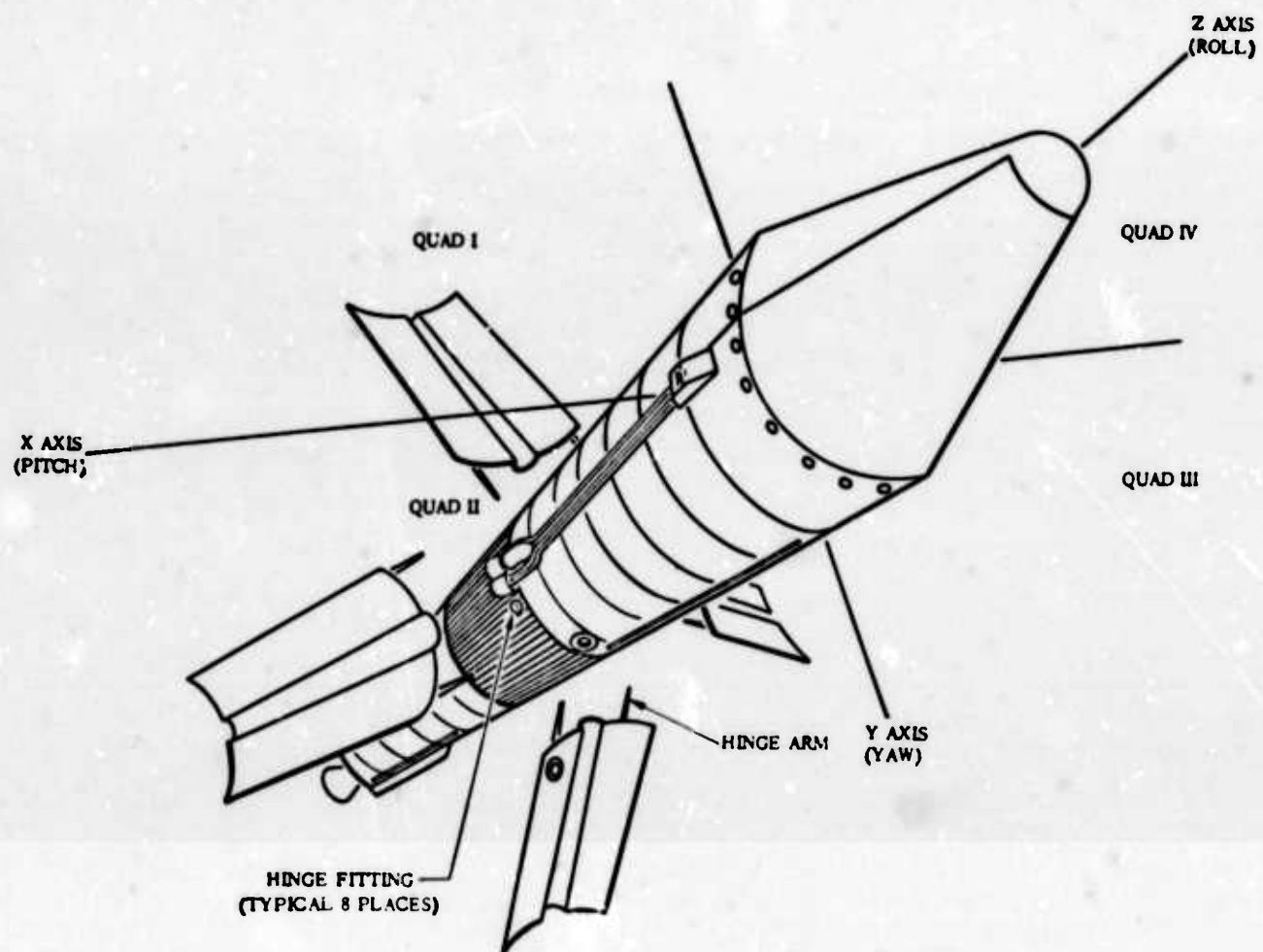
Fig. 1. Centaur jettisonable insulation system
