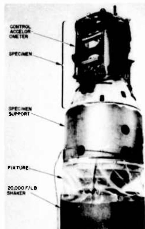
Fig. 7. Test specimen mounted on 20,000-force pound shaker for shock testing
