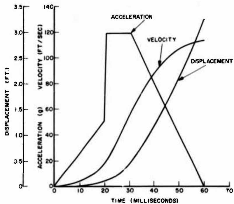
Fig. 9. Stationary sled acceleration, velocity, and displacement curves
