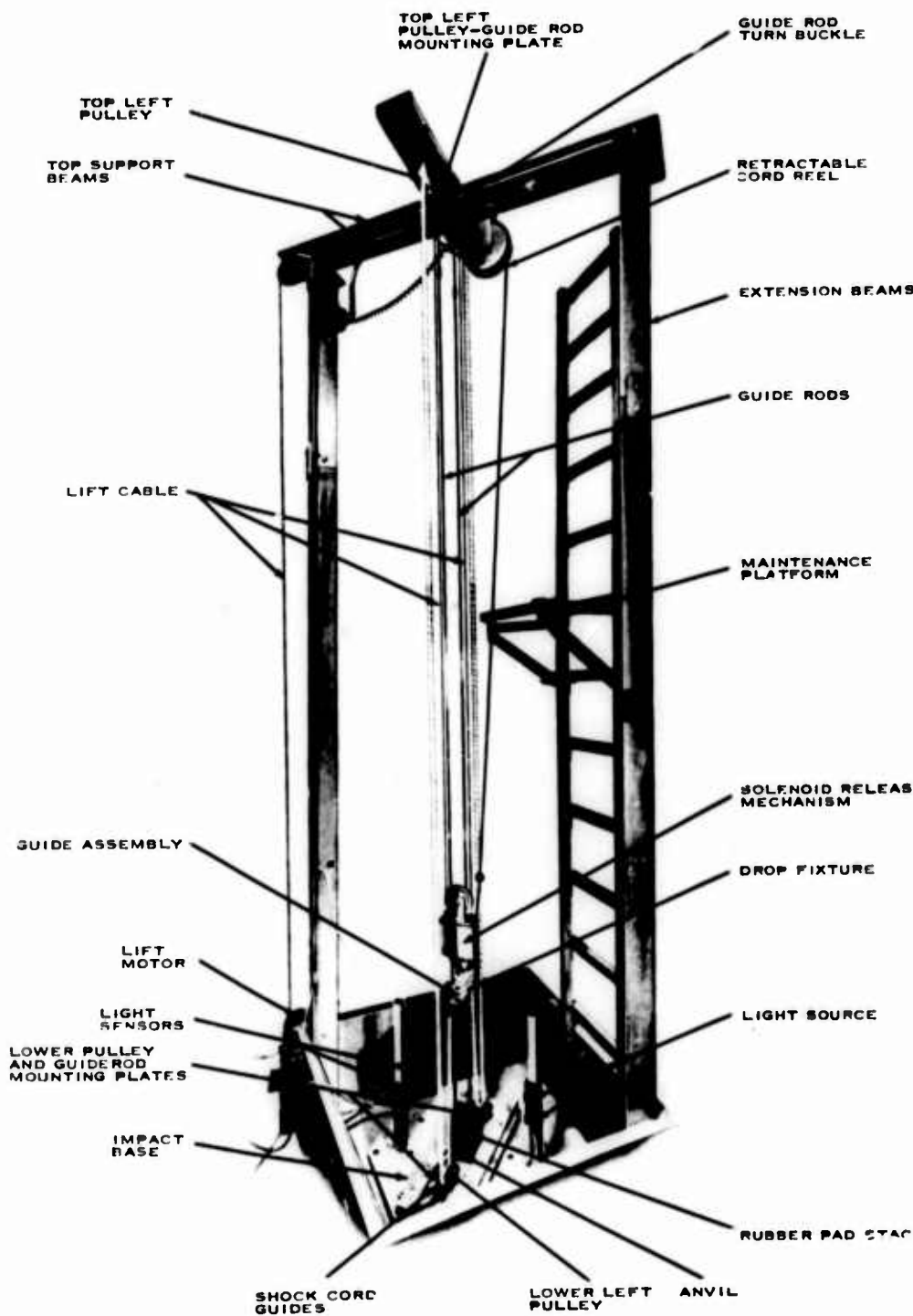
Fig. 2. Slingshot shock machine
