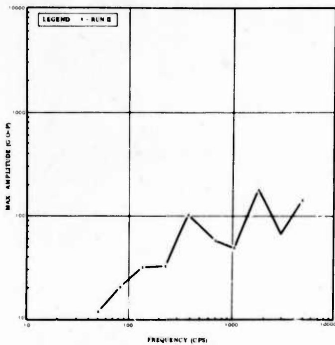
SHOCK RESPONSE SPECTRUM OF MEAS NO 16 (RANGE SAFETY POWER CONTROL BOX Z AXIS STA 164)
