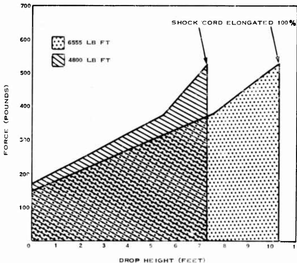
Fig. 1. Force deflection curves of shock machine using 3/4-in. shock cords
