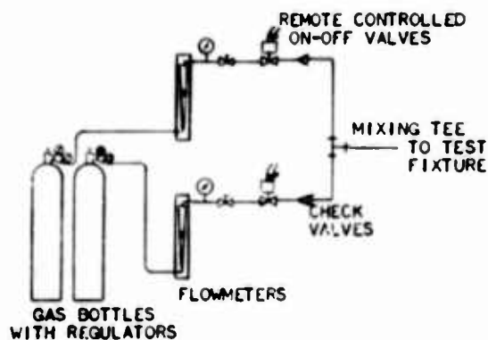
Fig. 5. Schematic diagram of gas metering equipment
