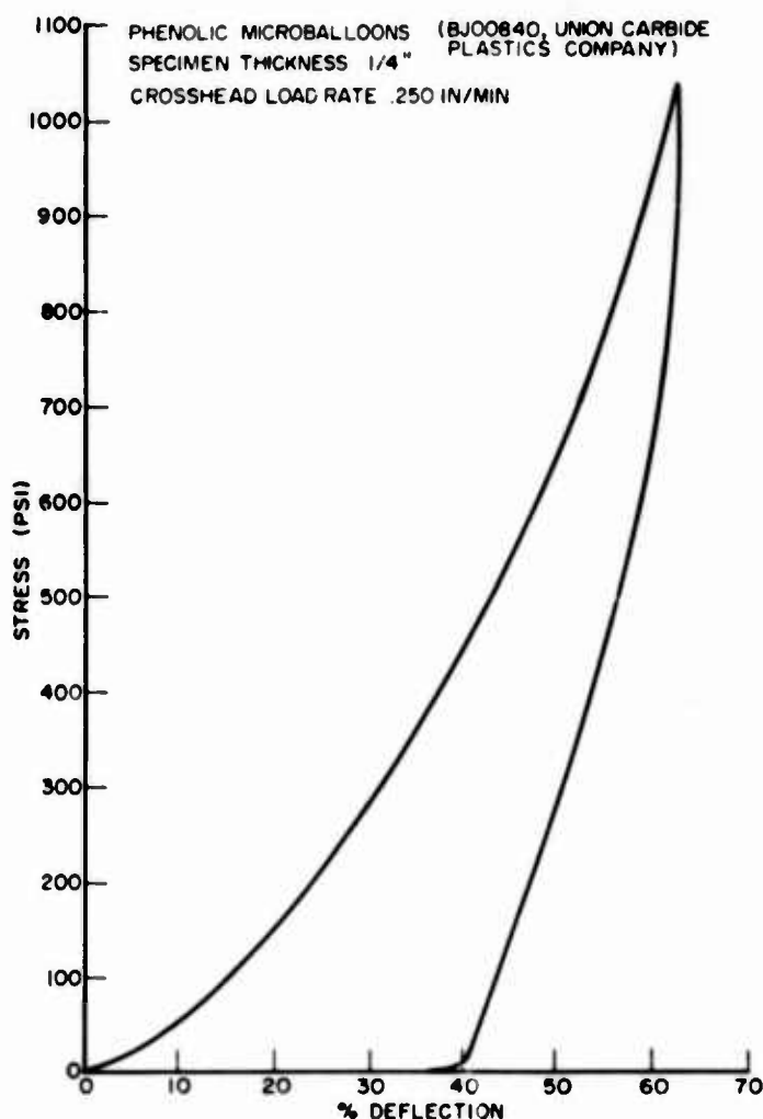
Fig. 6. Phenolic microballoon stress-strain curve
