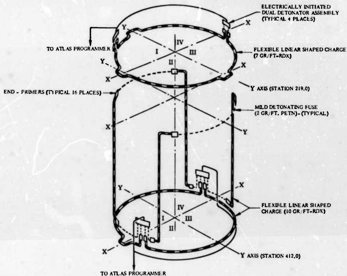
Fig. 2. Insulation panel shaped charge separation system
