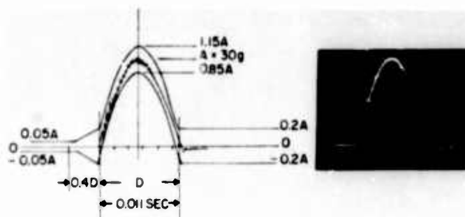
Fig. 11. Nominal 30-g 11-ms half-sine acceleration pulse, unfiltered; total impact weight 200 lb
