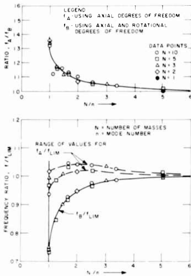
Fig. 12. Correlation of frequency ratios with N/n
