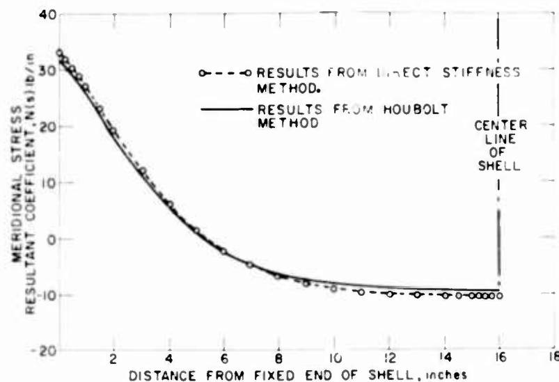
Fig. 20. Comparison of static analyses
