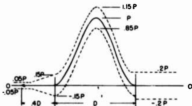
Fig. 4. Versed-sine, or haversine, acceleration pulse with tolerance envelopes. Maximum value is P and duration is D. Tolerance curves are obtained by translating the versed-sine curve upward and downward a distance of 0.15P. Velocity change associated with pulse is \Delta V_i = 0.5DP (D expressed in seconds and P as acceleration).
