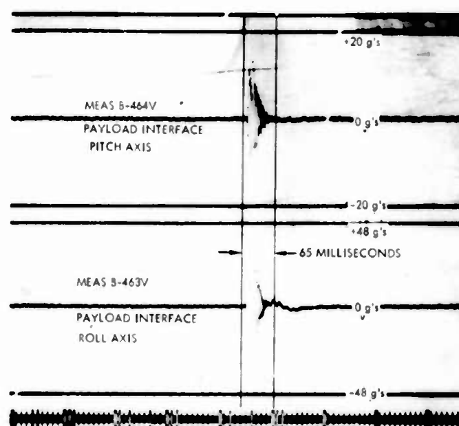
Fig. 7. Typical third stage ignition acceleration transient
