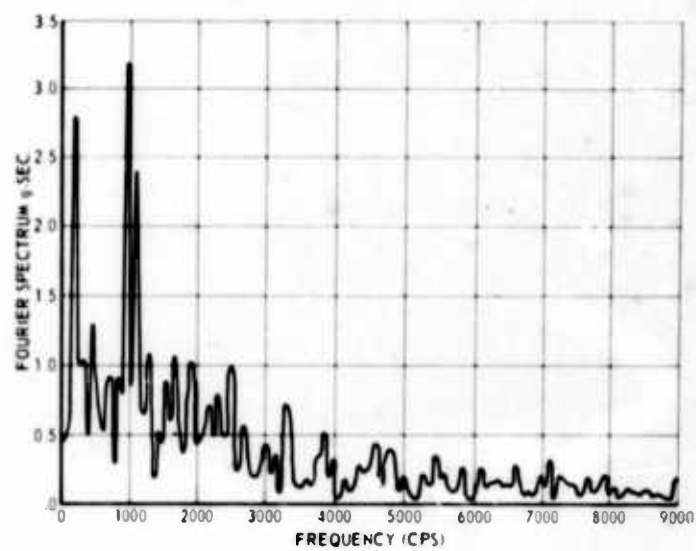
Fig. 14. Fourier amplitude spectrum-- test 1, accelerometer 7R
