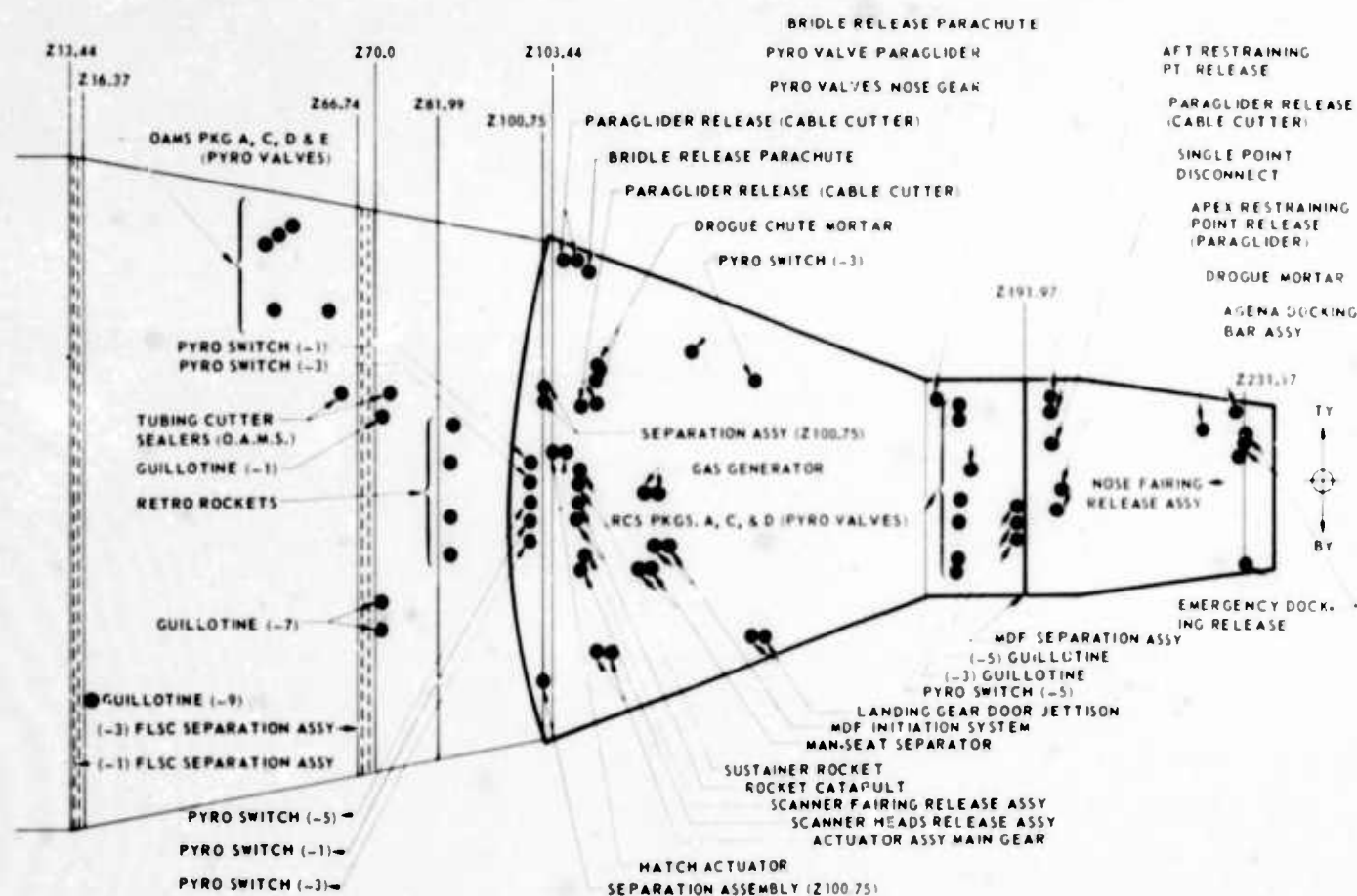
Fig. 1. Gemini spacecraft pyrotechnic locations
