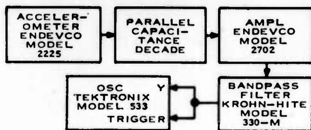
Fig. 9. Shock pulse instrumentation, block diagram
