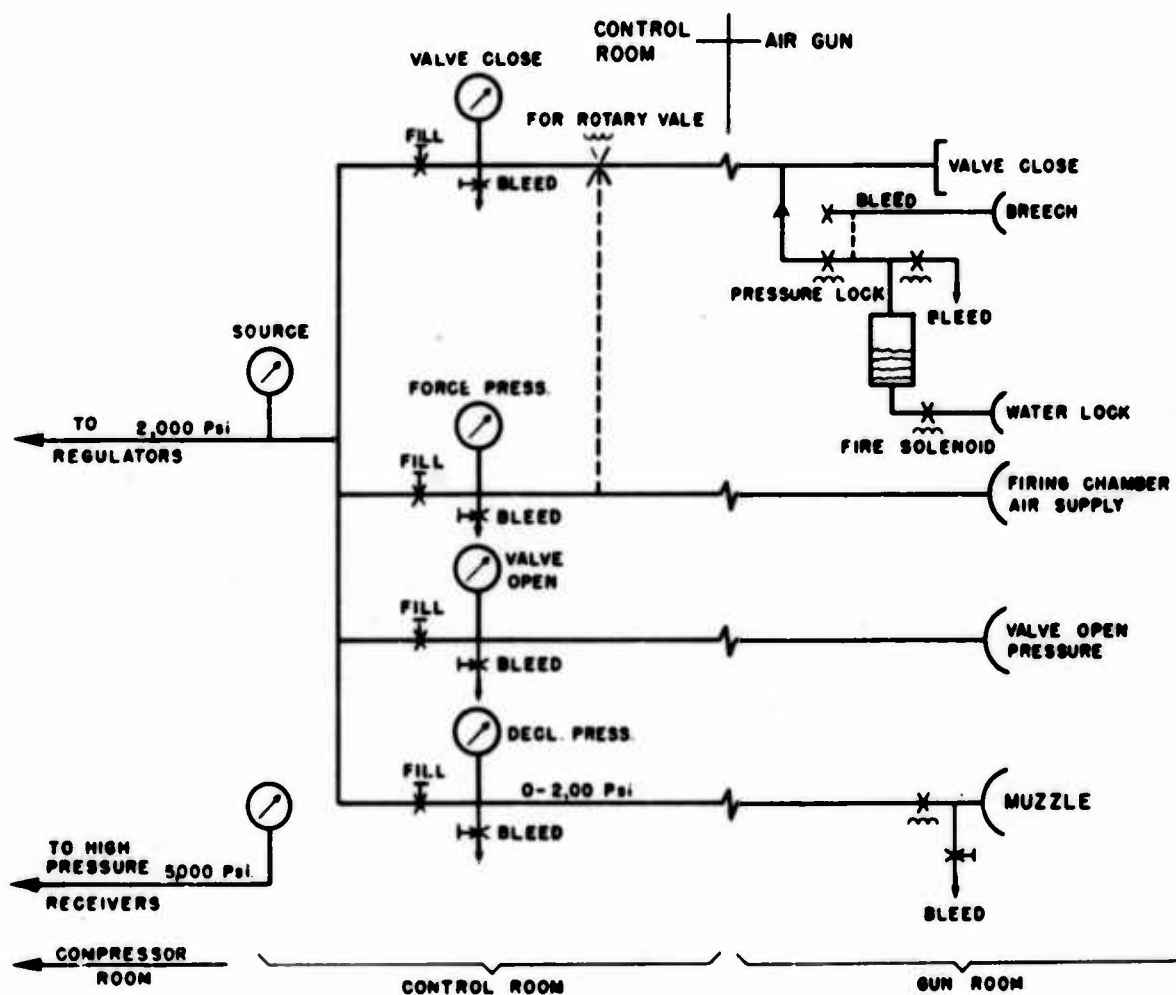
Fig. 14. Pneumatic control diagram
