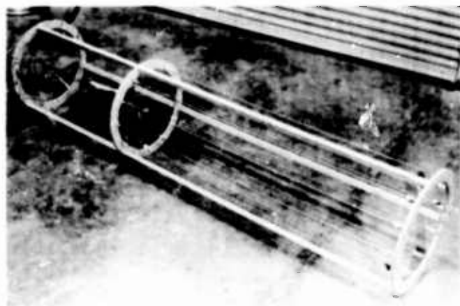
Fig. 9. Explosive strand array for 16-in. tube test
