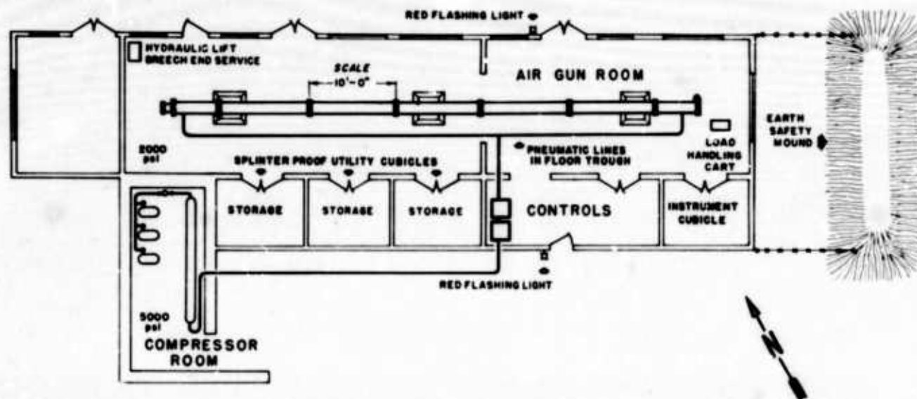
Fig. 1. Seal Beach 13-1/2-in. air gun facility arrangement
