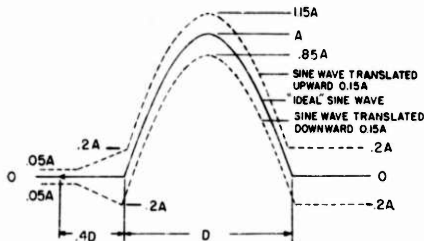
Fig. 2. Half-sine acceleration pulse with tolerance envelopes. Amplitude of pulse is A and duration is D. Velocity change associated with pulse is \Delta V_i = 0.636DA (D expressed in seconds and A as acceleration). \Delta V_m (measured) must be equal to \Delta V_i \pm 10 percent. Tolerances proposed for a revision of MIL-STD-202, method 213.
