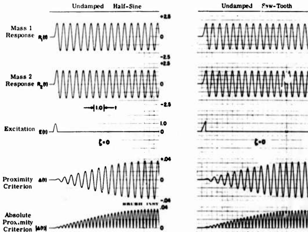
Fig. 2. Proximity criteria for half-sine and sawtooth pulses
