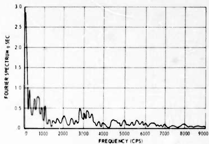
Fig. 13. Fourier amplitude spectrum -- test 1, accelerometer 4R
