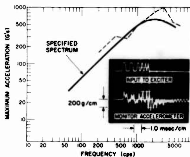
Fig. 4. Shock response spectrum for compound pulse input
