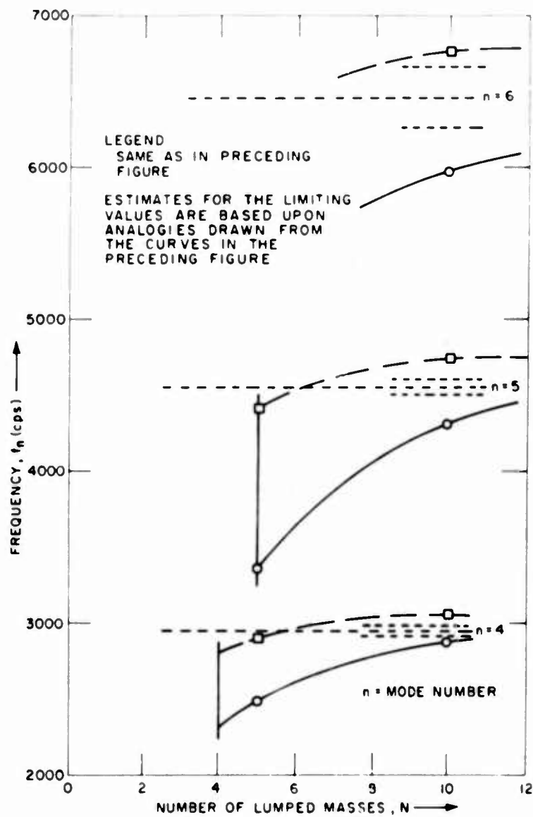
Fig. 11. Frequency vs number of masses
