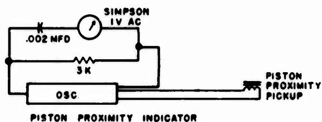
Fig. 15. Electric control diagram
