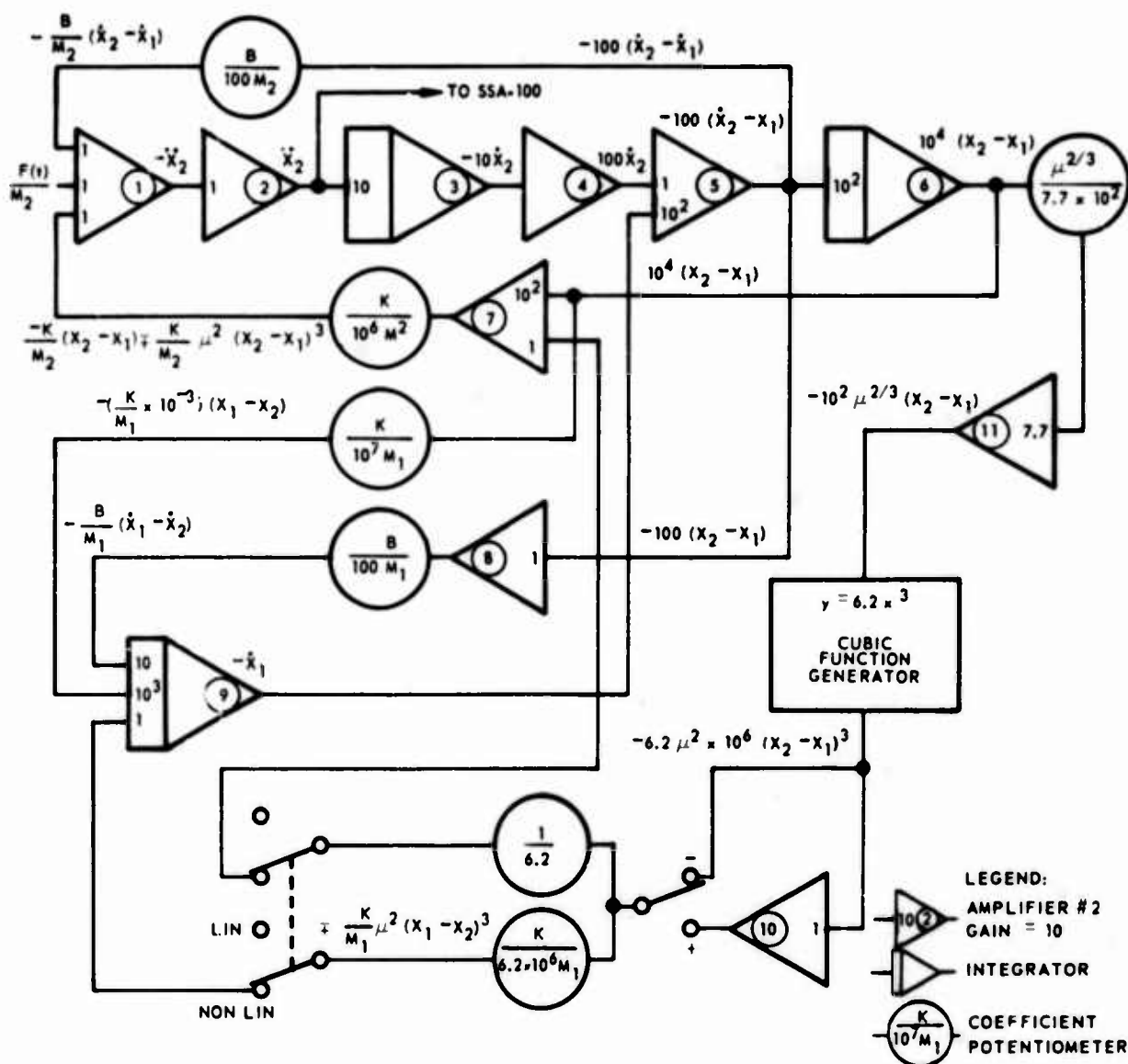
Fig. 4. Simulated load and armature dynamics
