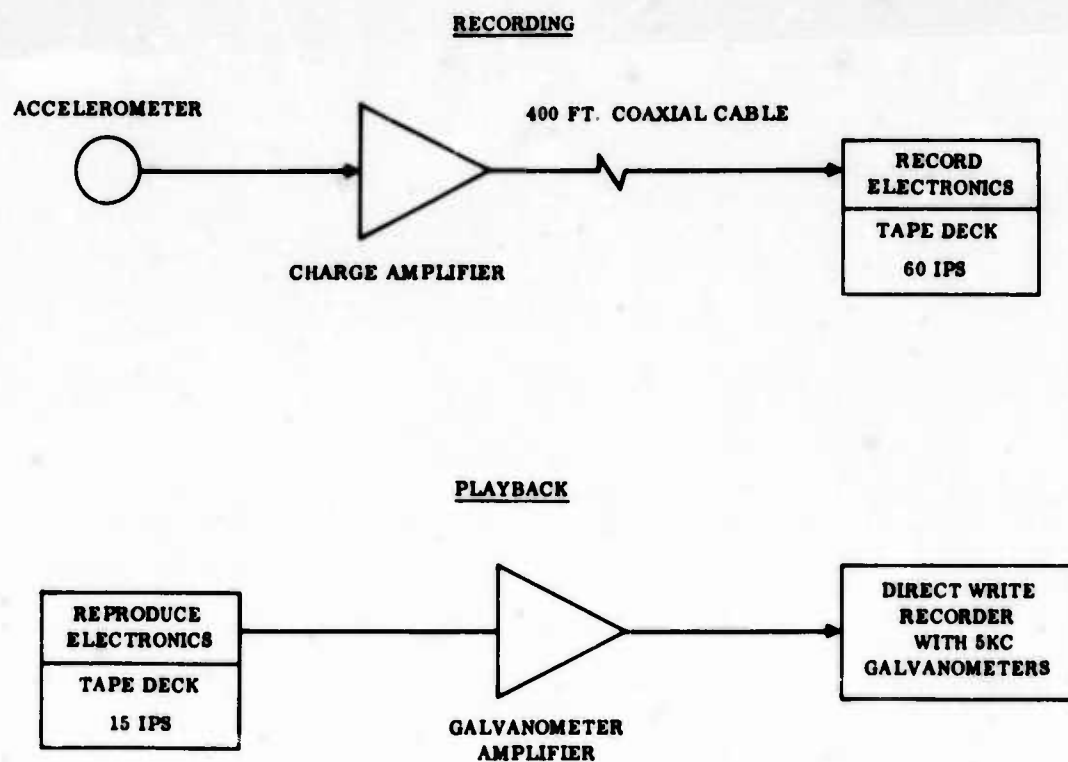
Fig. 7. Instrumentation recording system: block diagram
