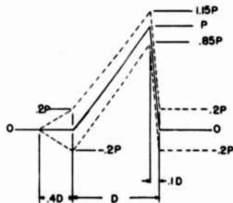
Fig. 6. Sloping terminal-peak sawtooth acceleration pulse with tolerance envelopes. Maximum value is P and duration is D. Peak values of pulse and tolerance envelopes are 0.1D from end of pulse. Velocity change associated with pulse is \Delta V_i = 0.5DP (D expressed in seconds and P as acceleration). \Delta V_m (measured) must be equal to \Delta V_i \pm 10 percent.
