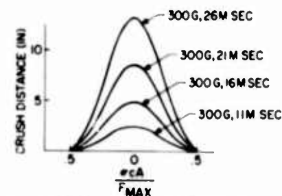
b) ANCHOR PROGRAMMER HONEYCOMB PROFILES
