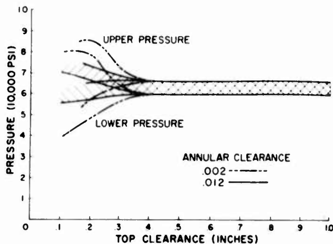
Fig. 11. Variation of peak pressures with top clearance
