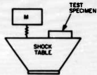
Fig. A3. Large resonant mass on shock table
