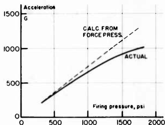
Fig. 25. Acceleration vs firing pressure
