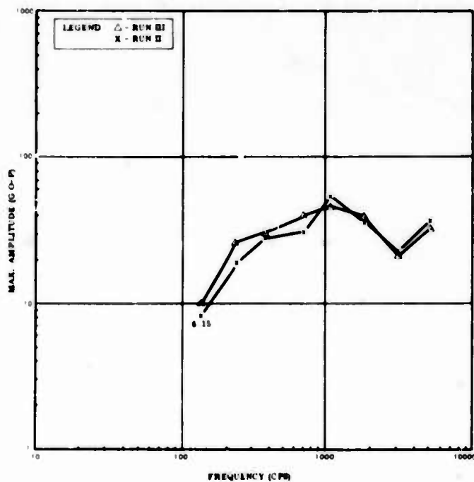
SHOCK RESPONSE SPECTRUM OF MEAS NO 21 (AT PAYLOAD LATCH RADIAL STA 128 - 129°)
