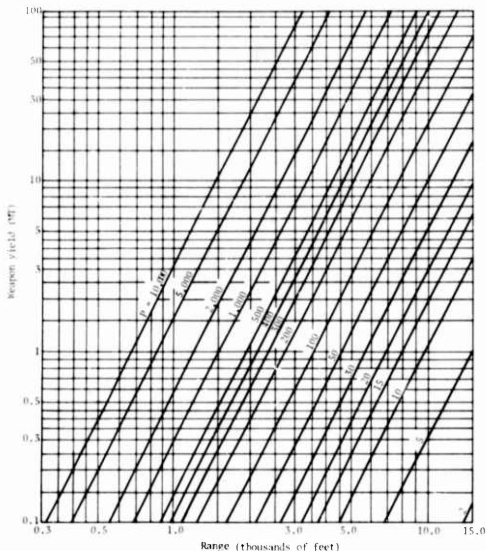
Fig. 1. Peak overpressure at ground surface vs range for various surface-burst weapon yields at sea level
