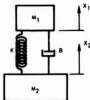
Fig. 2. Simple two-mass system
