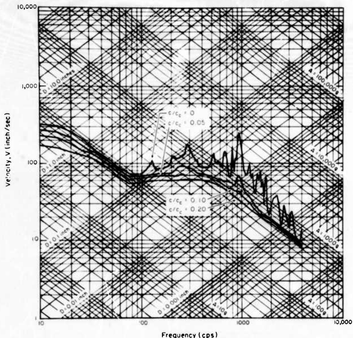
Fig. 10. Damped shock spectra for record 4
