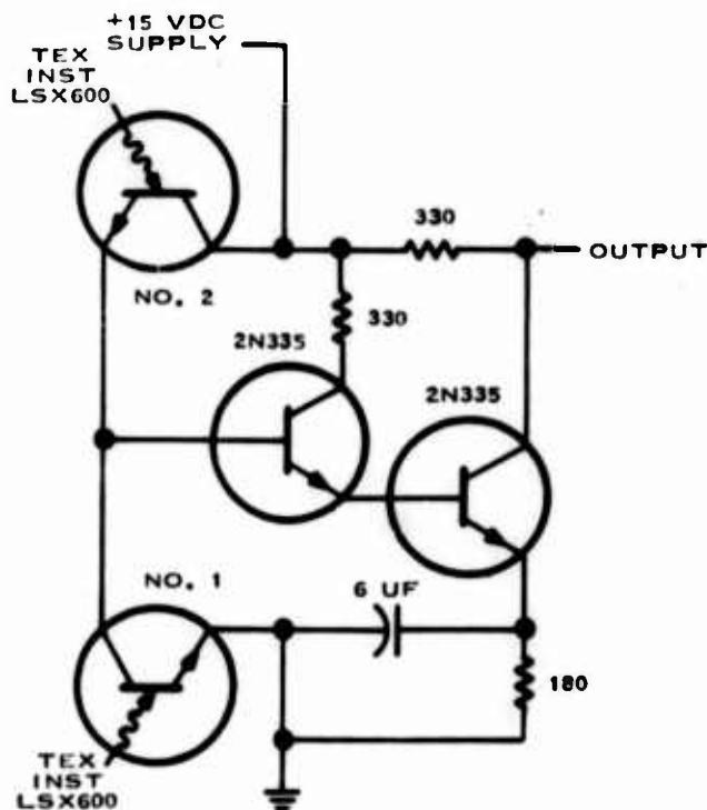
Fig. 6. Light sensor circuit, schematic diagram
