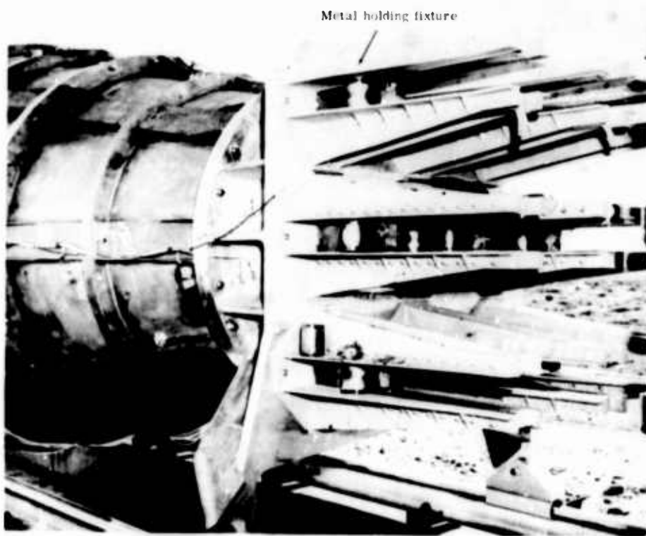
Fig. 14. Metal holding fixtures
