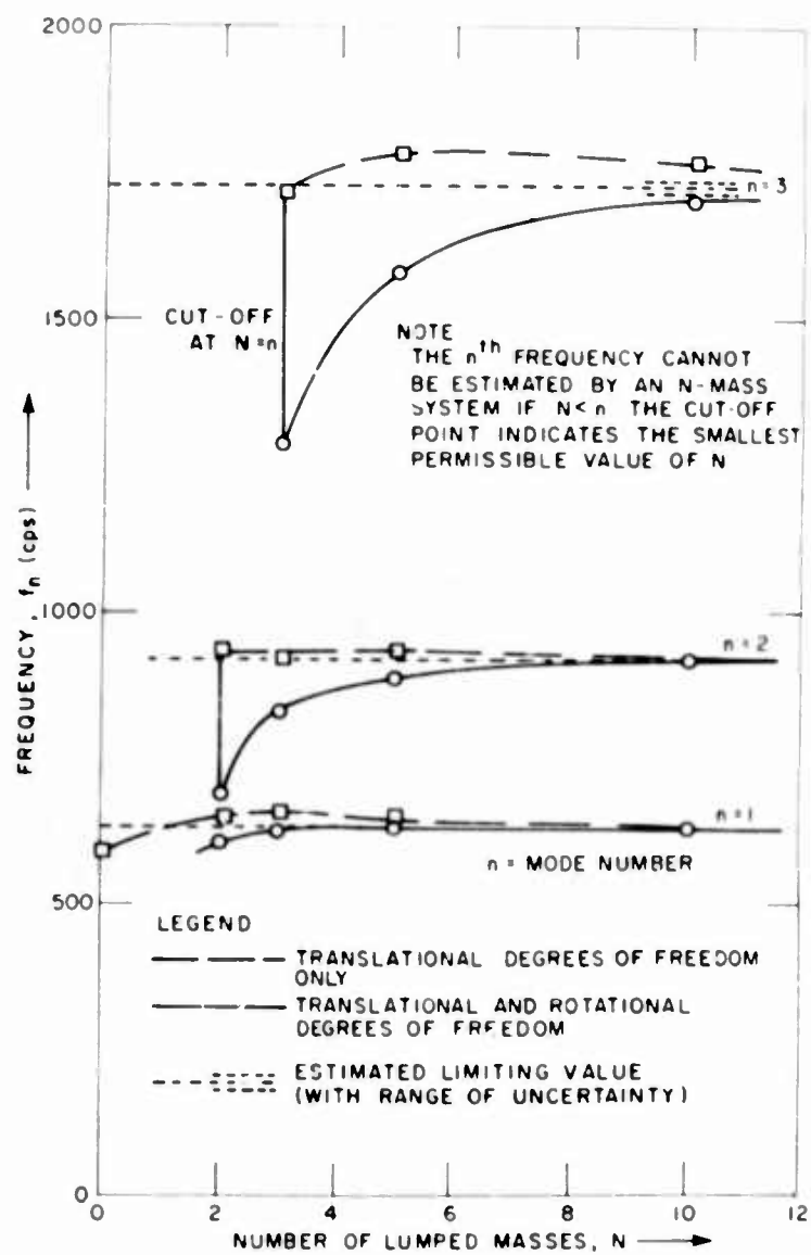
Fig. 10. Frequency vs number of masses
