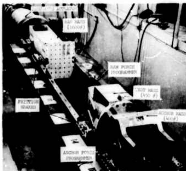
Fig. 3. Setup for shock test -- longitudinal axis
