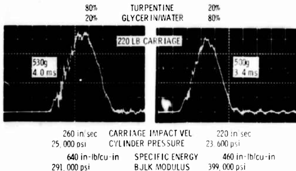
Fig. 22. Pulses obtainable with constant volume variable rate liquid spring
