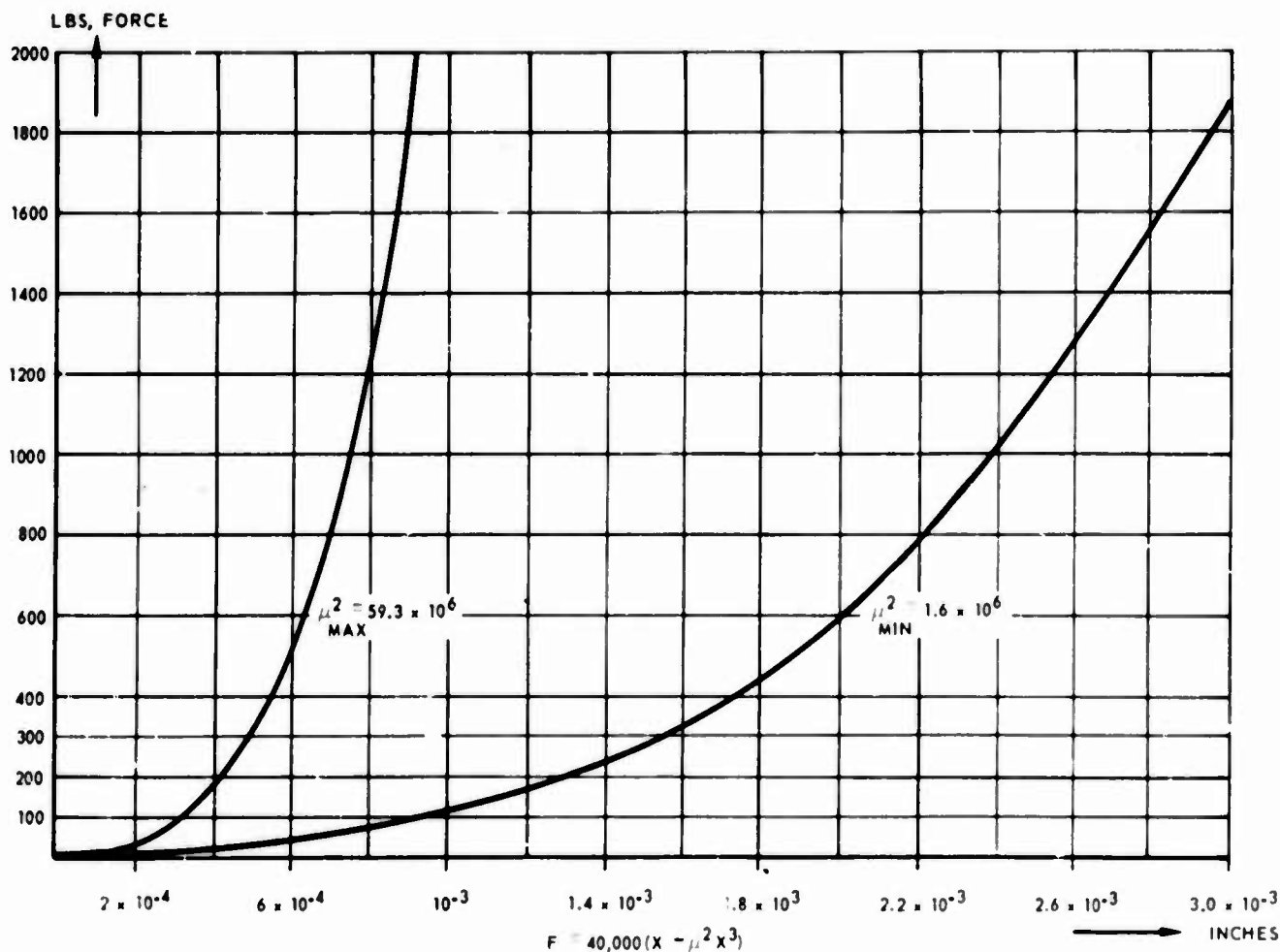
Fig. 5. Nonlinear spring force vs displacement
