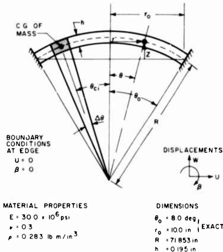
Fig. 9. Spherical cap model used for analytical study
