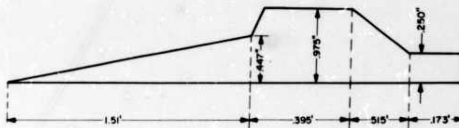
Fig. 16. Cross section of shear metal configuration
