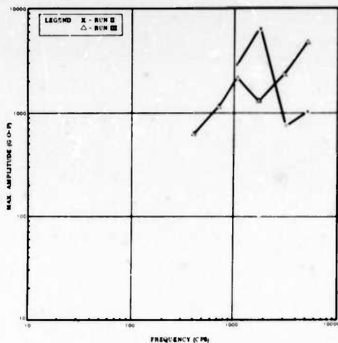
SHOCK RESPONSE SPECTRUM OF MEAS NO 27A (ELECTRICAL STAGING DISCONNECT MOUNT Z AXIS STA 406)
