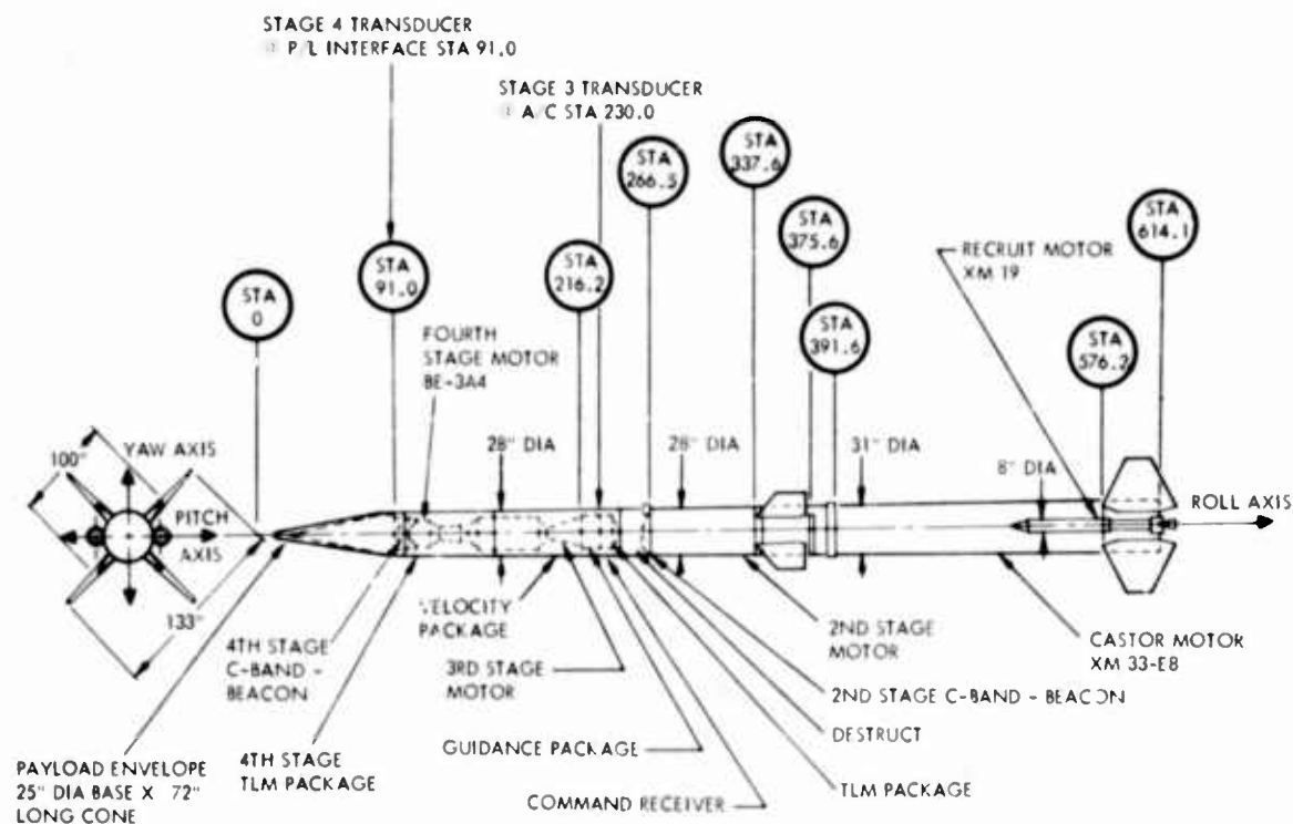
Fig. 1. Configuration of ATHENA vehicle
