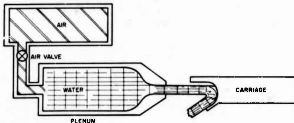
Fig. 1. Schematic of water jet catapult system
