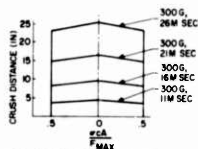
a) RAM PROGRAMMER HONEYCOMB PROFILES
