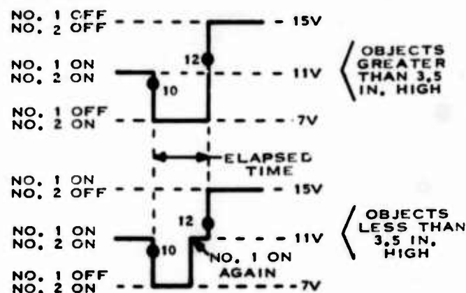
Fig. 7. Theoretical light sensor circuit output pulse
