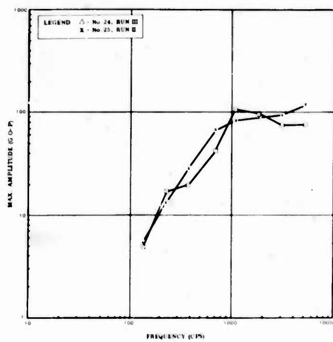
SHOCK RESPONSE SPECTRUM OF MEAS NO 24 & 25 (A/P SEQUENCE TIMER BASE Z AXIS MEAS NO 24 RADIAL MEAS NO 25)
