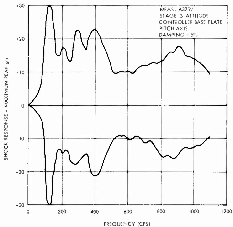
Fig. 13. Shock response spectrum, maximum envelope A-325V
