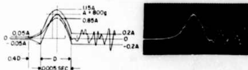
Fig. 20. Nominal 800-g 0.5-ms unfiltered pulse; total impact weight 240 lb; \Delta V_m = 7.8 fps; \Delta V_i = 8.2 fps
