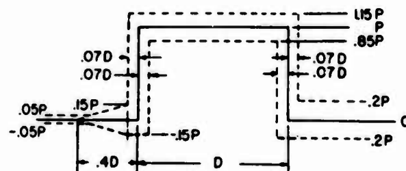
Fig. 7. Rectangular acceleration pulse with tolerance envelopes. Maximum value is P and duration is D. Velocity change associated with pulse is \Delta V_i = DP (D expressed in seconds and P as acceleration).
