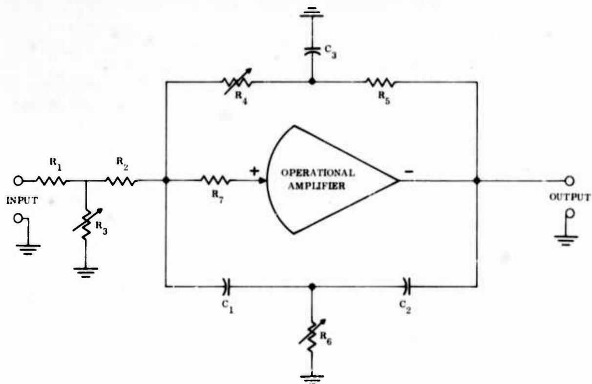
Fig. 9. Schematic of typical simulated system
