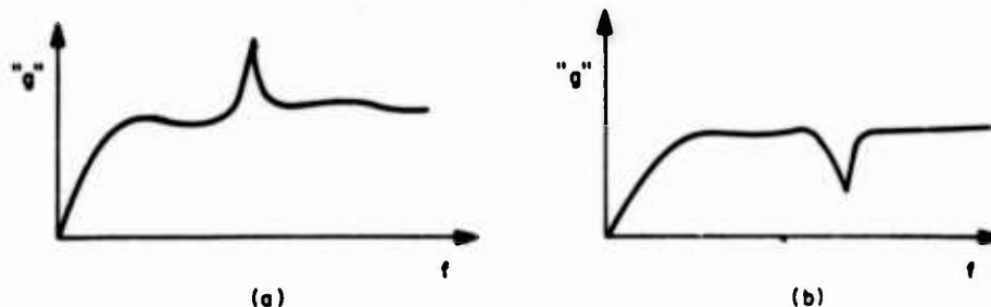
Fig. A-1. Peaks and notches in shock spectra
