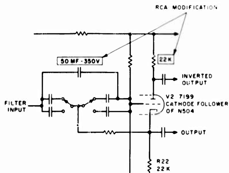
Fig. 5. Schematic diagram of modification to N504 amplifier
