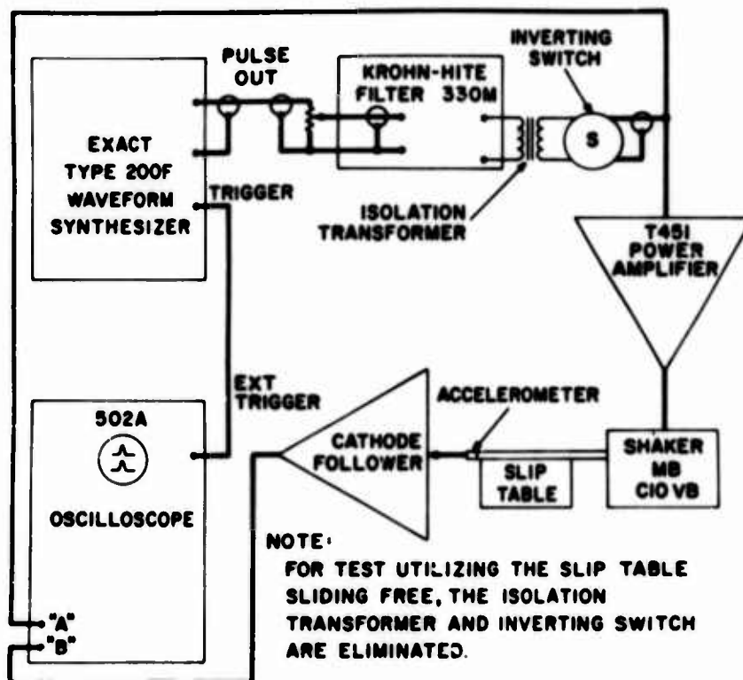
Fig. 7. Transformer isolation test setup
