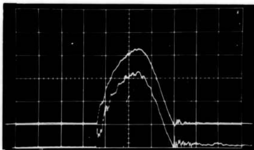
Fig. 8. Pressure-time pulse
