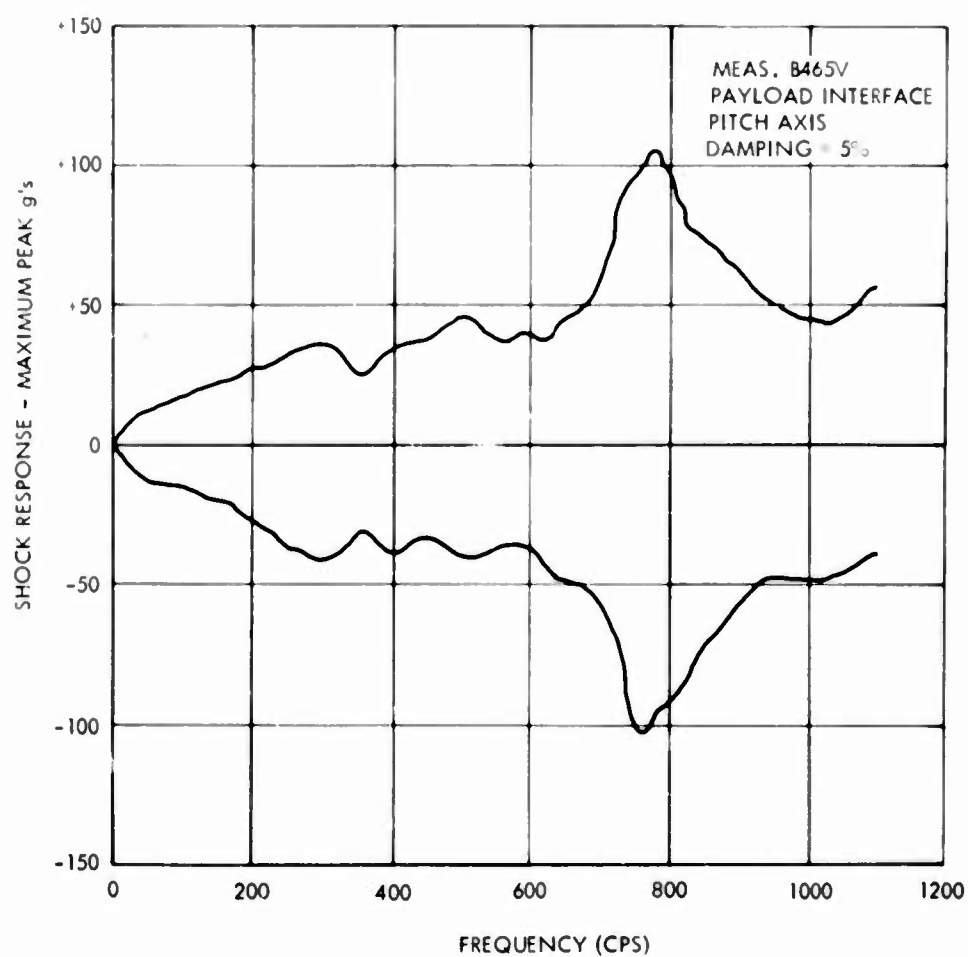
Fig. 10. Shock response spectrum, maximum envelope B-465V
