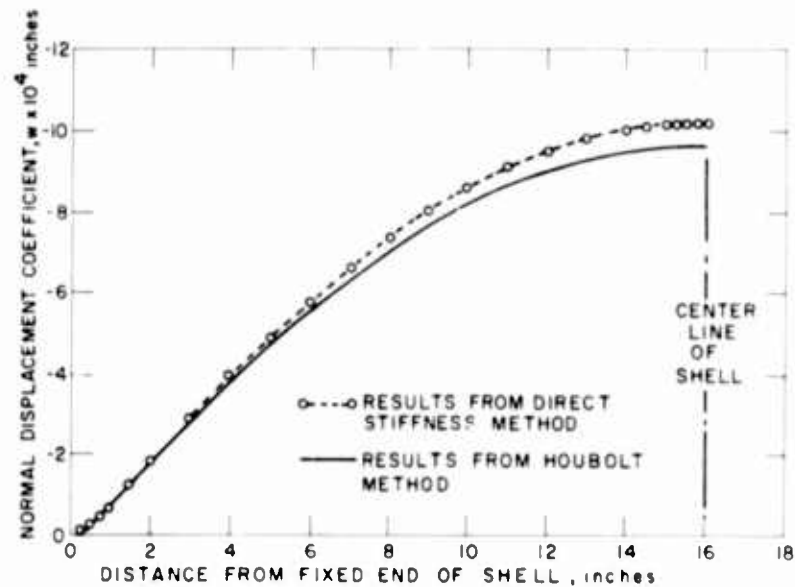
Fig. 19. Comparison of static analyses
