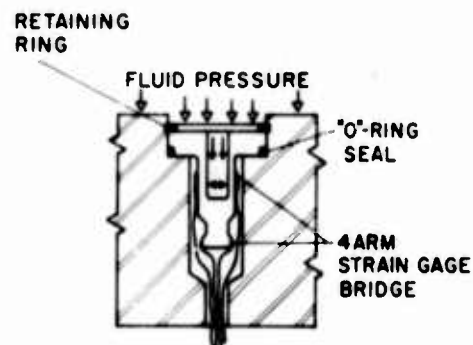
Fig. 2. Pressure gage
