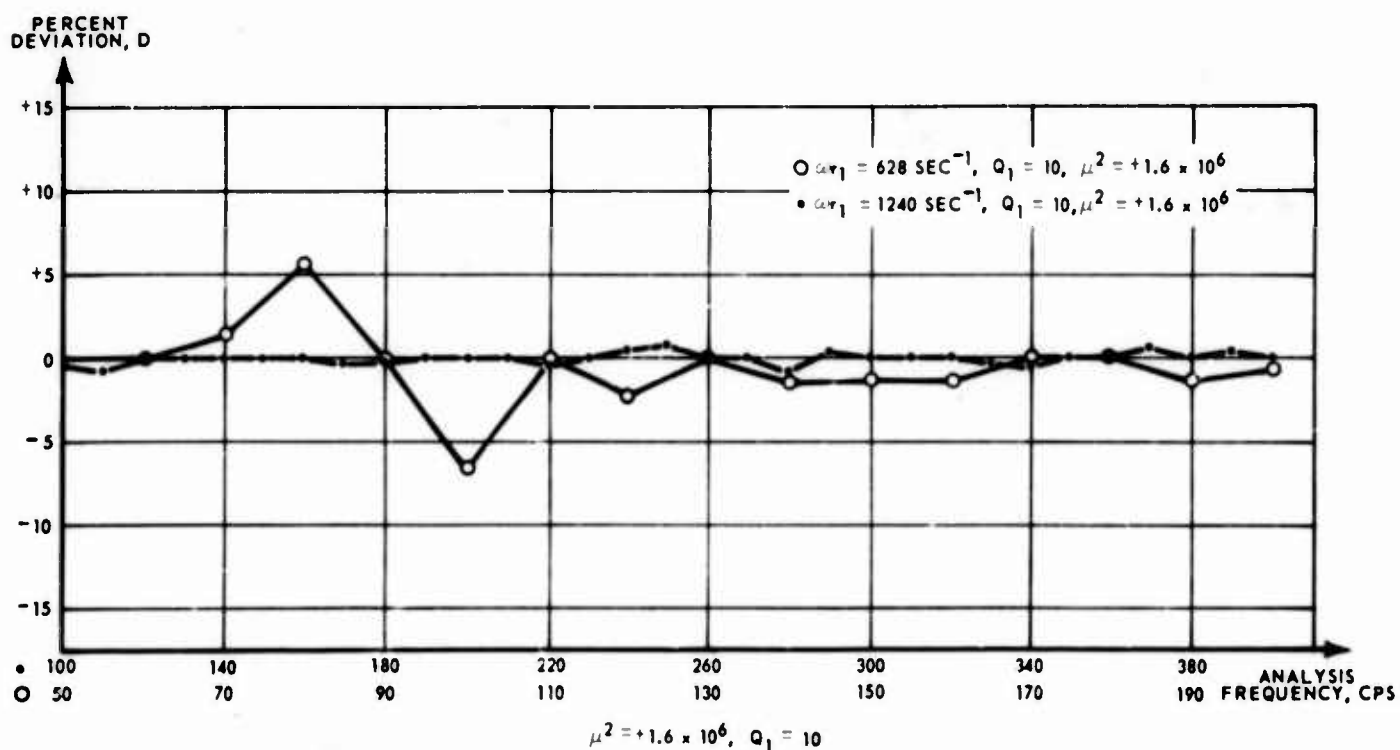
Fig. 8. Deviations in shock spectra due to \omega_{r1}
