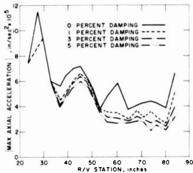
Fig. 27. Absolute max acceleration vs station axial model
