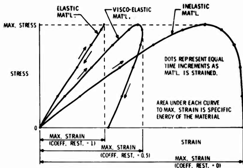
Fig. 12. Theoretical dynamic stress-strain curves of various materials for half-sine pulse generation
