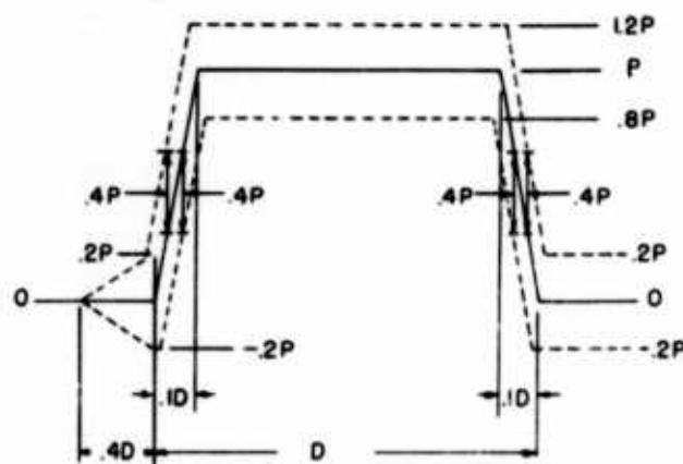
Fig. 8. Trapezoidal acceleration pulse with tolerance envelopes. Maximum value is P and duration is D . Velocity change associated with pulse is \Delta V_i = 0.9DP ( D expressed in seconds and P as acceleration).
