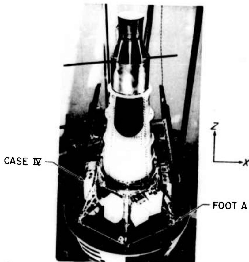
Fig. 4. Ranger pyrotechnic test configuration
