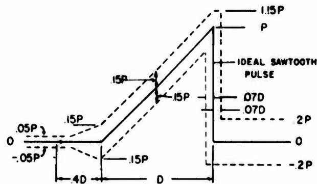
Fig. 5. Terminal-peak sawtooth acceleration pulse with tolerance envelopes. Maximum value is P and duration is D. Velocity change associated with pulse is \Delta V_i = 0.5DP (D expressed in seconds and P as acceleration). \Delta V_m (measured) must be equal to \Delta V_i \pm 10 percent.
