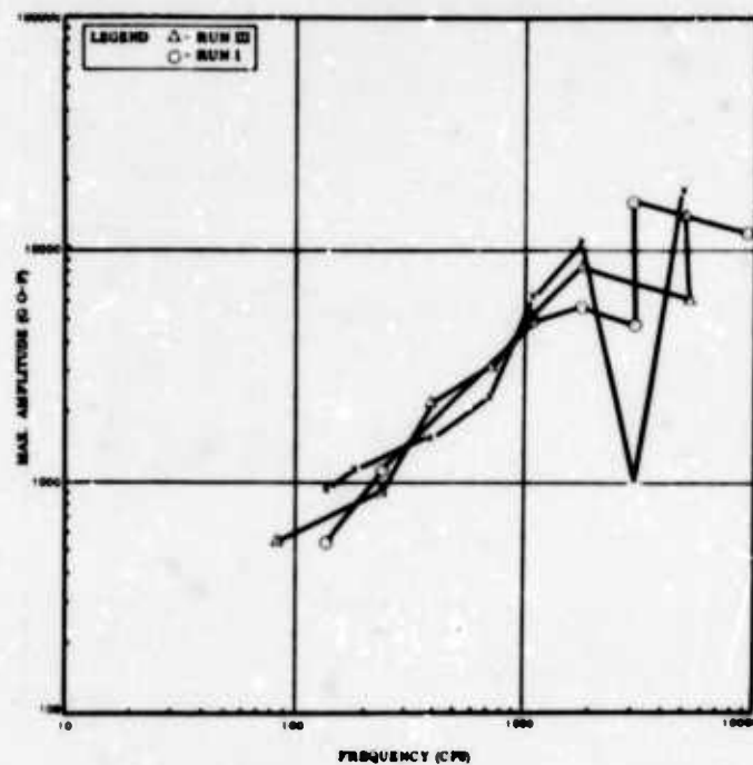
SHOCK RESPONSE SPECTRUM OF MEAS NO 26 (AFT SEAL PLATE, Z AXIS STA 406)
