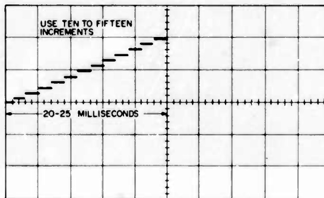
Fig. A-1. Exact program for half-sine pulse
