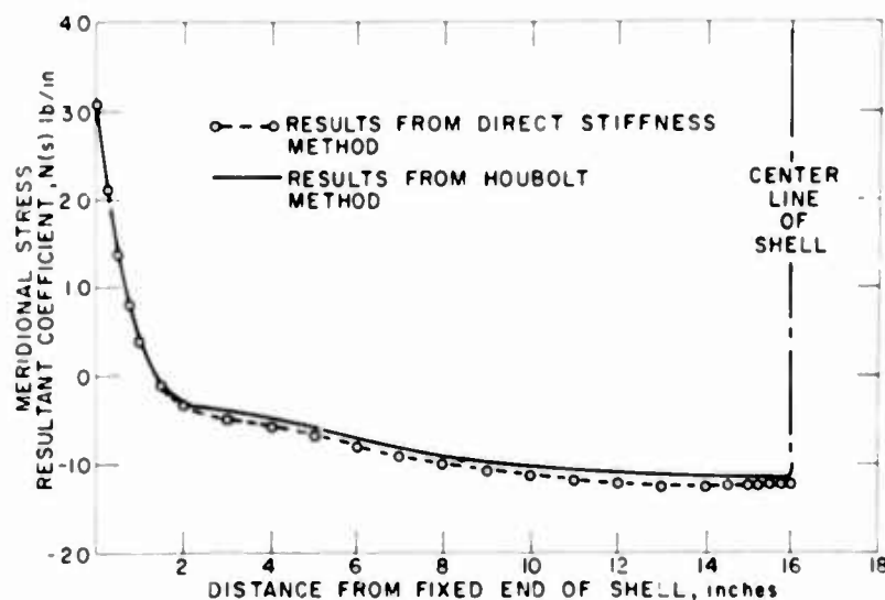
Fig. 21. Comparison of static analyses
