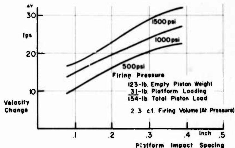
Fig. 26. Impact load velocity vs impact spacing
