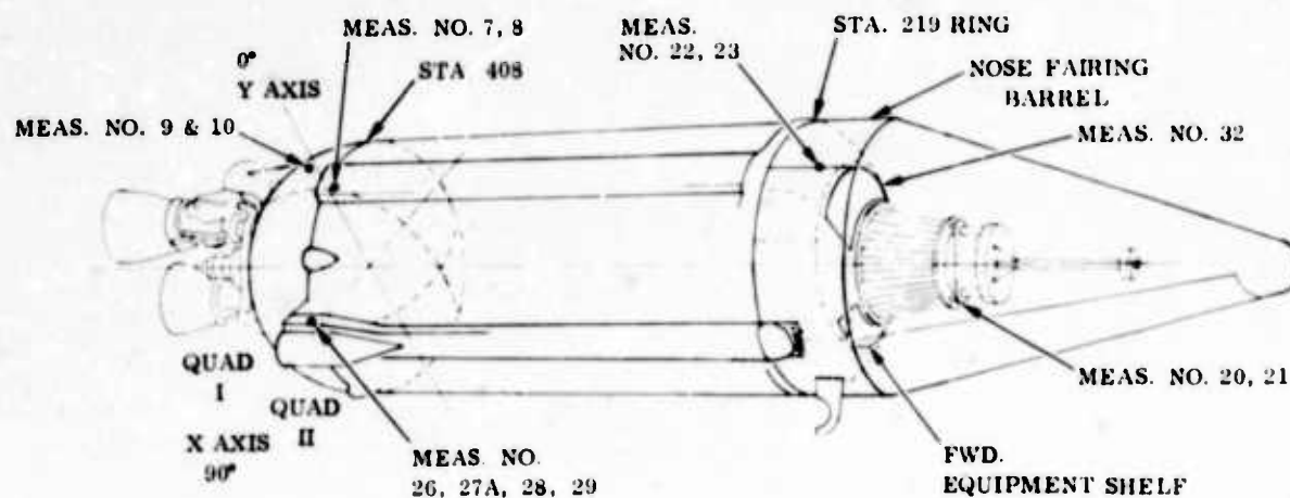
Fig. 4. Accelerometer locations for insulation panel jettison test
