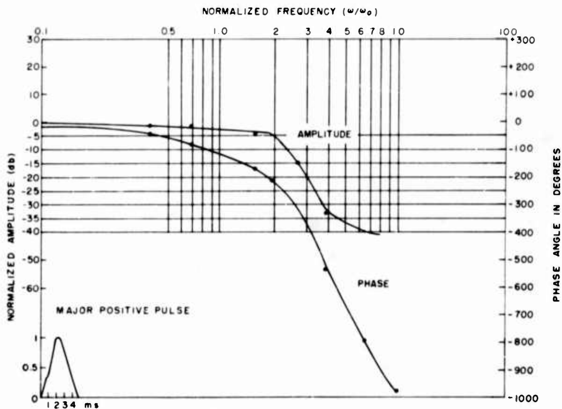
Fig. 8. Typical Bode diagram of 123-JAN shock machine pulse
