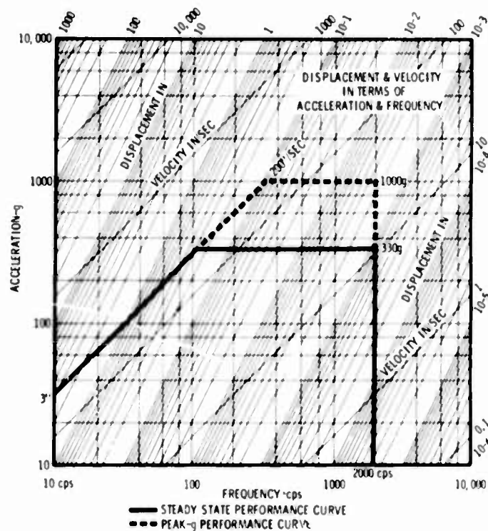
Fig. 10. Performance curve of shaker capable of simulating pyrotechnic events. Shaker would be capable of generating energy necessary for simulating shock spectrum of 3000 response g.
