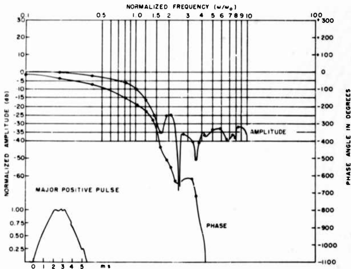
Fig. 12. Typical Bode diagram of JAN-S-44 shock machine pulse
