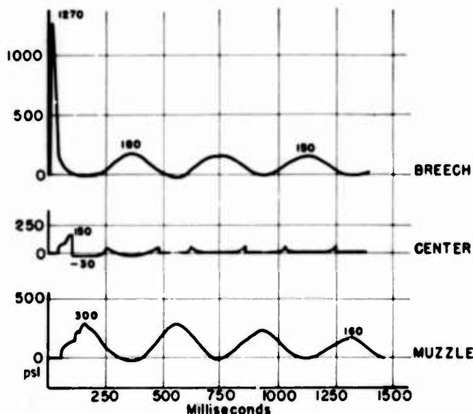
Fig. 28. Barrel air pressure vs time, 154-lb load
