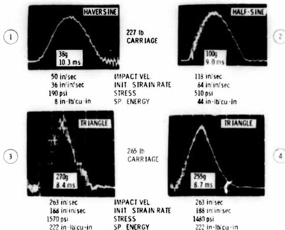
Fig. 3. Pulse conditions generated by typical neoprene rubber spring assembly
