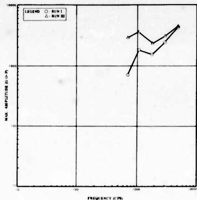
SHOCK RESPONSE SPECTRUM OF MEAS NO 28 (AFT SEAL PLATE NEAR STAGING DISC Y AXIS STA 406)
