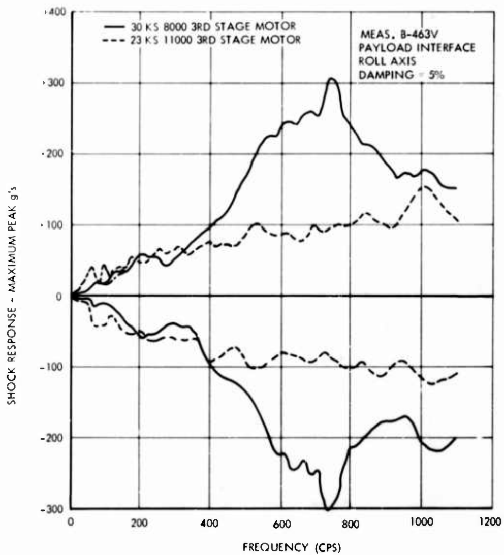
Fig. 14. Shock response spectra, third stage ignition
