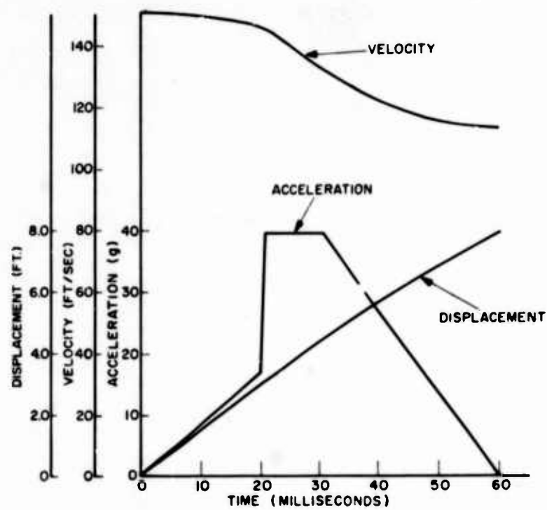
Fig. 8. Moving sled acceleration, velocity, and displacement curves
