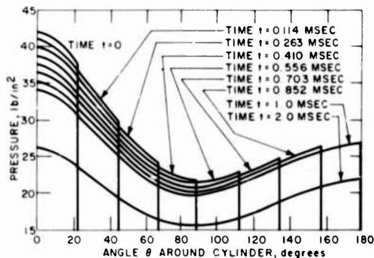
Fig. 3. Pressure distributions around cylinder during engulfment by blast
