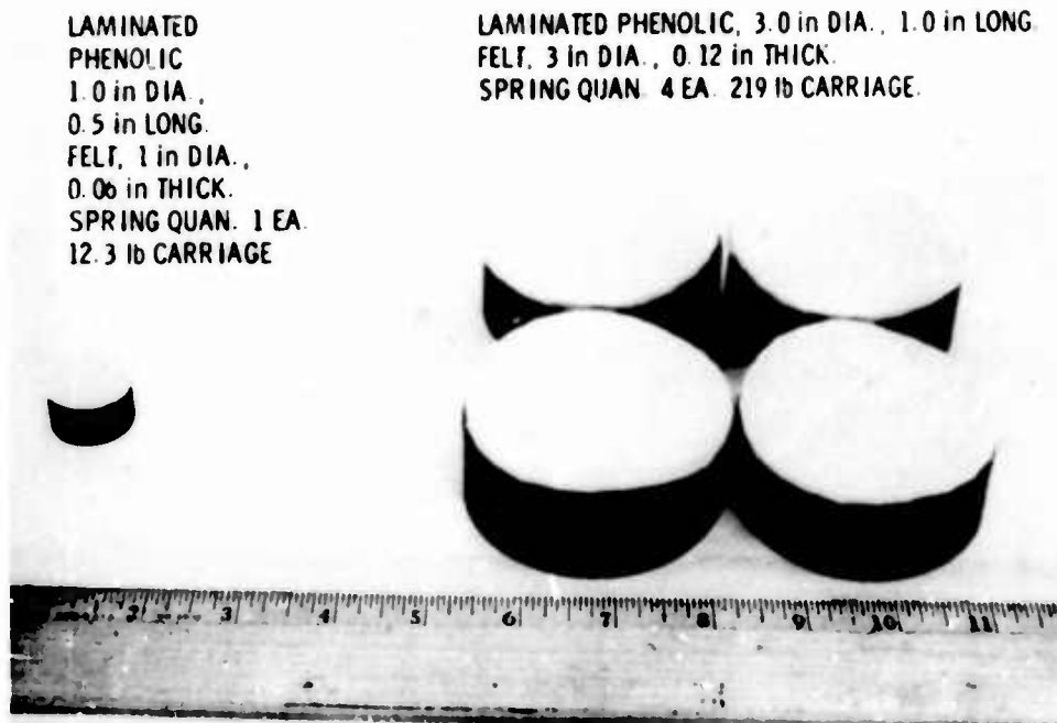
Fig. 13. Two laminated phenolic spring setups
