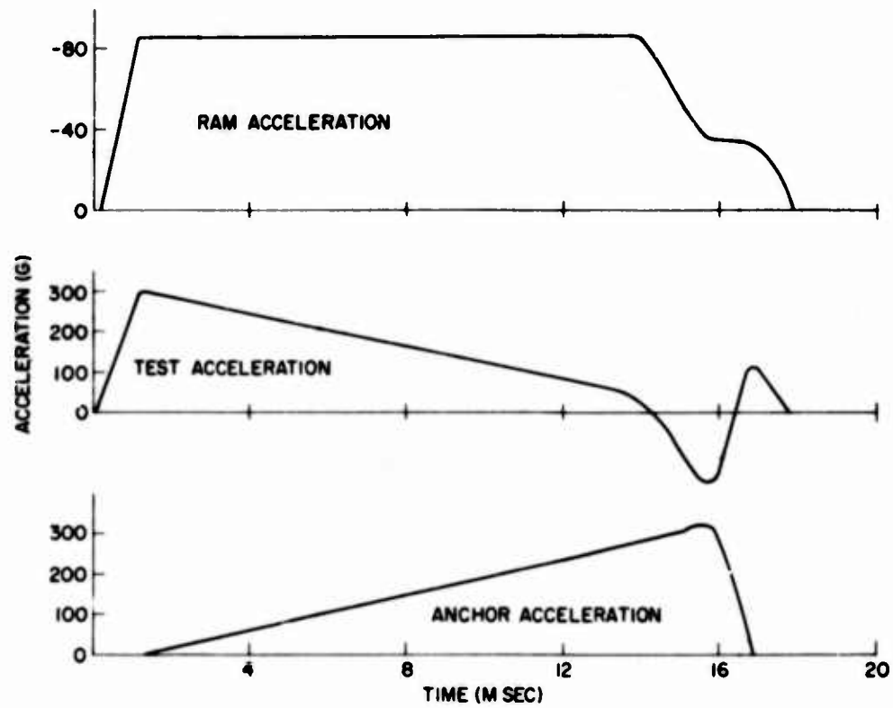
Fig. 14. Computed acceleration results allowing for restitution -- ram impact velocity reduced to 110 fps
