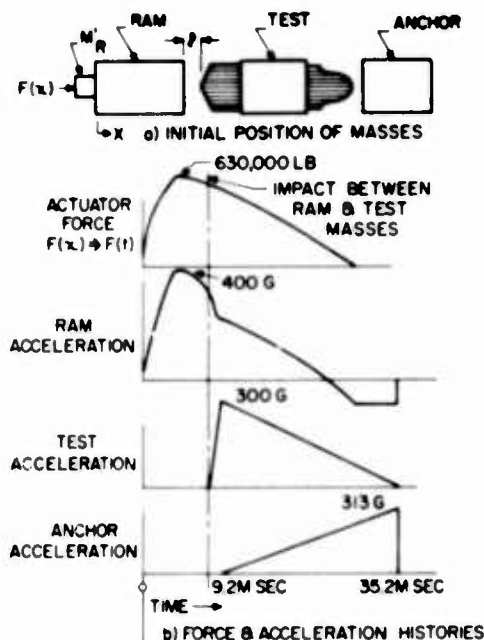
Fig. 10. Setup and motion histories calculated for impulsive impact
