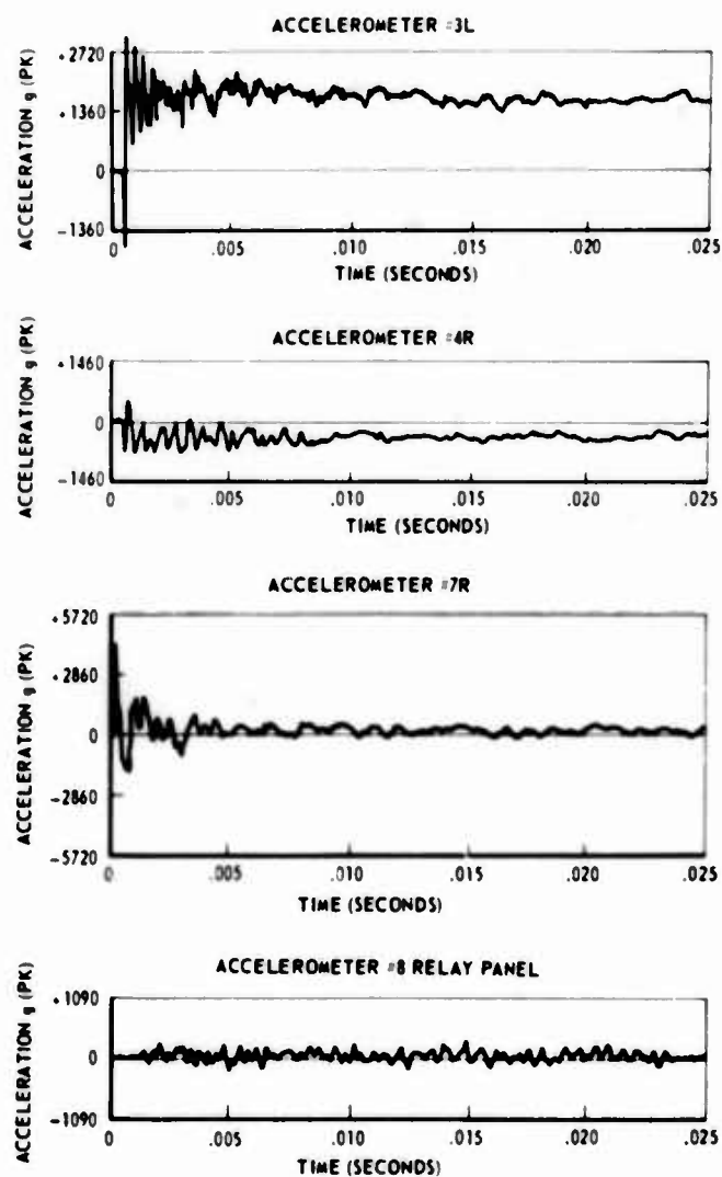
Fig. 6. Shaped charge firing at Z-13 -- test 1
