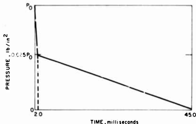
Fig. 1. Idealized pressure pulse
