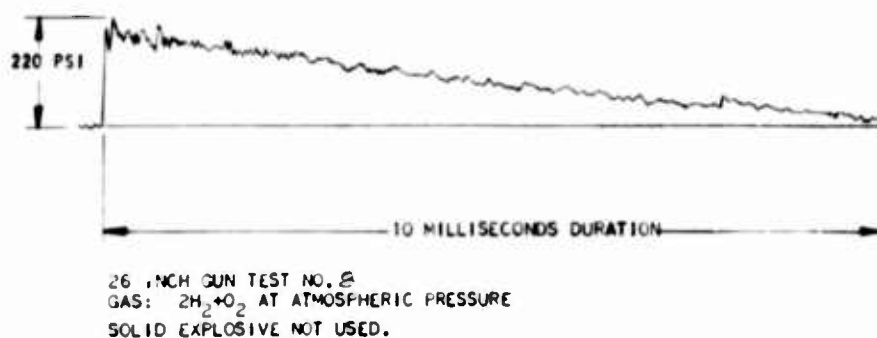
Fig. 13. Typical pressure-time record of explosive gas test in 130-ft gun, solid explosive not used
