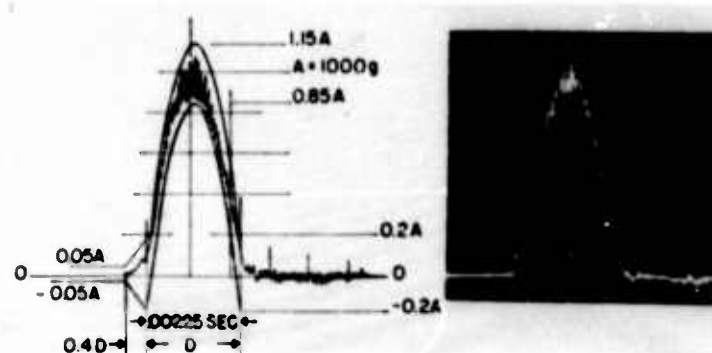
Fig. 21. Nominal 1000-g 2.25-ms unfiltered pulse; total impact weight 91 lb; \Delta V_m = 48.3 fps; \Delta V_i = 46.1 fps
