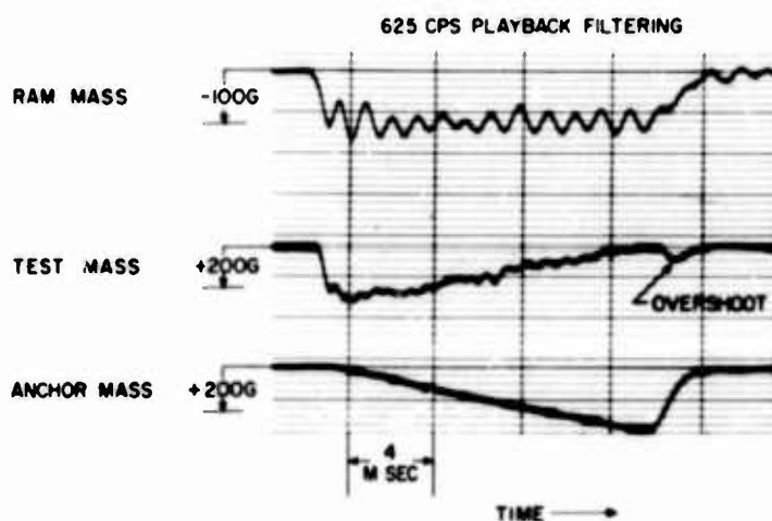
Fig. 5. Acceleration results obtained using setup of Fig. 3
