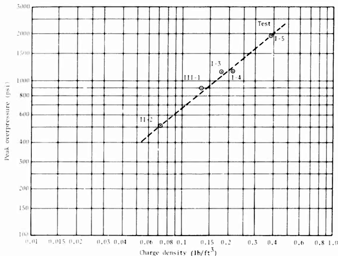
Fig. 12. Peak overpressure vs charge density
