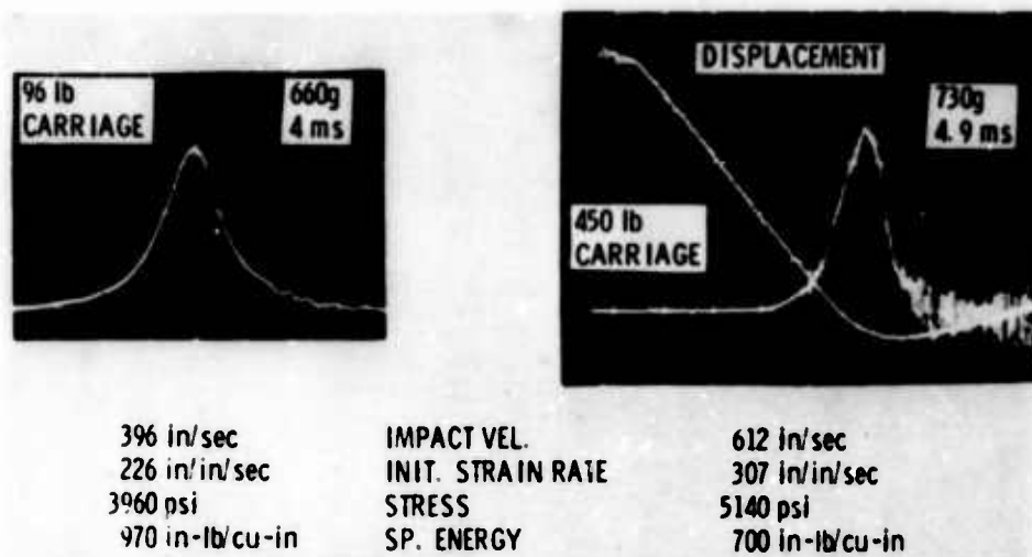
Fig. 4. Parabolic cusps from 30 Durometer A butyl rubber
