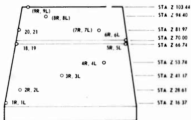
Fig. 5. Accelerometer locations on adapter skin -- test 2
