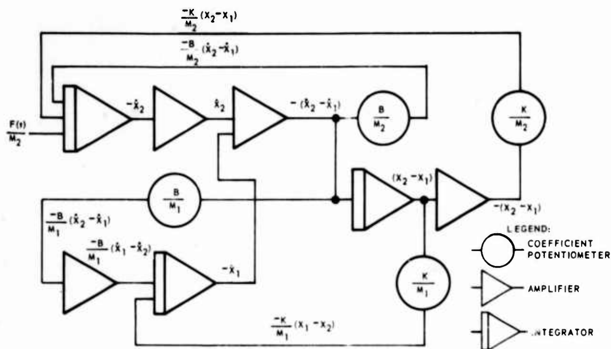
Fig. 3. Analog setup for two-mass system
