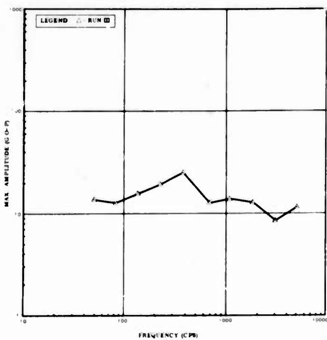
SHOCK RESPONSE SPECTRUM OF MEAS NO 19 (LOCATED INSIDE OF RANGE SAFETY POWER CONTROL BOX NEXT TO RELAY)
