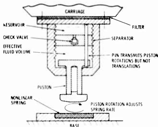
Fig. 15. Commercial variable rate, changing volume, liquid shock spring
