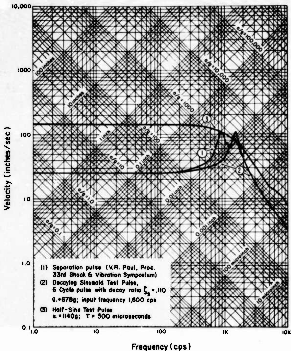
Fig. 6. Separation shock test pulse comparison
