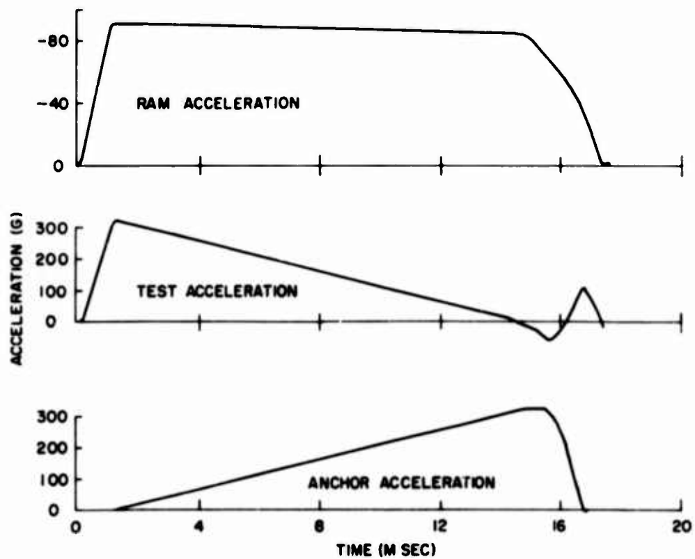
Fig. 17. Computed acceleration results allowing for restitution and rate sensitivity
