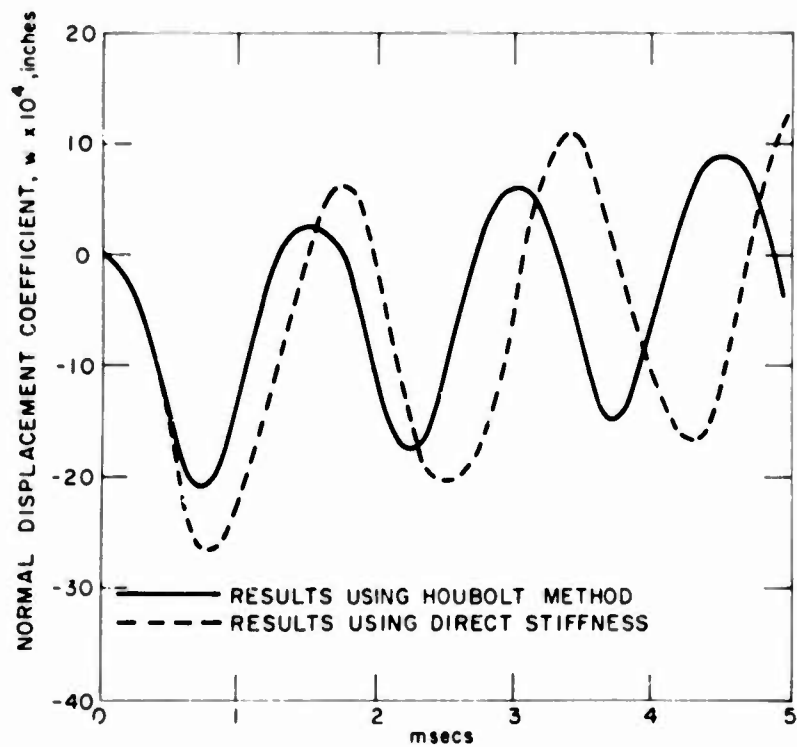
Fig. 23. Comparison of dynamic response at centerline of shell -- normal displacement coefficient W
