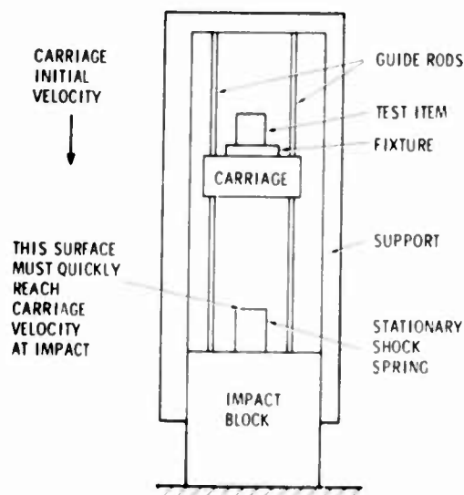
Fig. 2. Impact shock machine
