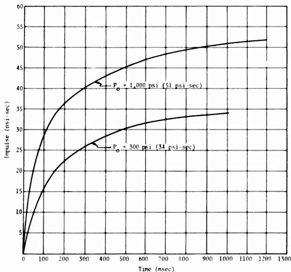
Fig. 5. Total impulse vs time for 300- and 1,000-psi peak overpressures, 1-Mt weapon
