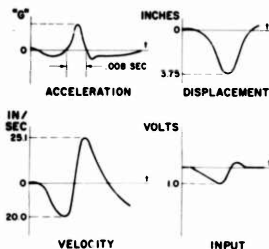
Fig. 2. Typical half-sine pulse on C10VB
