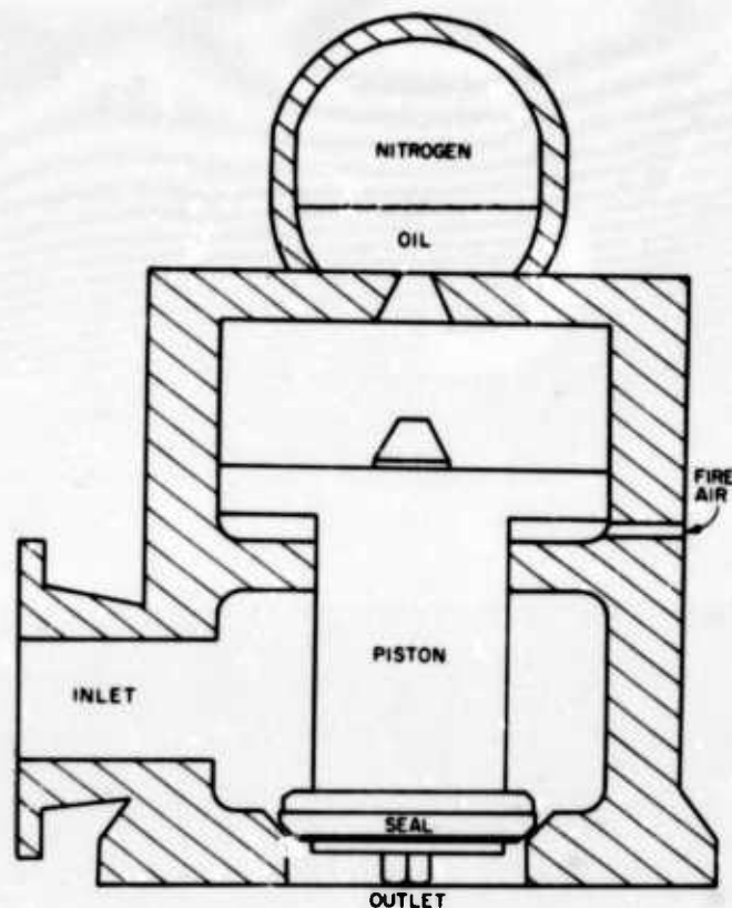
Fig. 2. Firing valve for water jet catapult
