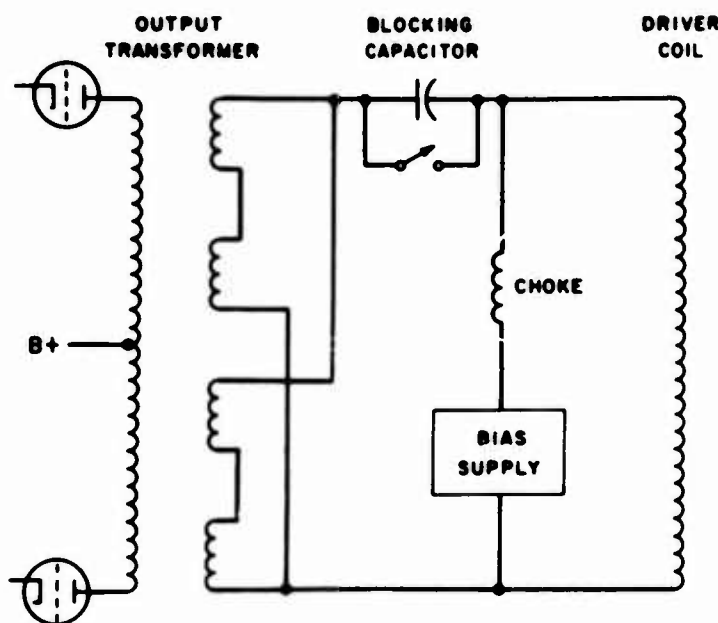
Fig. 1. Typical shaker dc bias
