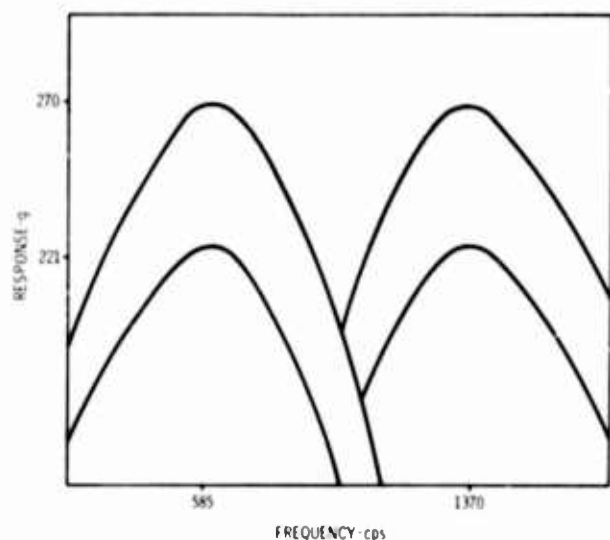
Fig. 5. Resulting spectral deviation based on amplitude time specification of shock pulse. Allowed margins in performing a shock pulse test, 150 \pm 15 g, 1 \pm 0.4 ms, results with scatter in response shown by shaded area in Figs. 4 and 5.
