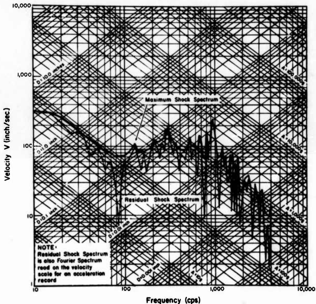
Fig. 9. Maximax and residual spectra for record 4
