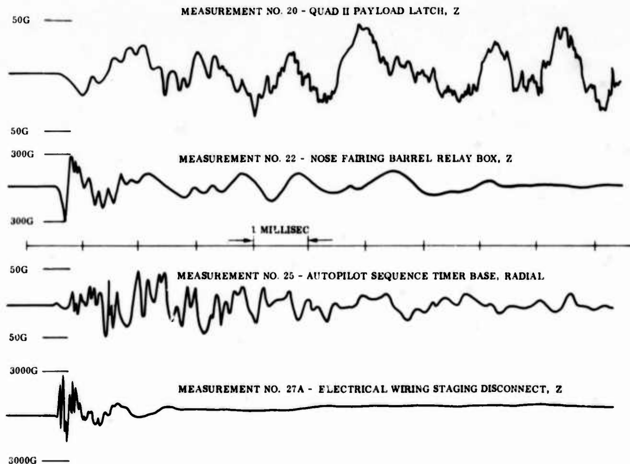
Fig. 10. Selected waveforms from insulation panel separation tests
