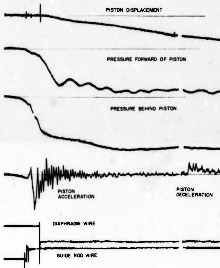
Fig. 8. Typical oscillograph record of water jet catapult test, all values plotted vs time
