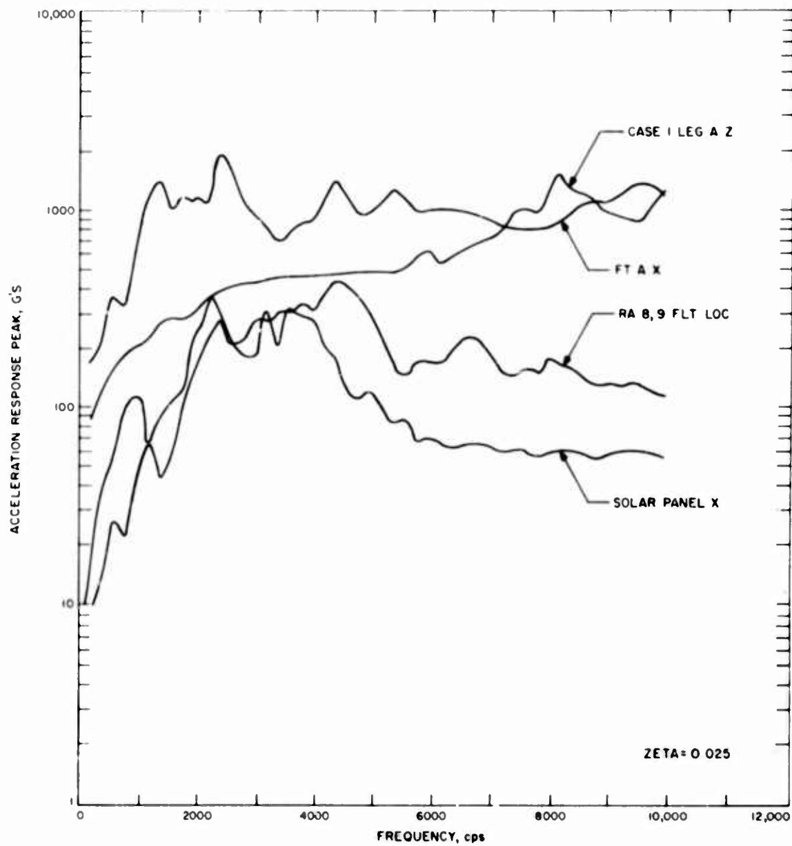
Fig. 17. Shock spectra, Ranger mechanical separation test
