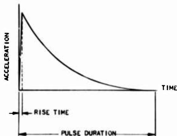
Fig. 1. Idealized blast wave rigid body acceleration-time history
