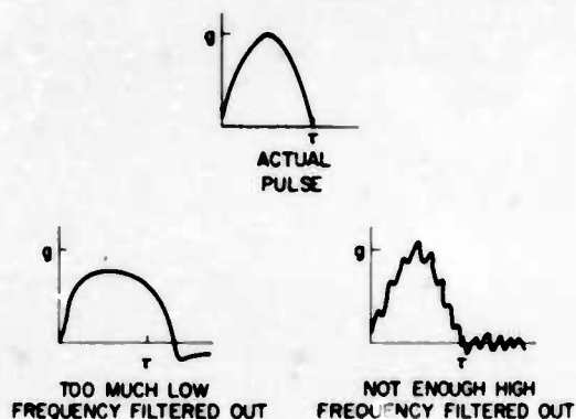
Fig. 1. Effect of filtering on shock pulses
