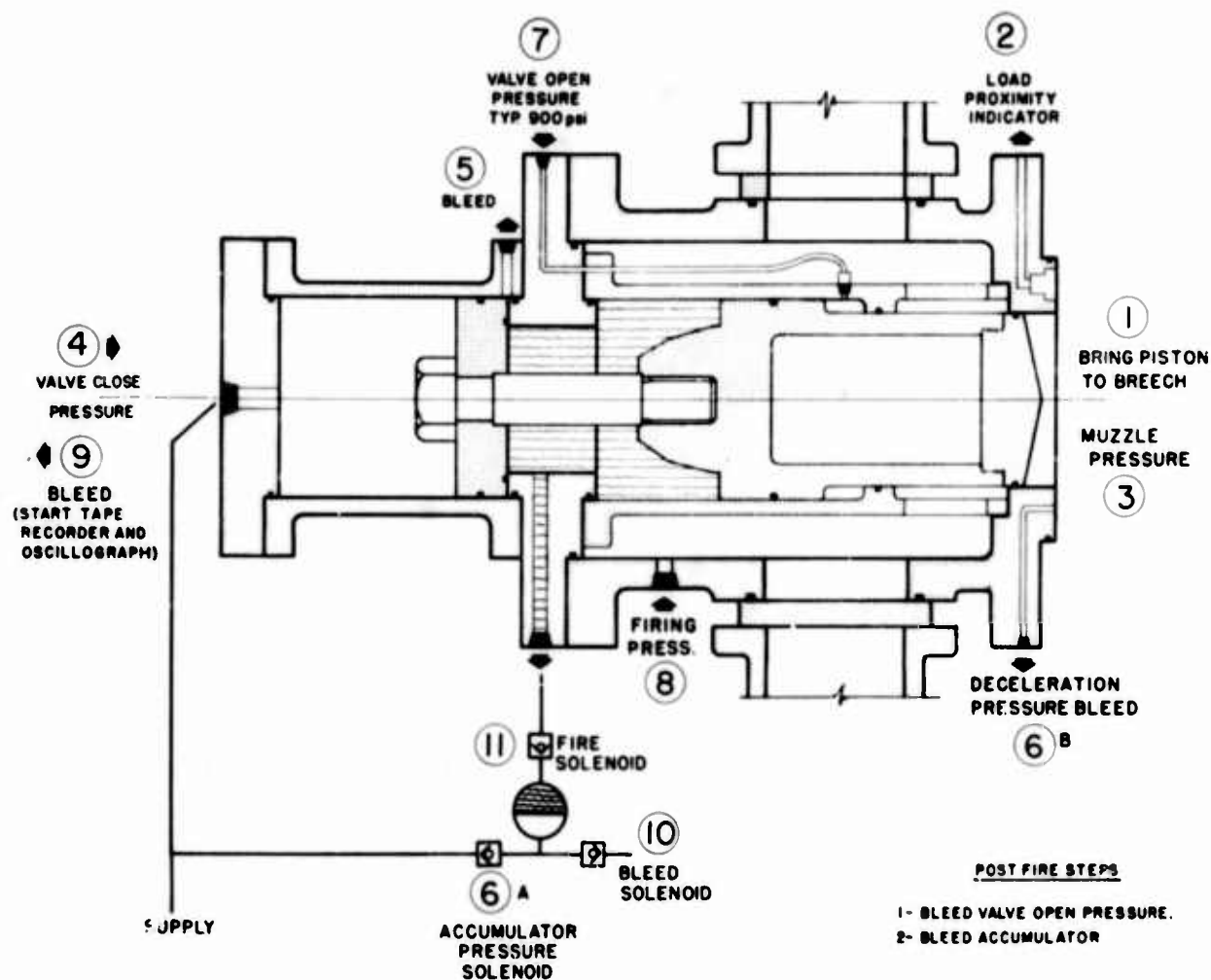
Fig. 18. Fast-opening valve diagram
