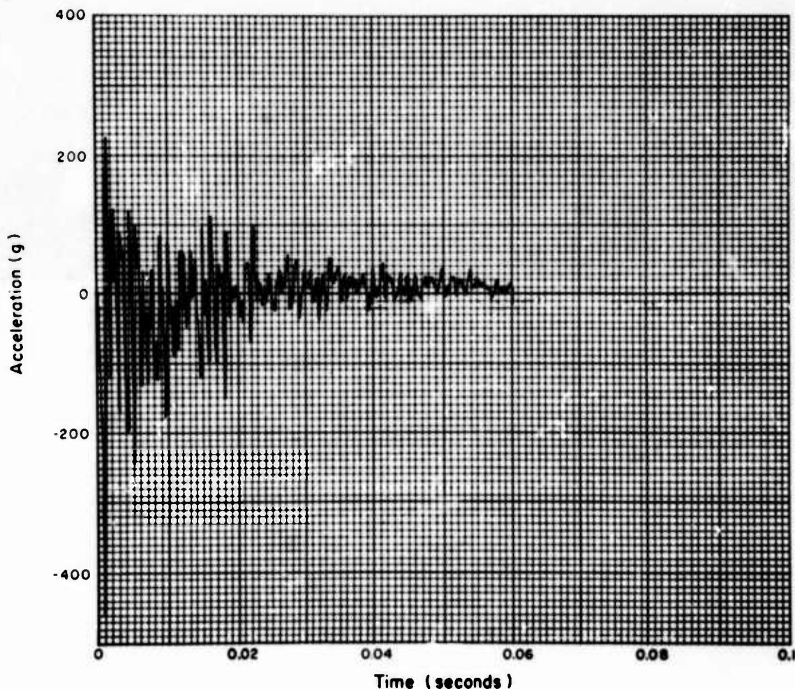
Fig. 7. Shock input time history for record 4
