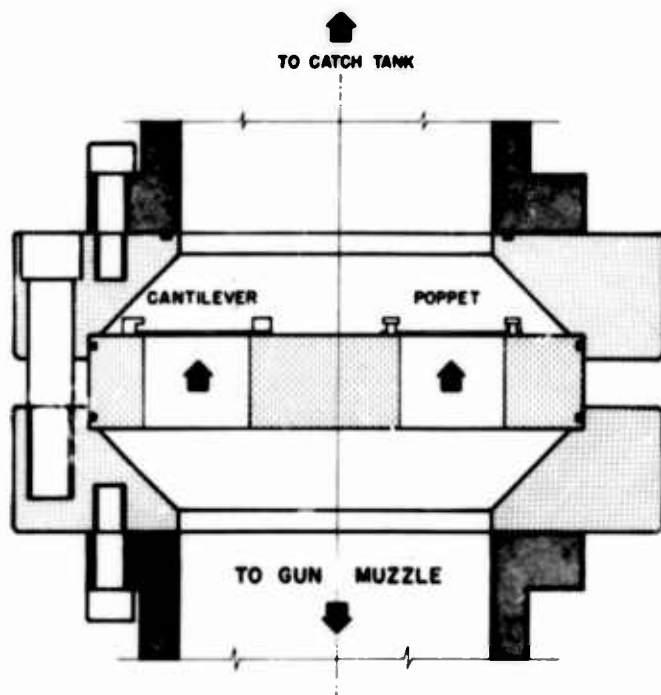
Fig. 19. Muzzle check valve diagram
