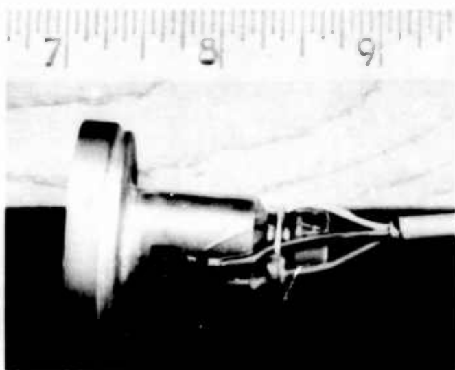
Fig. 3. Pressure gage
