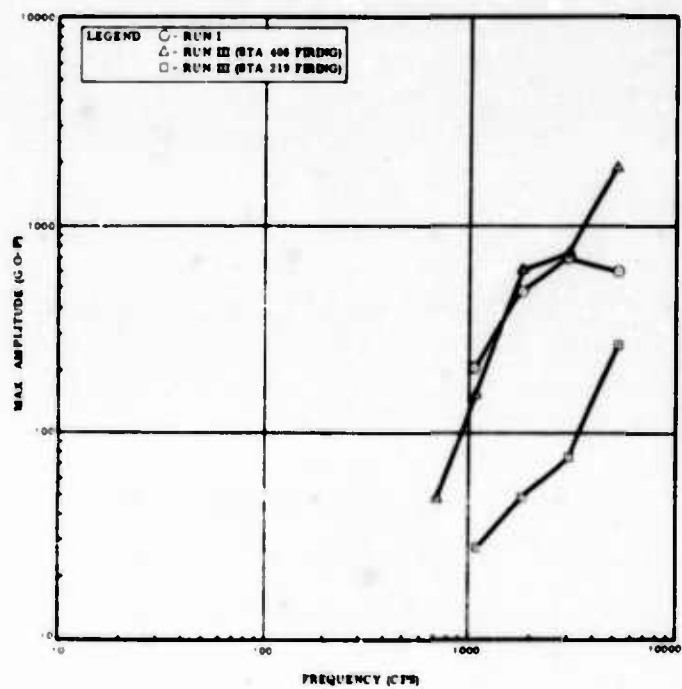
SHOCK RESPONSE SPECTRUM OF MEAS. NO. 9 (DESTRUCT PACKAGE Z AXIS STA 400)
