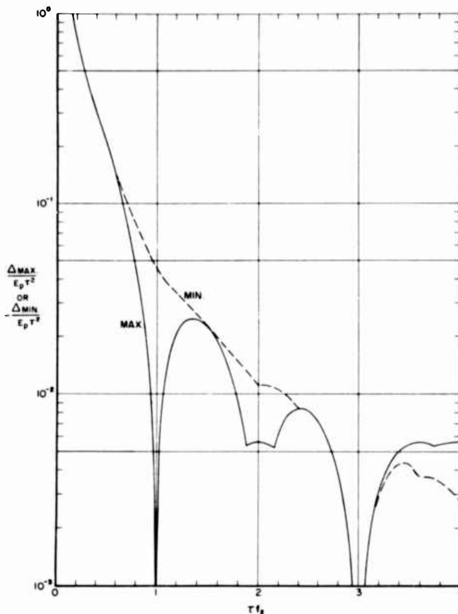
Fig. 7. Proximity spectra of square wave excitation function when \zeta = 0 and \tau f_1 = 3.0
