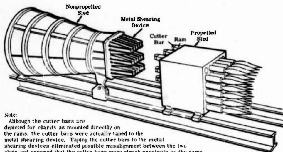
Fig. 2. Propelled and nonpropelled sleds
