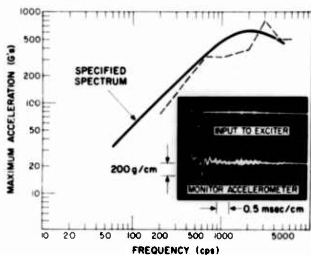
Fig. 3. Shock response spectrum for half-cycle sine input
