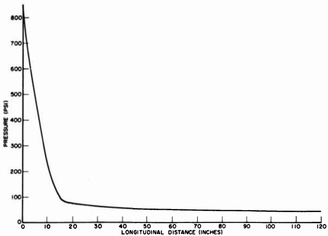
Fig. 5. Normal pressure distribution curve for 119.5 g
