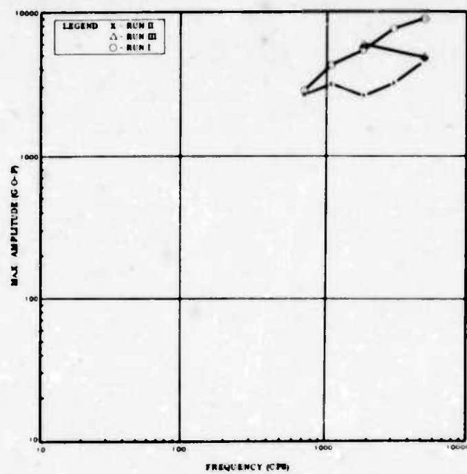
SHOCK RESPONSE SPECTRUM OF MEAS NO 26 (AFT SEAL PLATE, X AXIS STA 406)
