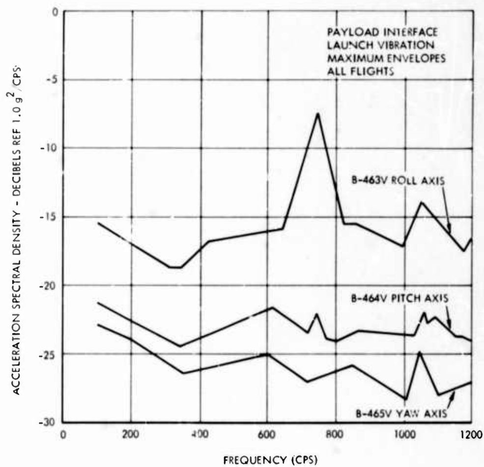
Fig. 5. Acceleration spectral density, Stage 4
