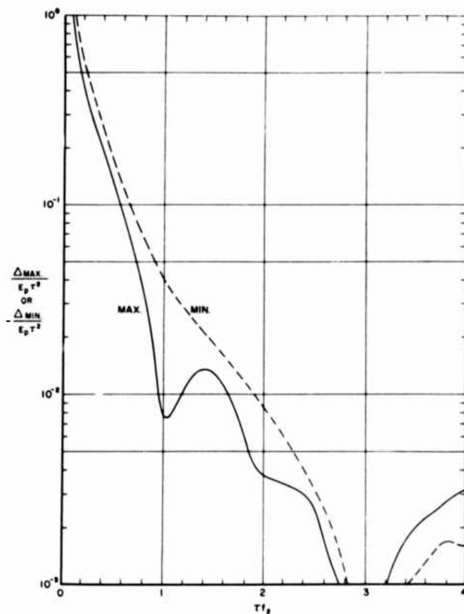
Fig. 9. Proximity spectra of square wave excitation function when \zeta = 0.1 and \tau f_1 = 3.0
