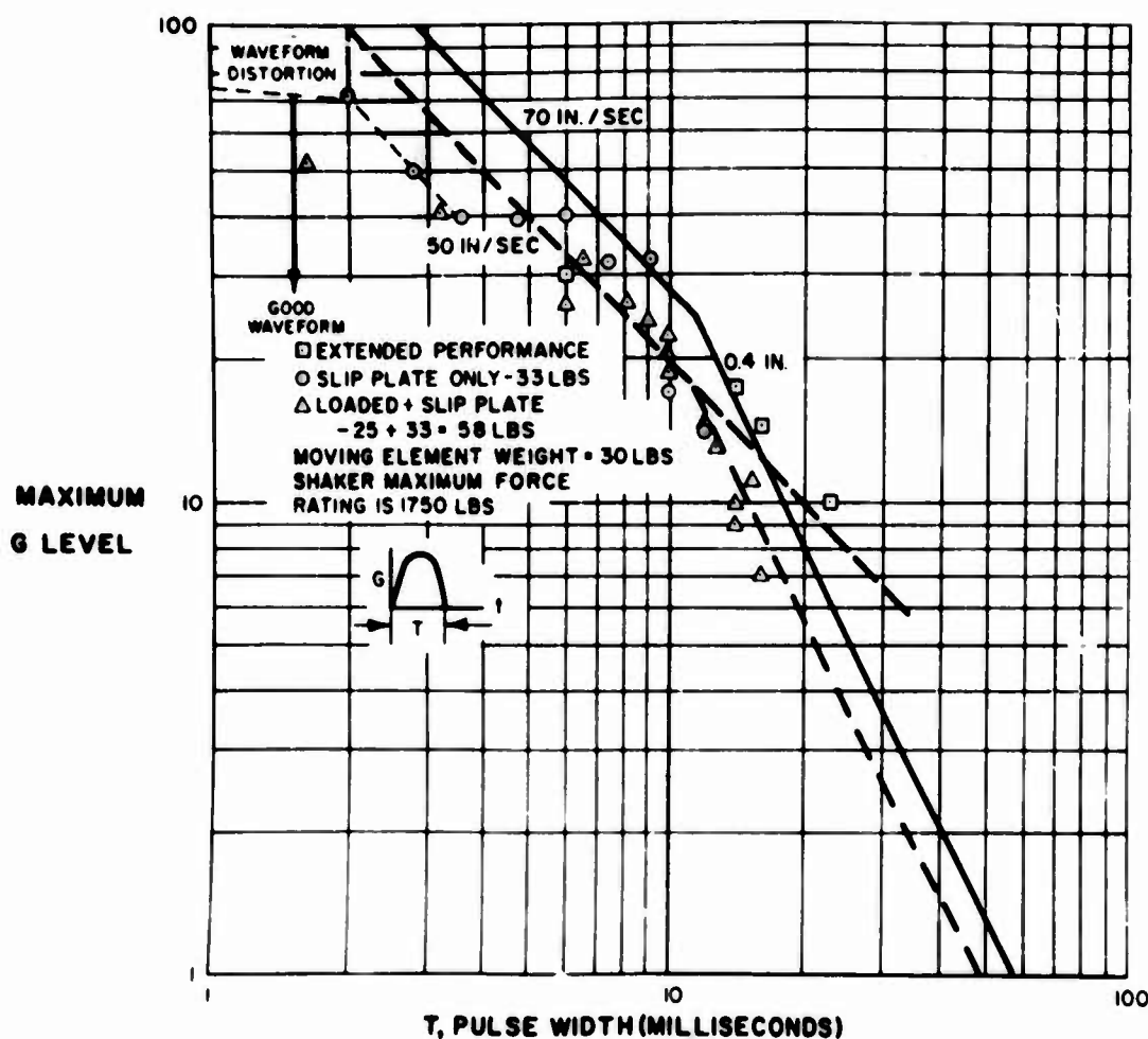
Fig. 3. Half-sine shock on M.B. C10VB
