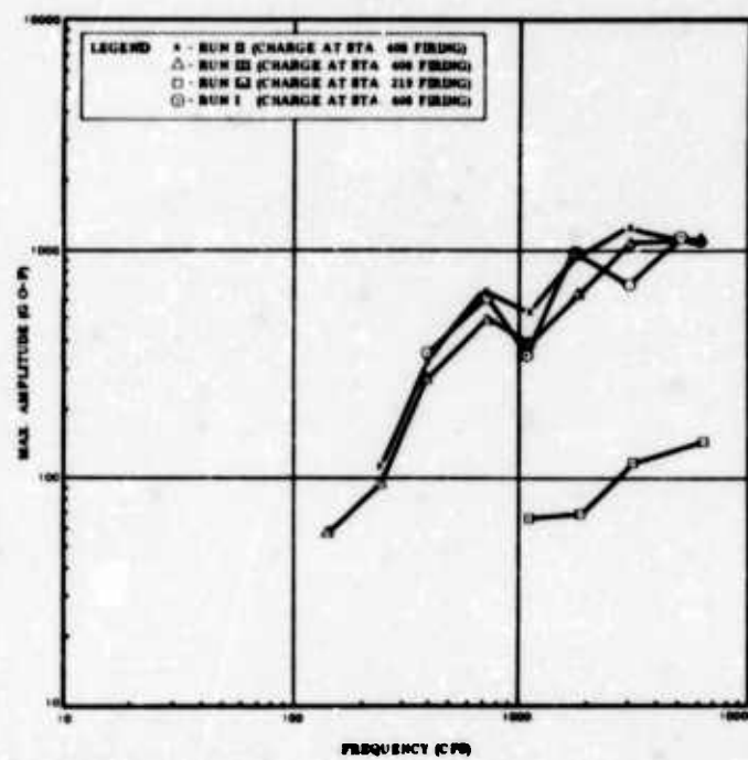
SHOCK RESPONSE SPECTRUM OF MEAS. NO. 8 (PROPELLANT UTILIZATION ELECTRONICS PACKAGE ACCEL. NORMAL TO BHD AT STA 437)
