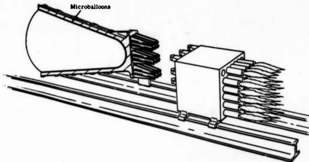
Fig. 3. Cutaway showing microballoons
