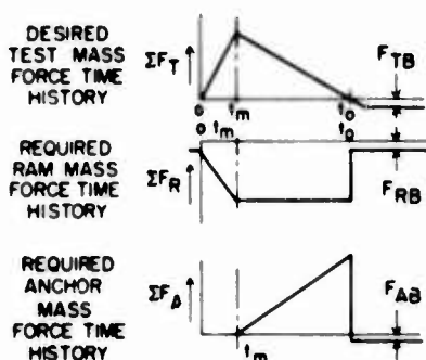
Fig. 7. Ideal force time histories on each mass during impact
