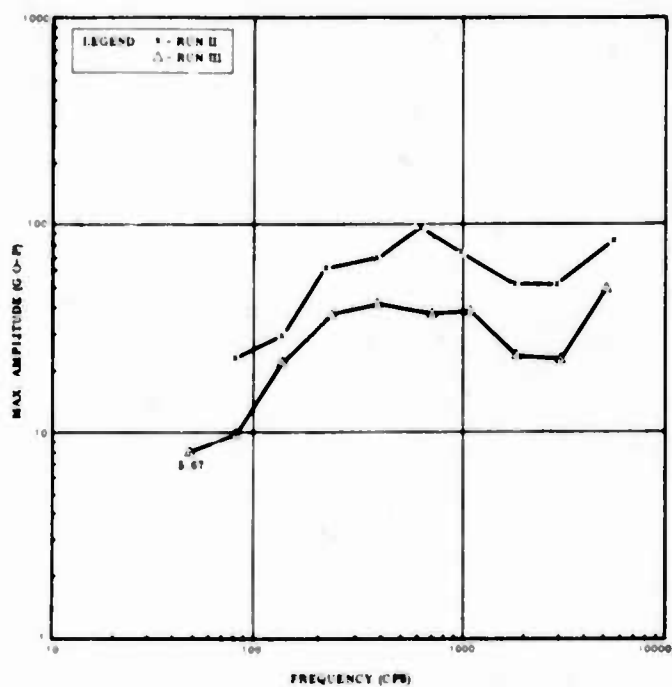
SHOCK RESPONSE SPECTRUM OF MEAS. NO. 12 (POWER CHANGEOVER SWITCH RADIAL STA 104)
