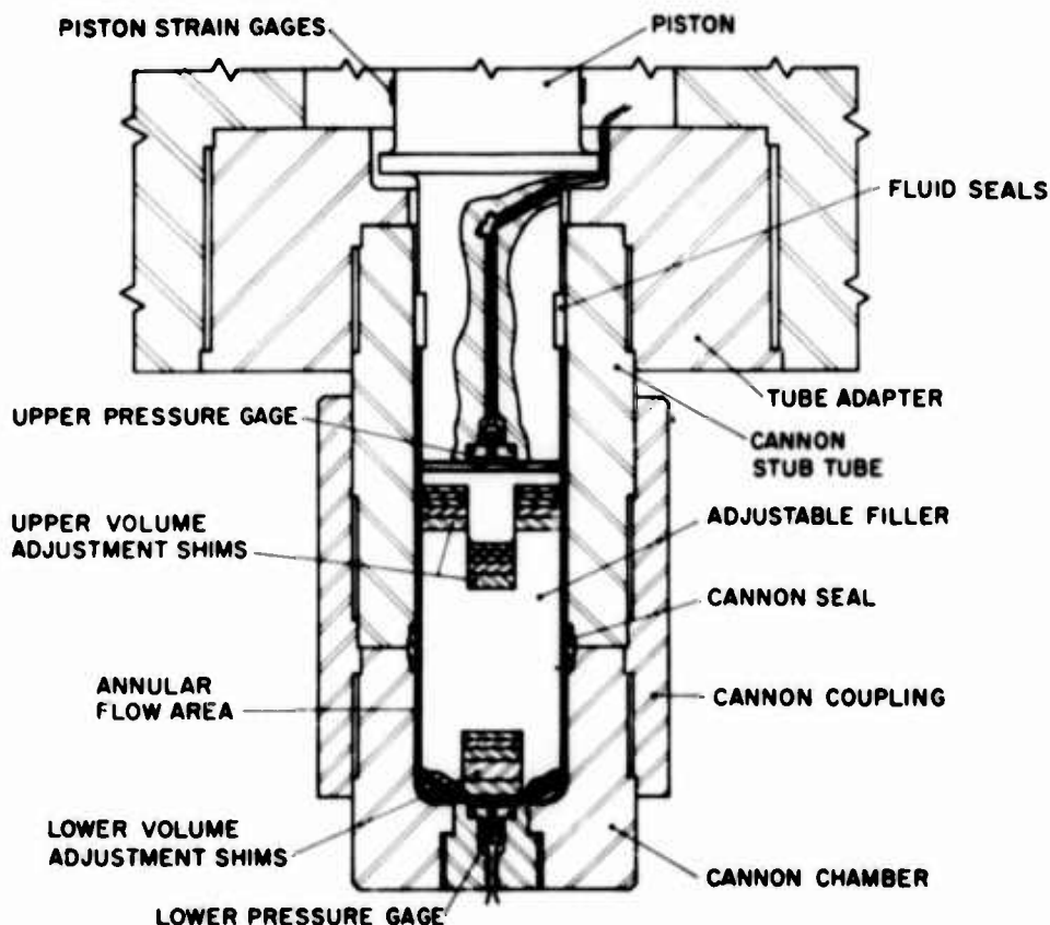
Fig. 4. Experimental apparatus for pressure-volume-flow study
