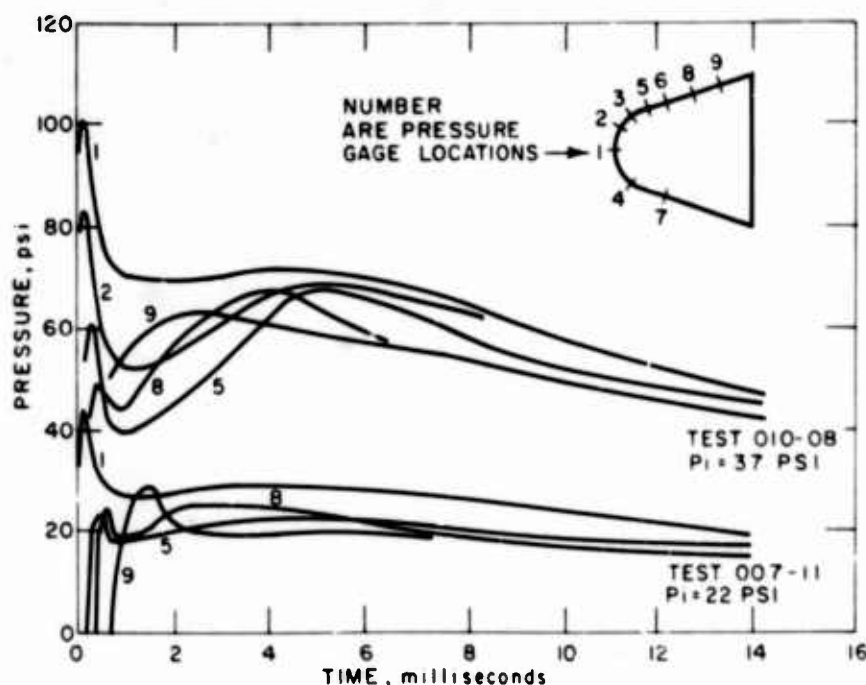
Fig. 4. Smoothed pressure-time functions for specific calibration tests
