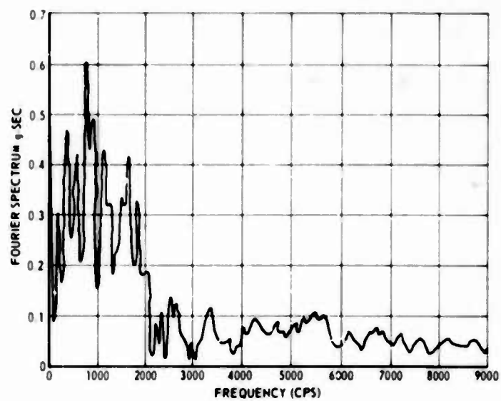
Fig. 15. Fourier amplitude spectrum-- test 1, accelerometer 8, relay panel
