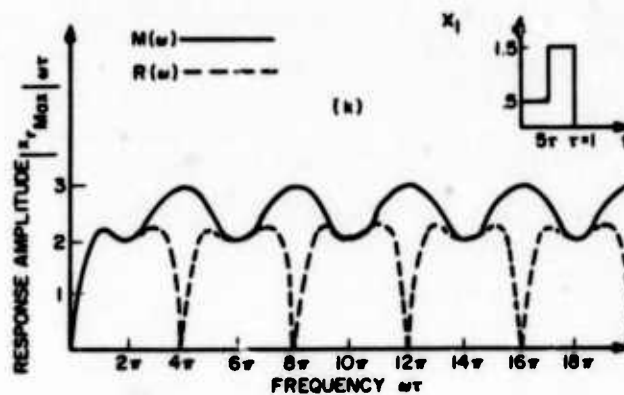
Fig. B-1. (Continued) Shock spectra for step-type pulses
