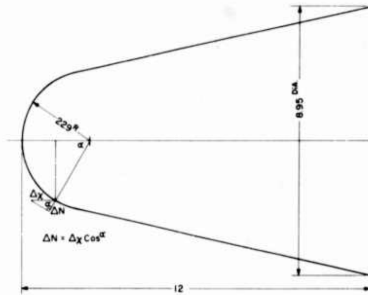
Fig. 7. Drawing of 1/10-scale model
