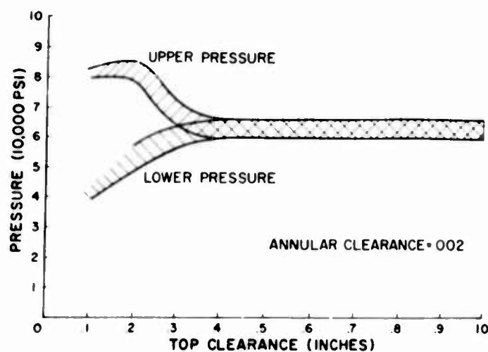
Fig. 10. Variation of peak pressures with top clearance
