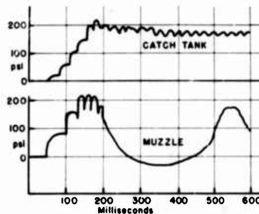
Fig. 20. Muzzle check valve performance chart
