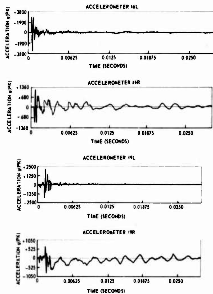
Fig. 8. Shaped charge firing at Z-69 -- test 2
