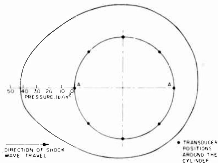
Fig. 2. Distribution of initial peak pressures
