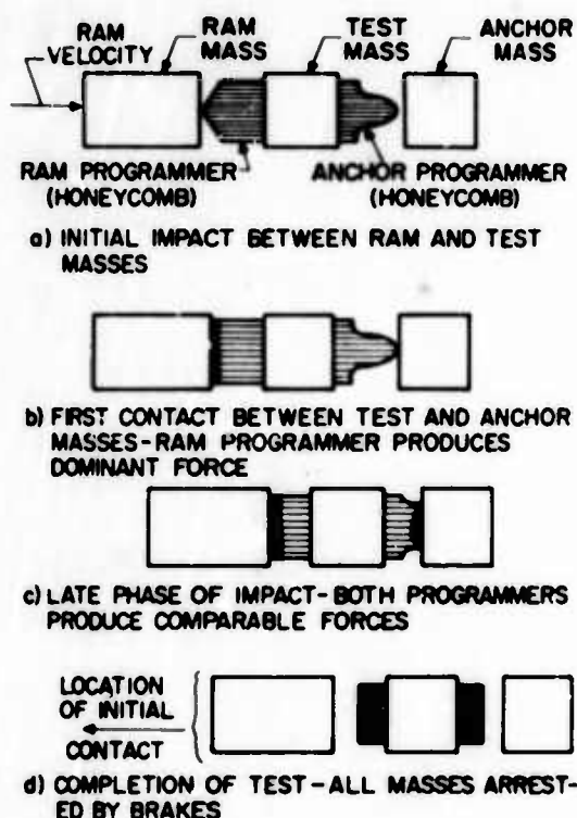
Fig. 1. Schematic of free impact test
