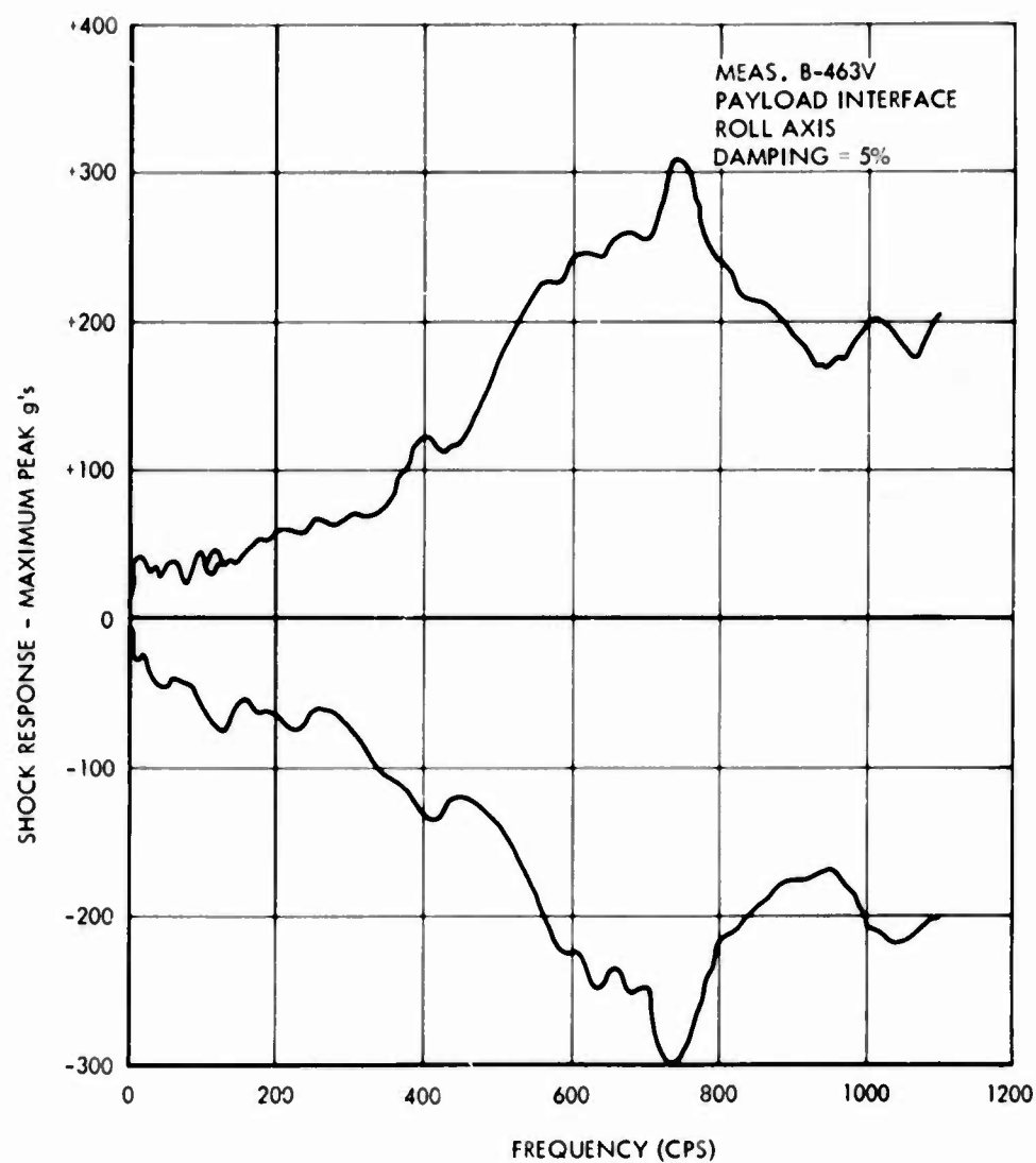
Fig. 8. Shock response spectrum, maximum envelope B-463V
