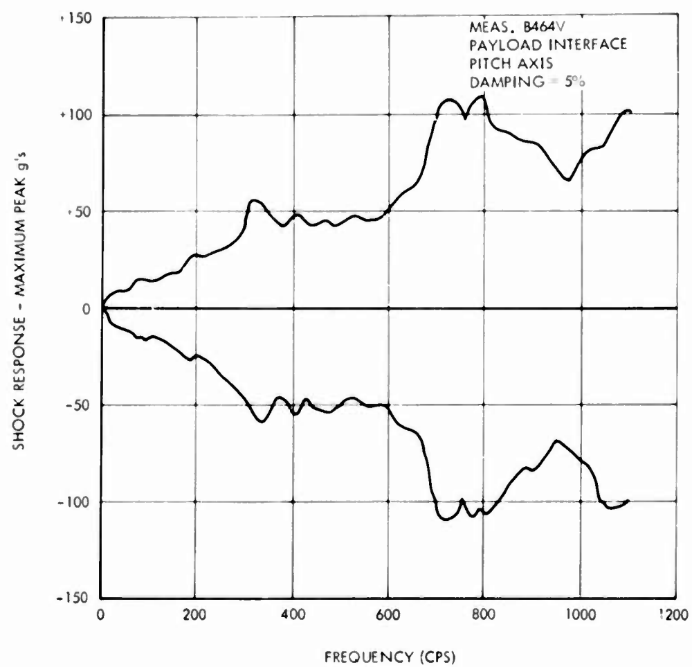
Fig. 9. Shock response spectrum, maximum envelope B-464V
