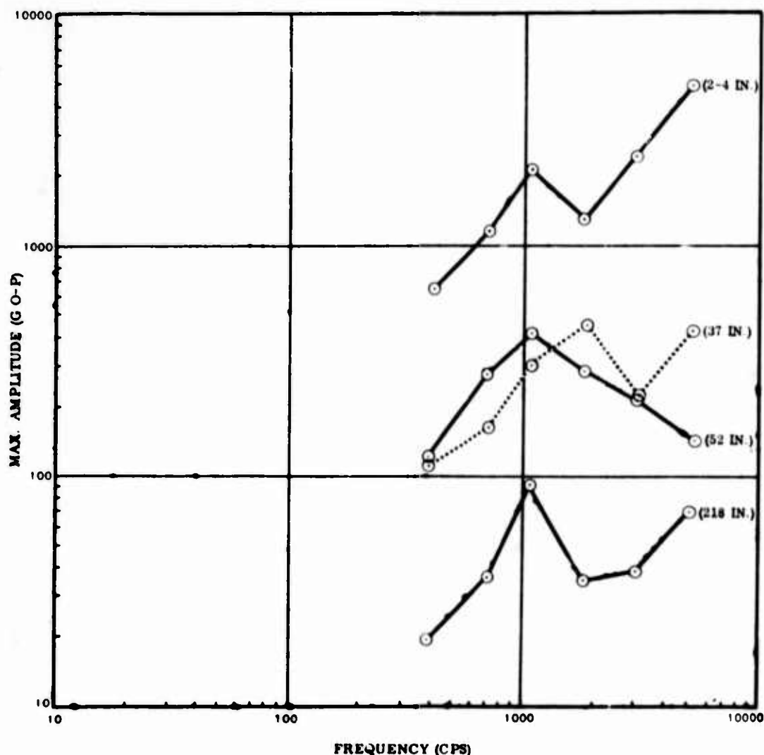
Fig. 19. Comparison of shock spectra and distance from shaped charge ( Q = 5 )
