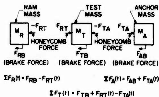
Fig. 6. Force diagrams used during analysis
