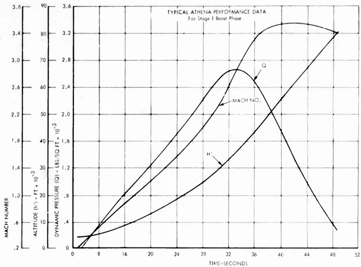
Fig. 4. ATHENA performance data
