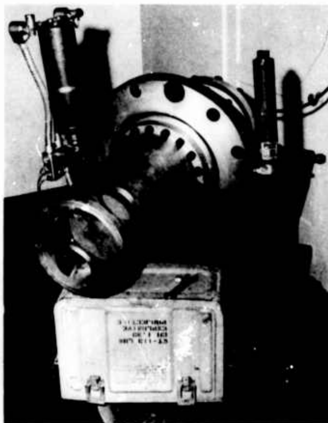
Fig. 17. Fast-opening valve removed, forward end
