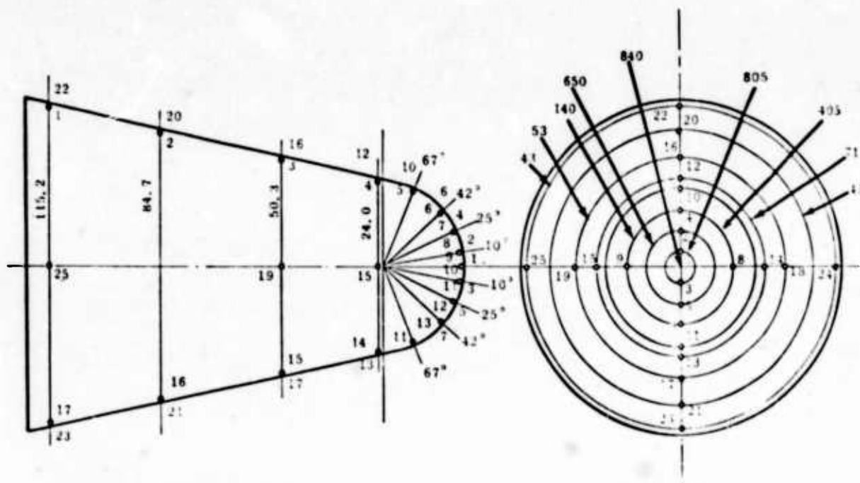
Fig. 15. Pressure transducer locations
