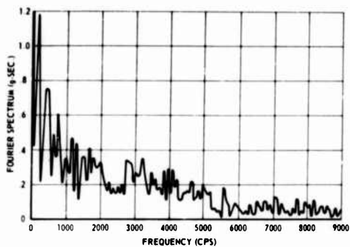
Fig. 19. Fourier amplitude spectrum-- test 2, accelerometer 6R
