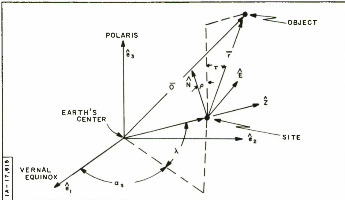
Figure 4. Site-Earth Geometry
