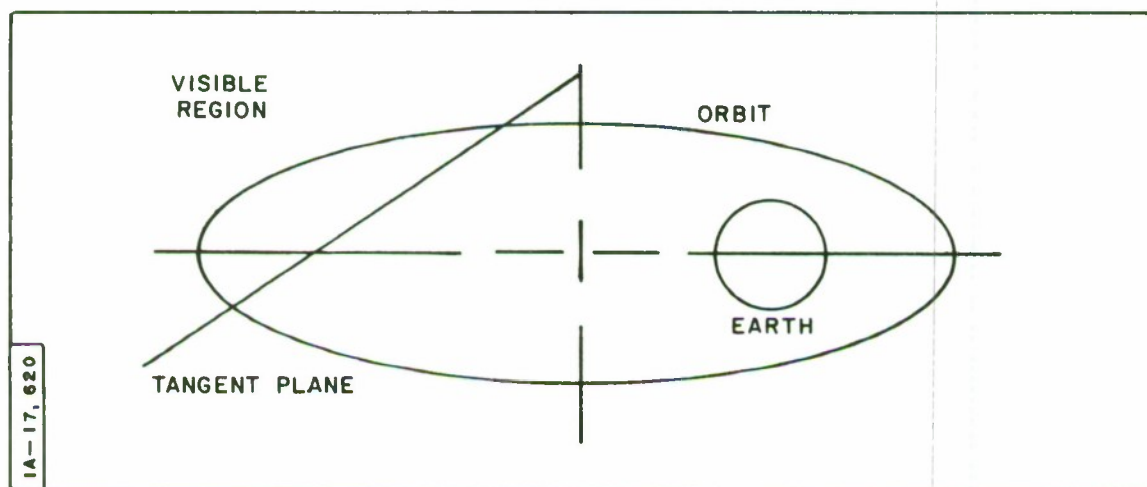
Figure 5. Region of Satellite Visibility
