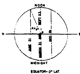
Figure 1. Diagram of the Earth's Equator.
