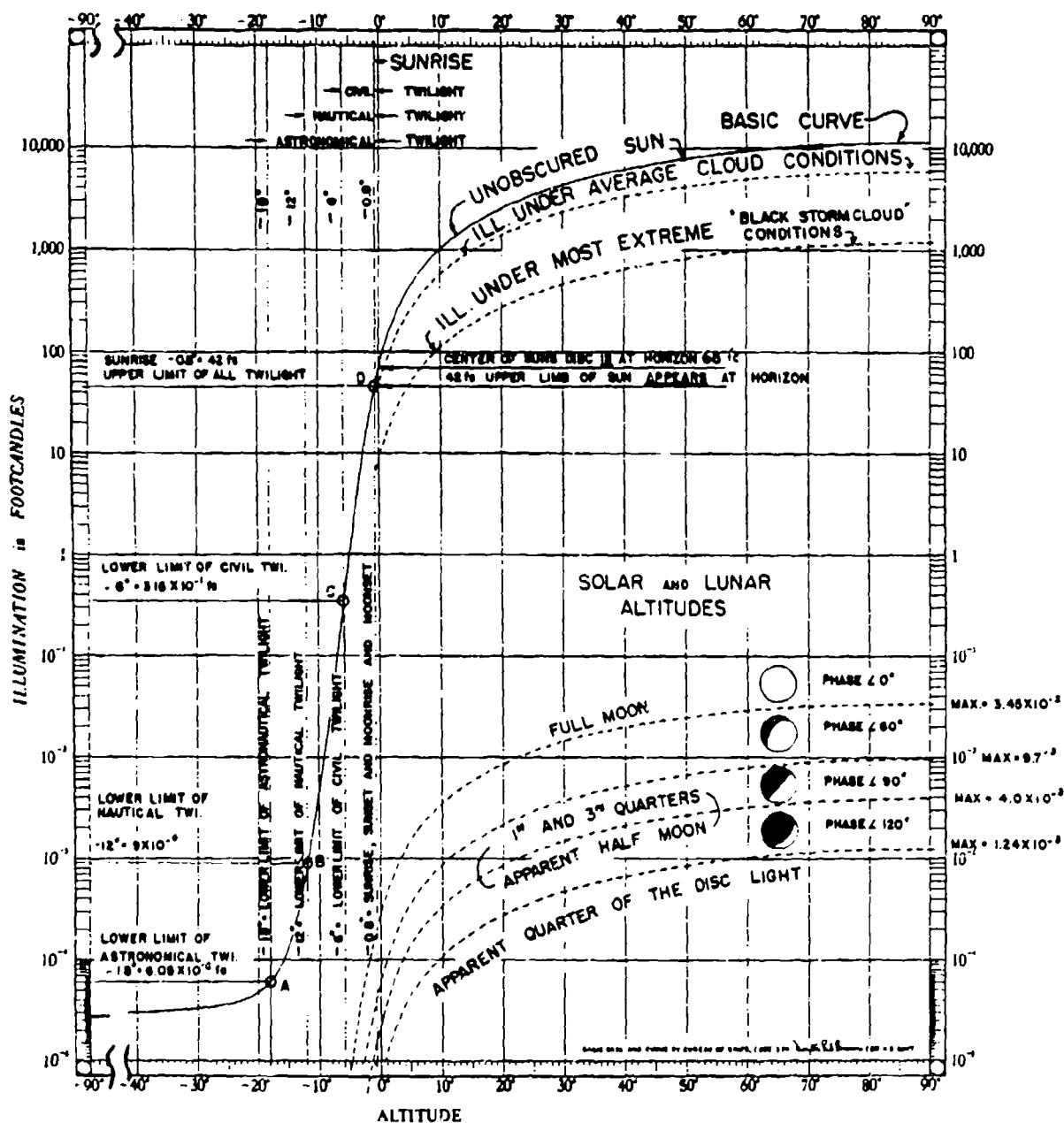
Figure 6. Time range of celestial illumination.
