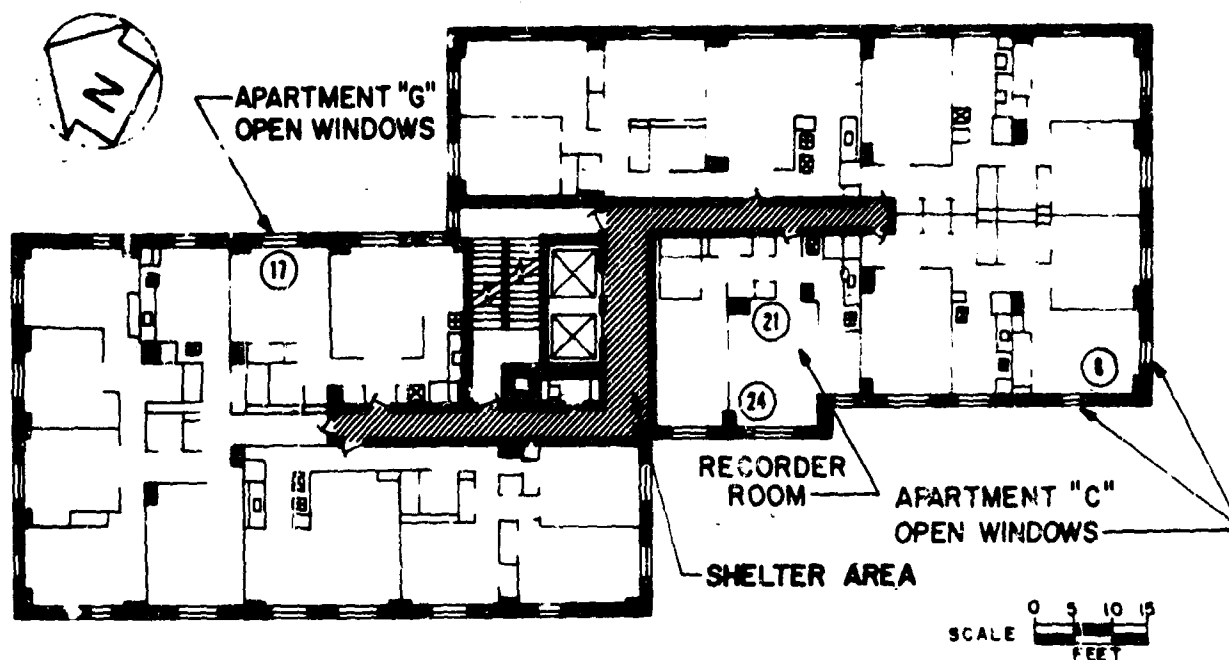
BUILDING #7 - 18 TH FLOOR PLAN
