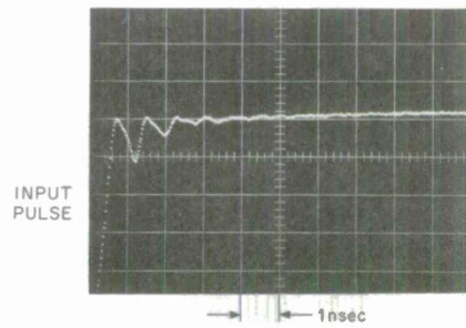
Fig. 16. Rise time of sample holder compared to rise time of input pulse.
