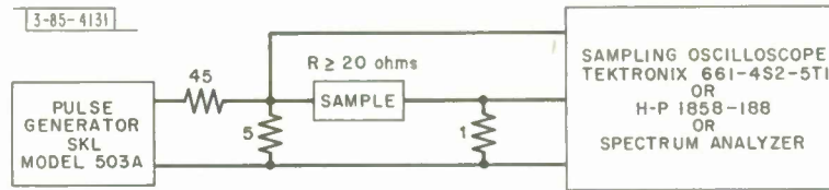
Fig. 12. Diagram of circuit used to measure sample current and voltage vs time.
