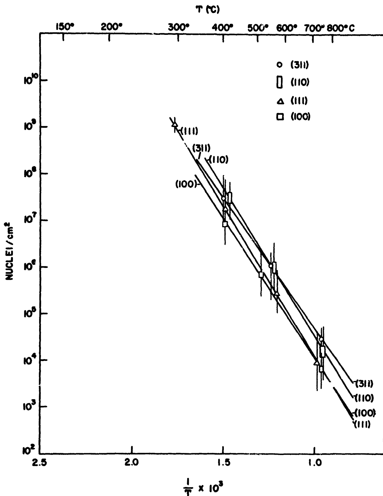
FIGURE 16 DENSITY OF NUCLEI PER SQUARE CENTIMETER AS A FUNCTION OF TEMPERATURE FOR VARIOUS CRYSTAL FACES AT 10^{-2} TORR.
