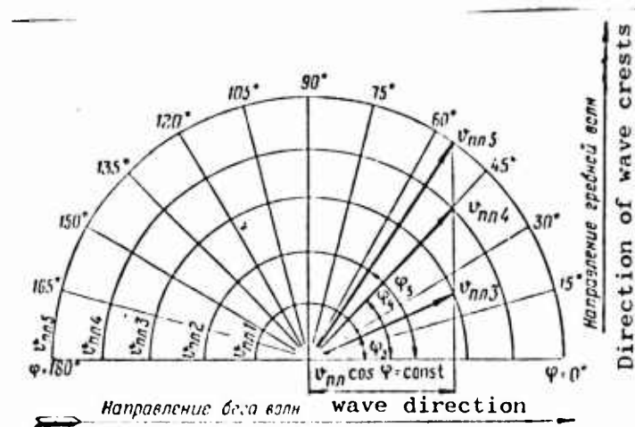
Figure 148. V. G. Vlasov roll diagram grid.
