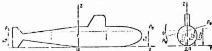
Figure 9. Submarine attitude: even keel, but with list.
