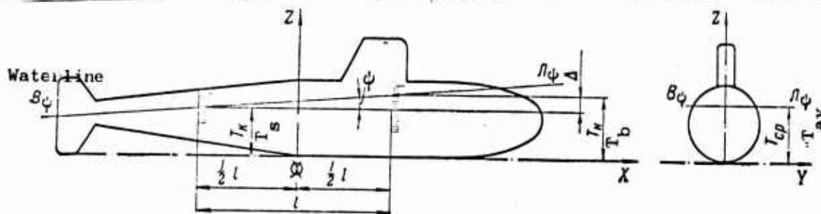
Figure 7. Submarine attitude: upright, but with trim on.
