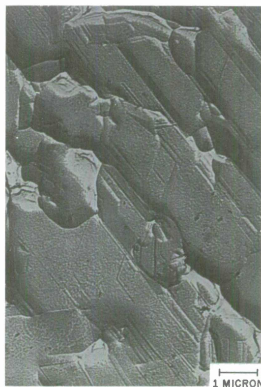
This electron micrograph of the surface of a silicon film grown epitaxially on sapphire has a magnification of 10,000 times. The ridge lines are the boundaries between adjacent silicon crystallites. The dislocation lines and triangles are visible in each crystallite. The silicon film is six microns thick, and it is oriented in the "111" direction.
