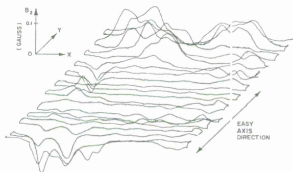
This illustration shows the uniformity of a 3 x 3 inch, thin magnetic film. The mountains and valleys are at the boundaries between differently magnetized areas, which occur when the film is in a partially switched state. The apparent third dimension corresponds to a vertical component of magnetic field.
