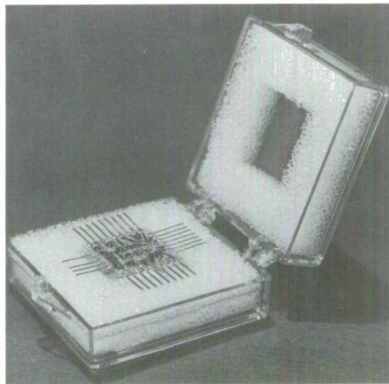
On the 0.5 by 0.5 inch glass substrate are ten vacuum-deposited nichrome resistors, gold conductor lands, ten chip transistors, and four chip diodes. The OR-gate high-speed logic circuit is given complete electrical tests in this form before being encapsulated in epoxy.
