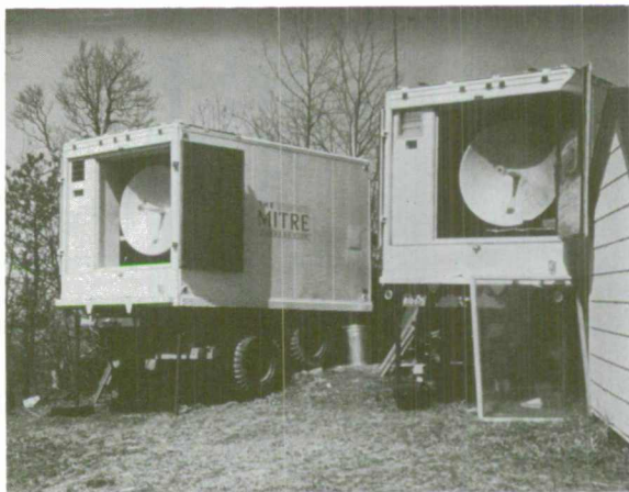
Line integral refractometer receivers aligned for reception of simultaneous, dual-frequency transmission at 15.6 Gc and 31.2 Gc. Each receiver measures the differential phase shift between the signals that are introduced along the path by the water vapor absorption at 22 Gc.
