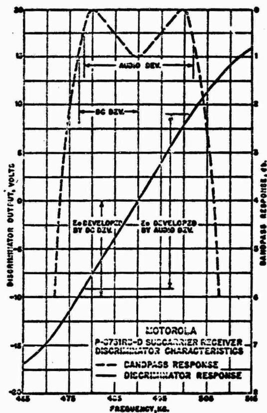
FIGURE 5 DISCRIMINATOR CHARACTERISTICS
