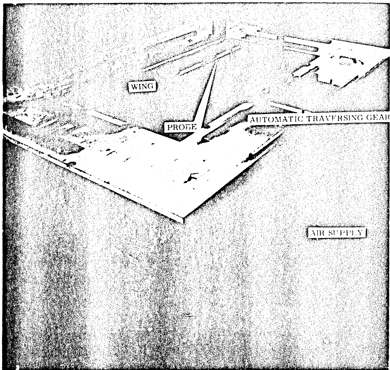
FIG.1 WING MOUNTED IN CALIBRATION RIG
