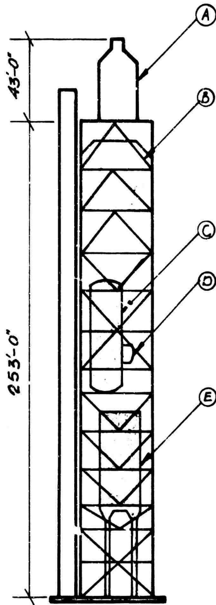
TCC SOUTH ELEVATION 1"=50'-0"
