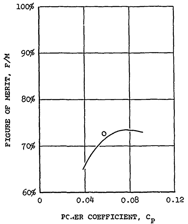
Figure 17. Figure of Merit Comparison.
