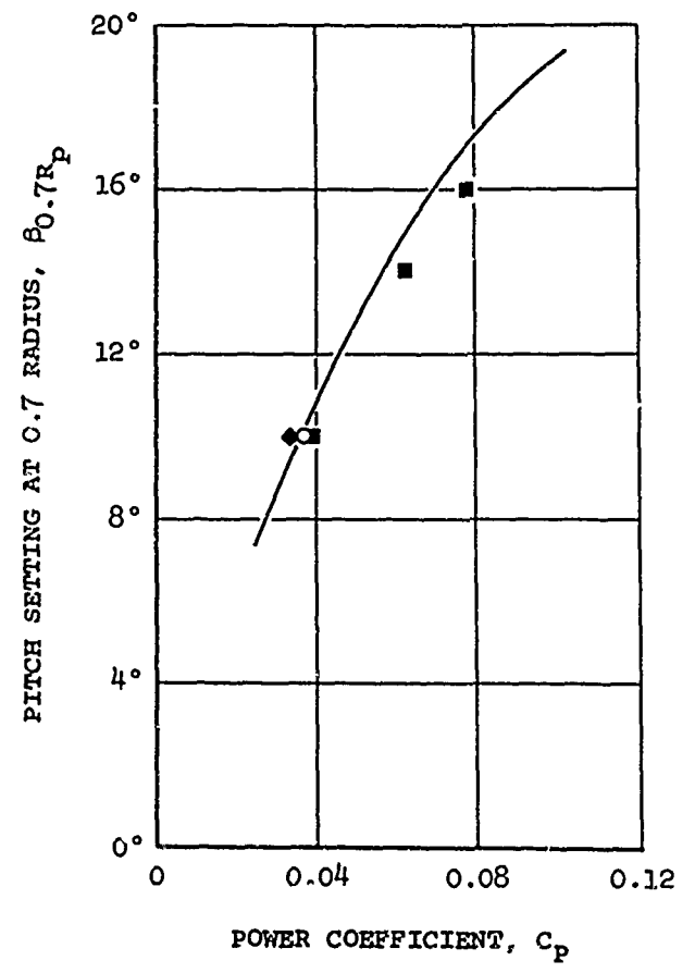
Figure 13. Pitch Setting Comparison.
