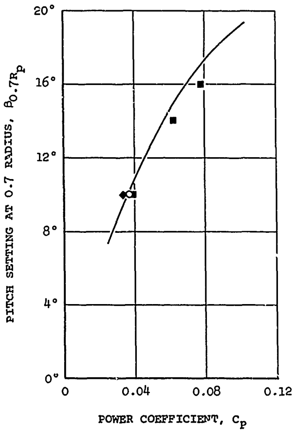
Figure 13. Pitch Setting Comparison.
