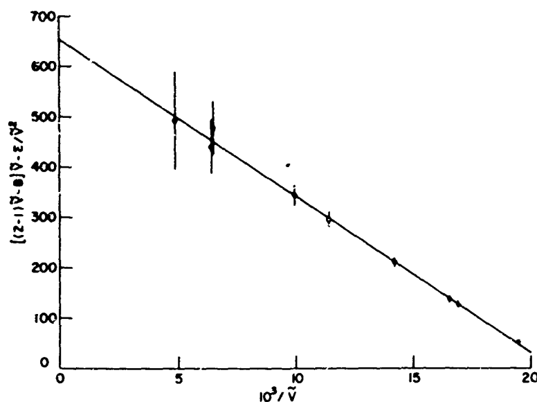
Fig. 7 - Plot of \{[(z - 1)\tilde{P} - B]\tilde{P} - E/\tilde{V}^2\} versus 1/\tilde{V} for cesium at 2400°F (vertical line for each point represents probable error)
